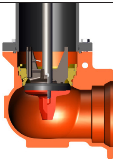
GUARDIAN 5-1/4" DRAIN VALVE
