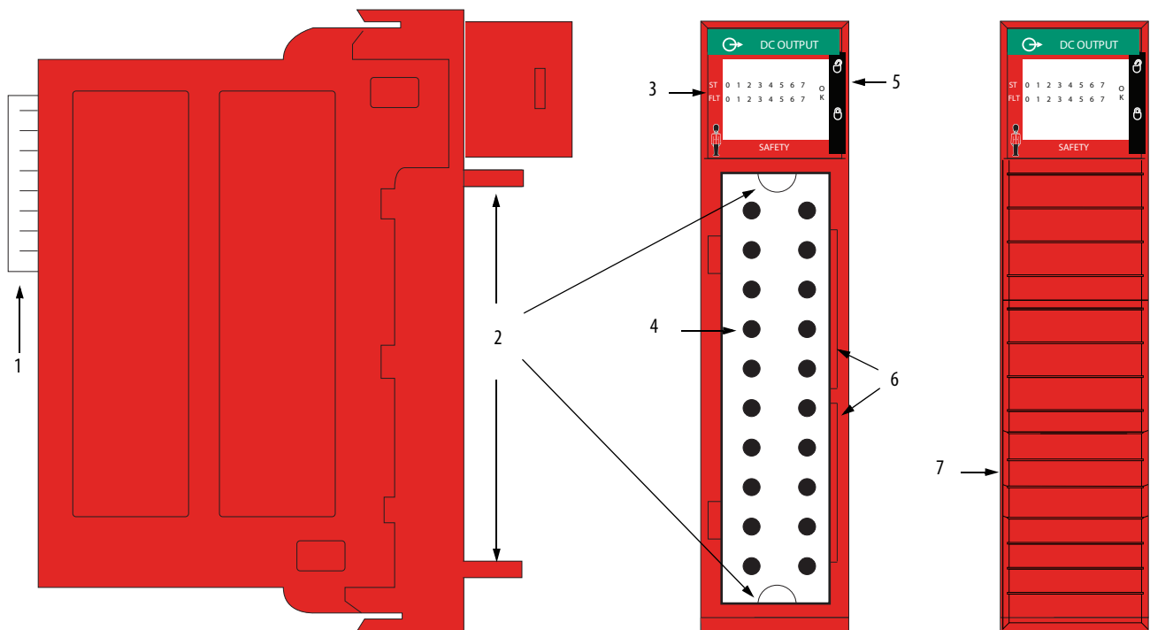
Figure 3 - Example 1756-0BV8S
