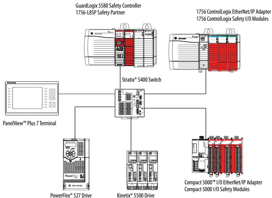
Figure 5 - Remote Safety I/O Modules in a GuardLogix 5580 Control Application
