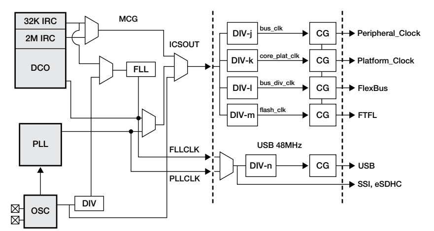
Clock Diagram
