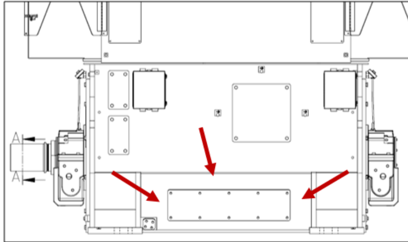
Figure 7.3 – Typical 680 (Types 1R.6), 800 (Types 1R.6), SH630 & SH710 Frame Space Heater Locations.
