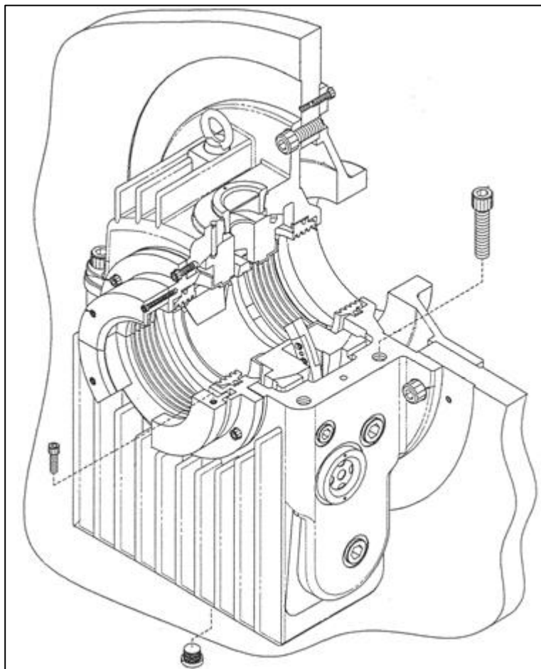
Figure 7.5 – Typical sleeve bearing construction for 680 (Types 1R.6), 800 (Types 1R.6), SH630 & SH710 Frames.
