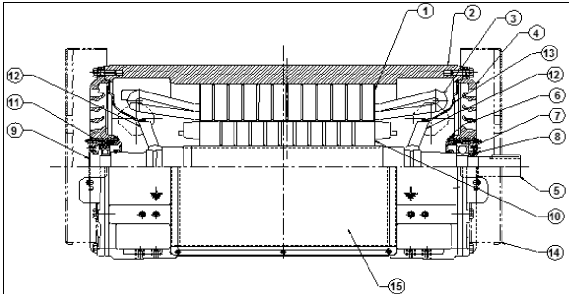
Typical aluminum die-cast rotor construction.
