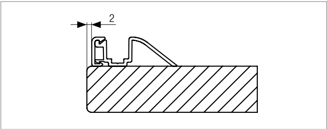
Fig. 4-13 Running track section on panel with recommended spacing
