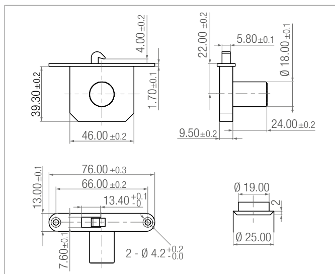
Fig. 4-43 Furniture mortise lock dimensions
