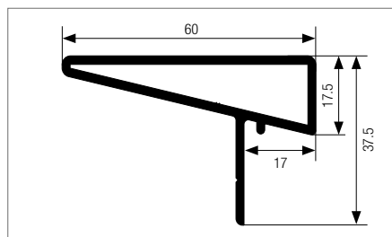
Vertical pelmet overlapping 60/17.5 mm
