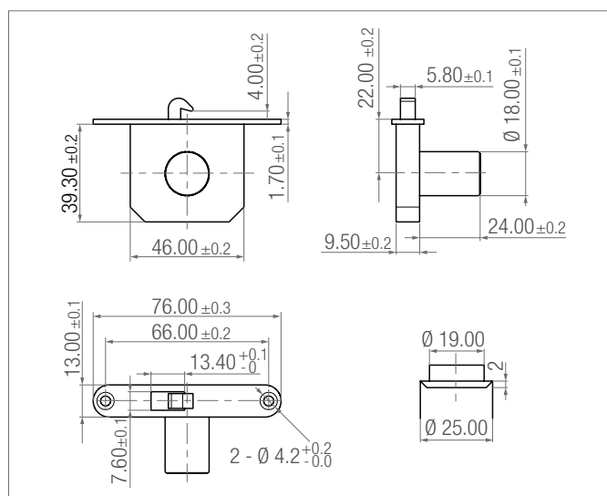
Fig. 4-26 Furniture mortise lock dimensions
