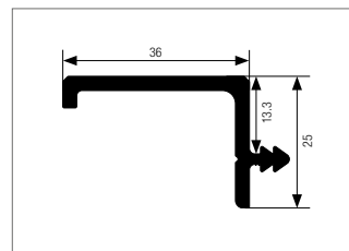
L-shaped vertical pelmet 36 mm with barb
