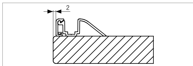
Fig. 4-35 Running track section on panel with recommended spacing
