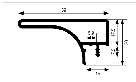
Vertical pelmet overlapping 59/17.5 m
