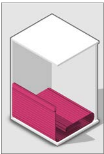
Fig. 4-32 Tambour door bottom running in spiral track
