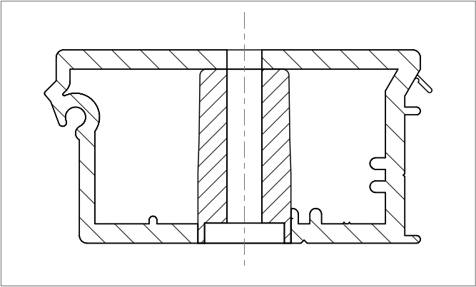
Fig. 4-39 Installation drawing
