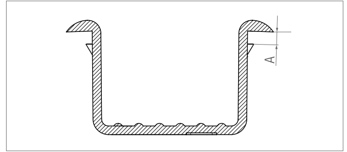
Fig. 4-41 Stop spacing A
