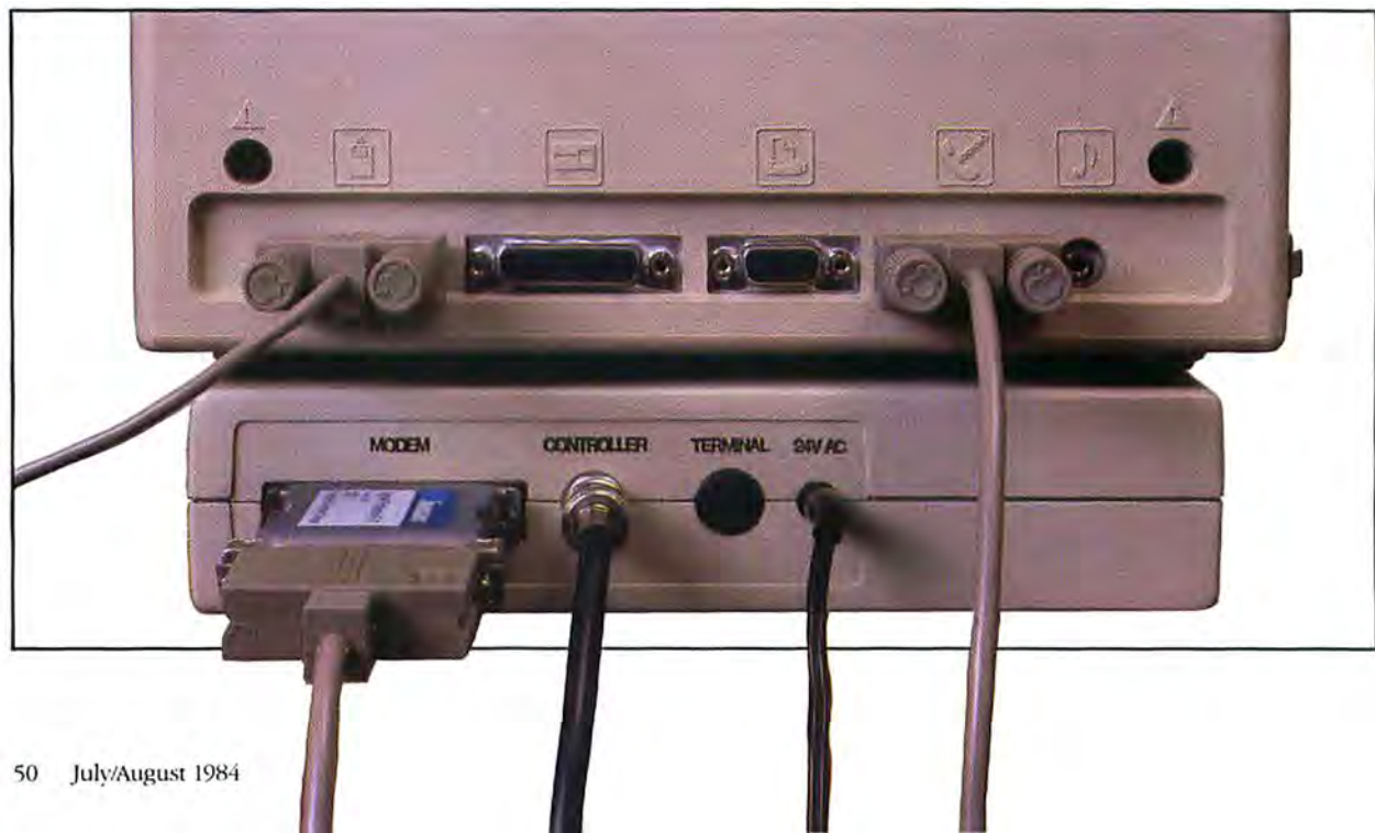
Figure 2 Using a gender changer, the serial cable connects to the modem port on the back of AppleLine and then to the Mac's telecommunications port. The coaxial cable extends from a 3274/6 communications controller and connects to the controller port. The rightmost port plugs AppleLine into a power source via an AC power adapter.
