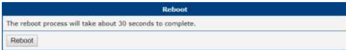
Figure 93: Reboot
