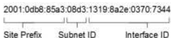
Figure 13: IPv6 Address with Prefix Example
