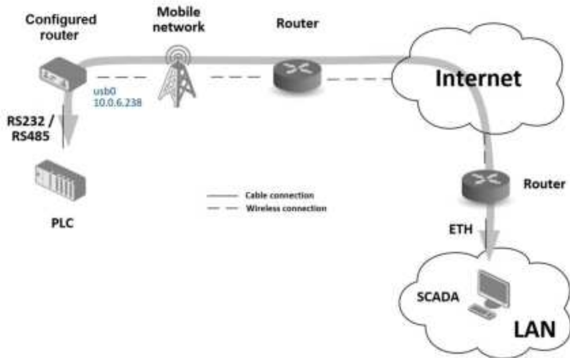
Figure 104: Serial Gateway – sample topology
