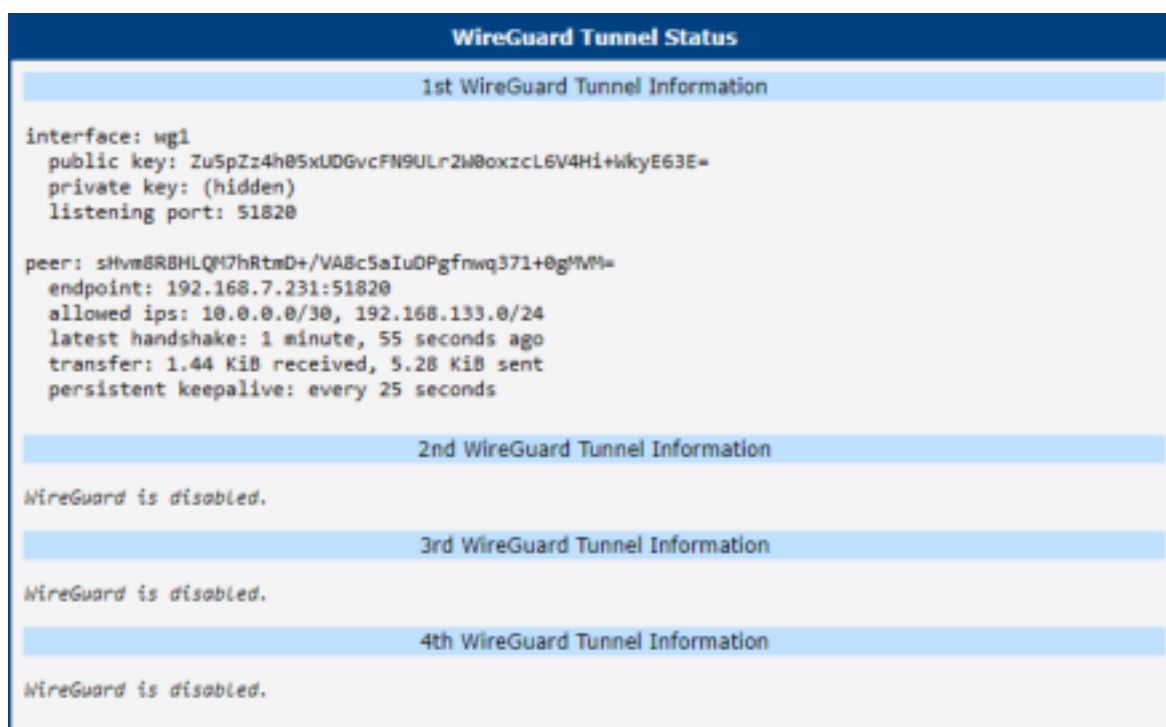
Figure 8: WireGuard Status Page
