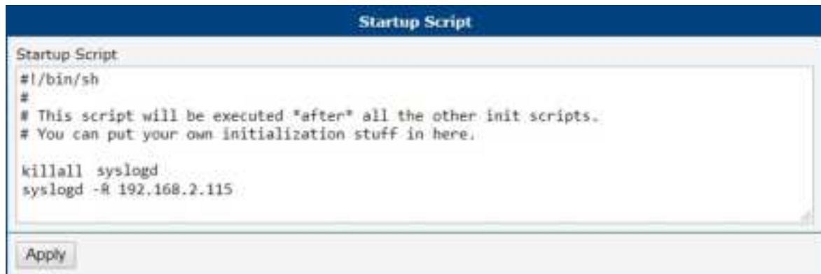
Figure 11: Example program syslogd start with the parameter -R
