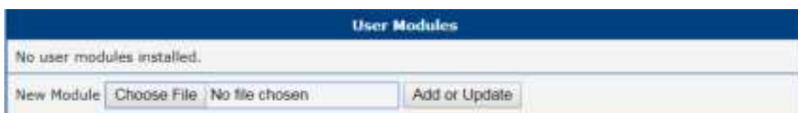
Figure 79: User modules
