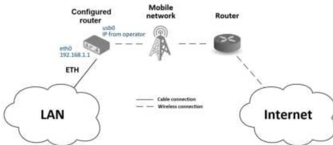
Figure 94: Access to the Internet from LAN – sample topology
