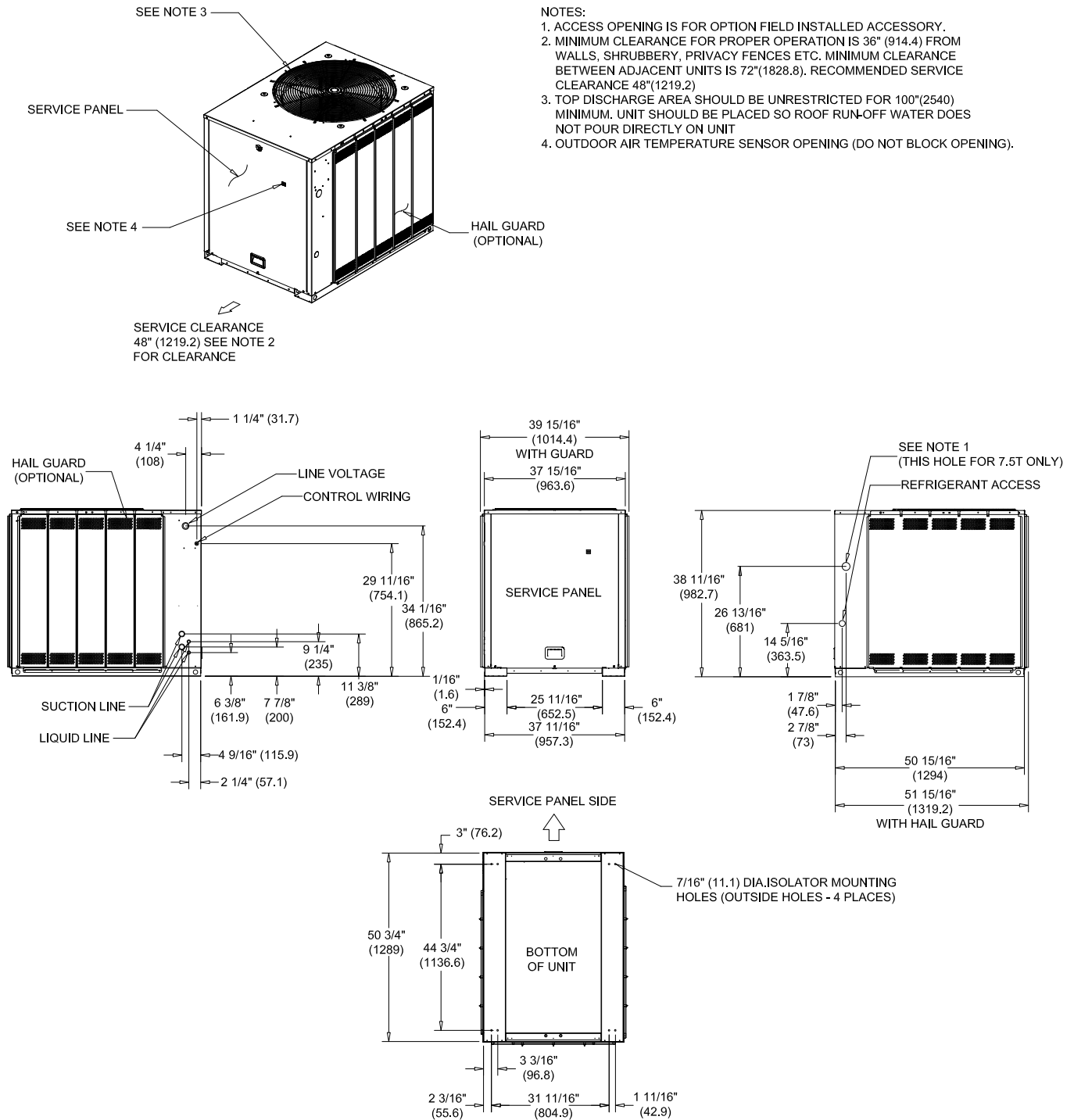
Figure 10. 5-6.25 ton heat pump, dual compressor
