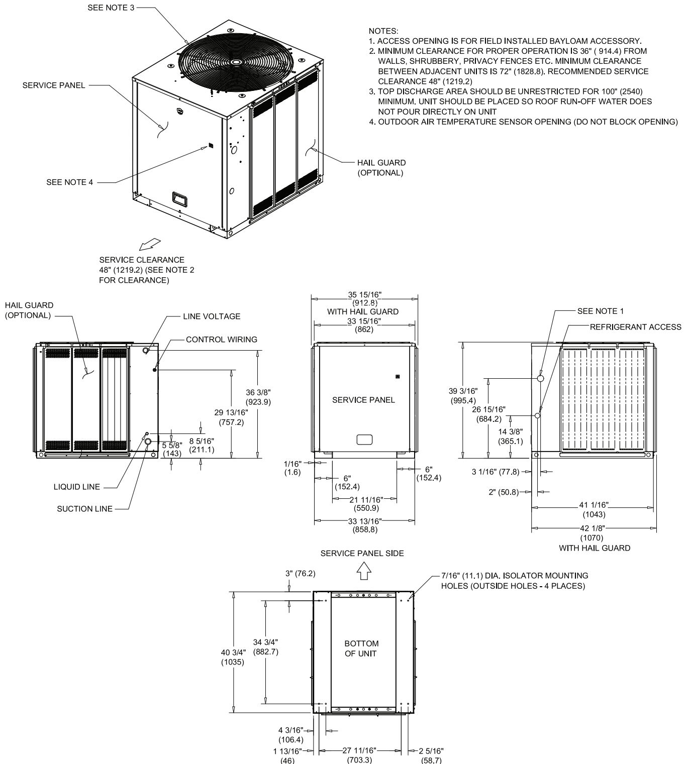
Figure 9. 5-6.25 ton heat pump, single compressor
