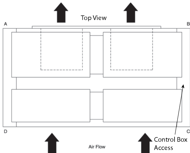
Figure 35. Horizontal — TWE126, 156, 201
