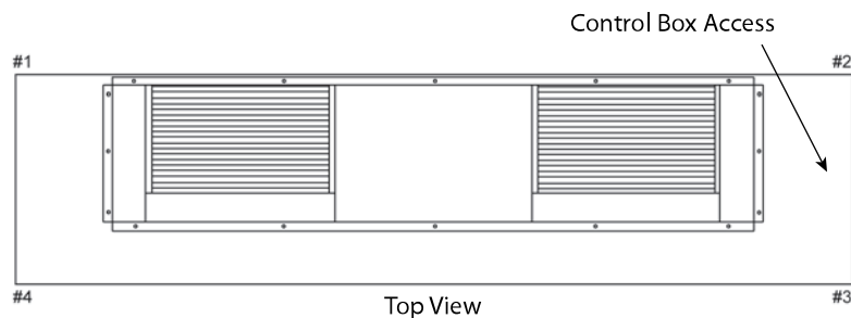
Figure 34. Horizontal — TWE051, 073, 076, 101
