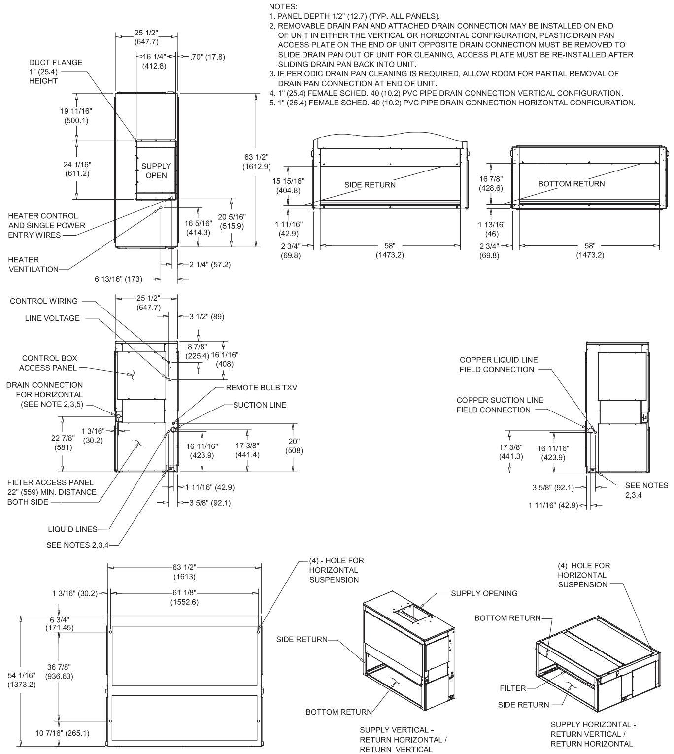
Figure 17. 8.33 ton air handler, single circuit
