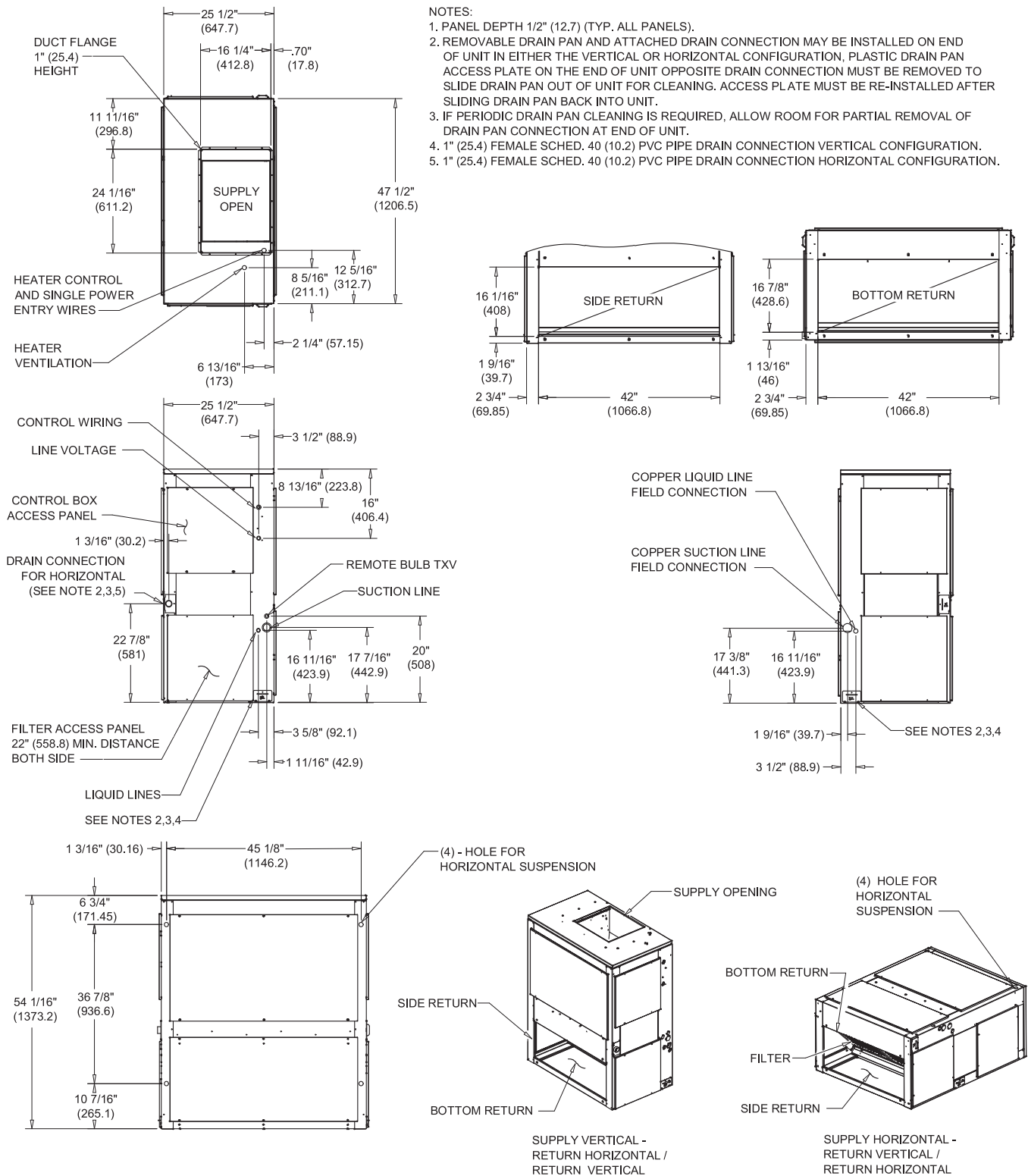
Figure 15. 6, 6.25 ton air handler, single circuit
