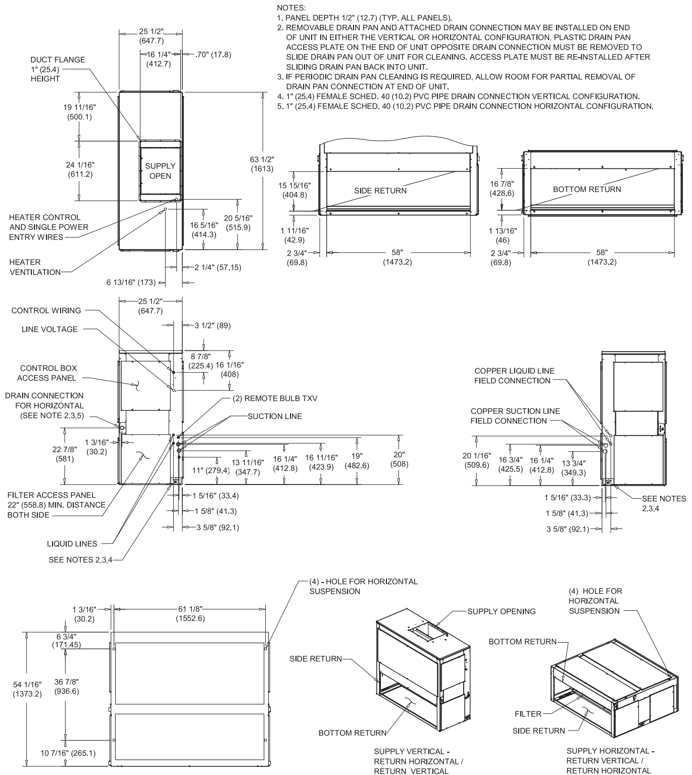
Figure 18. 8.33 ton air handler, dual circuit
