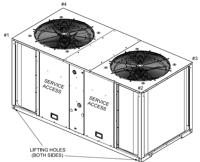
Figure 31. TWA156, 201
