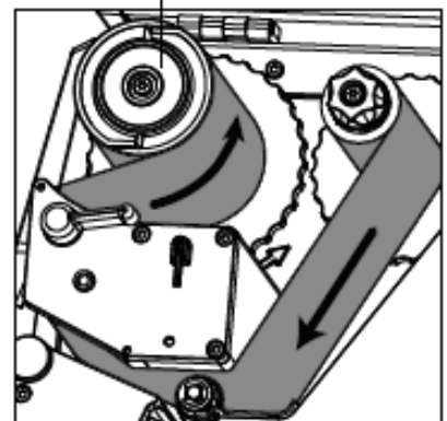
Ribbon Take-up Spindle
