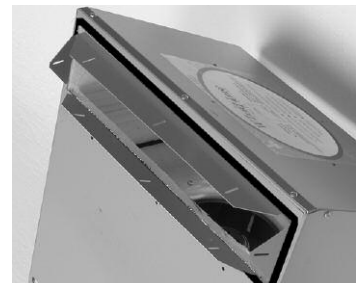
figure 2.2j- Bend tabs outward approximately 90 degrees.
