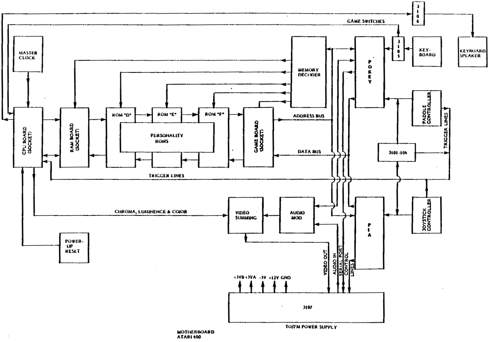
Figure 1-8. 400 Motherboard Flow Diagram
