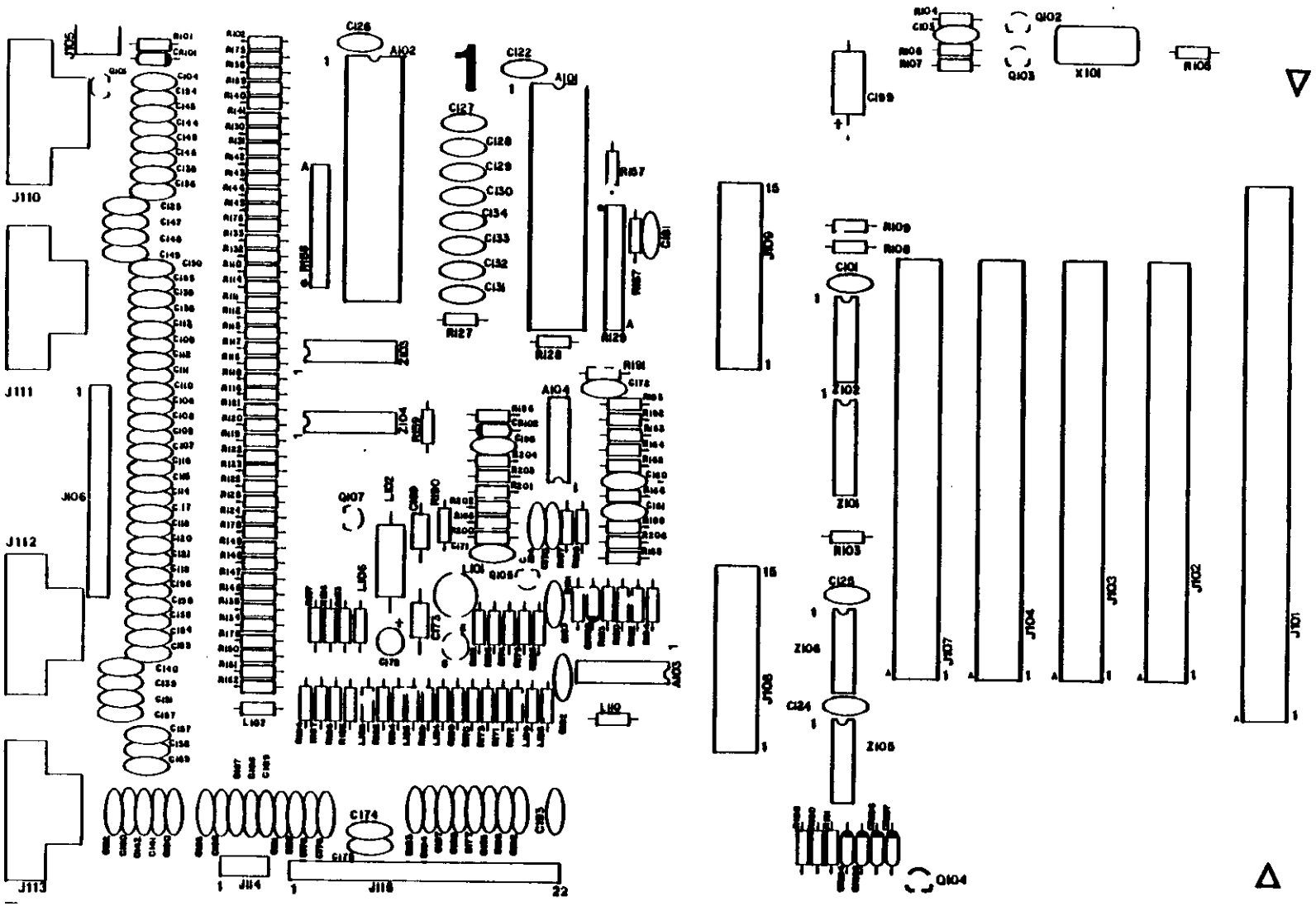
Figure 2-5. 800 Motherboard Silkscreen
