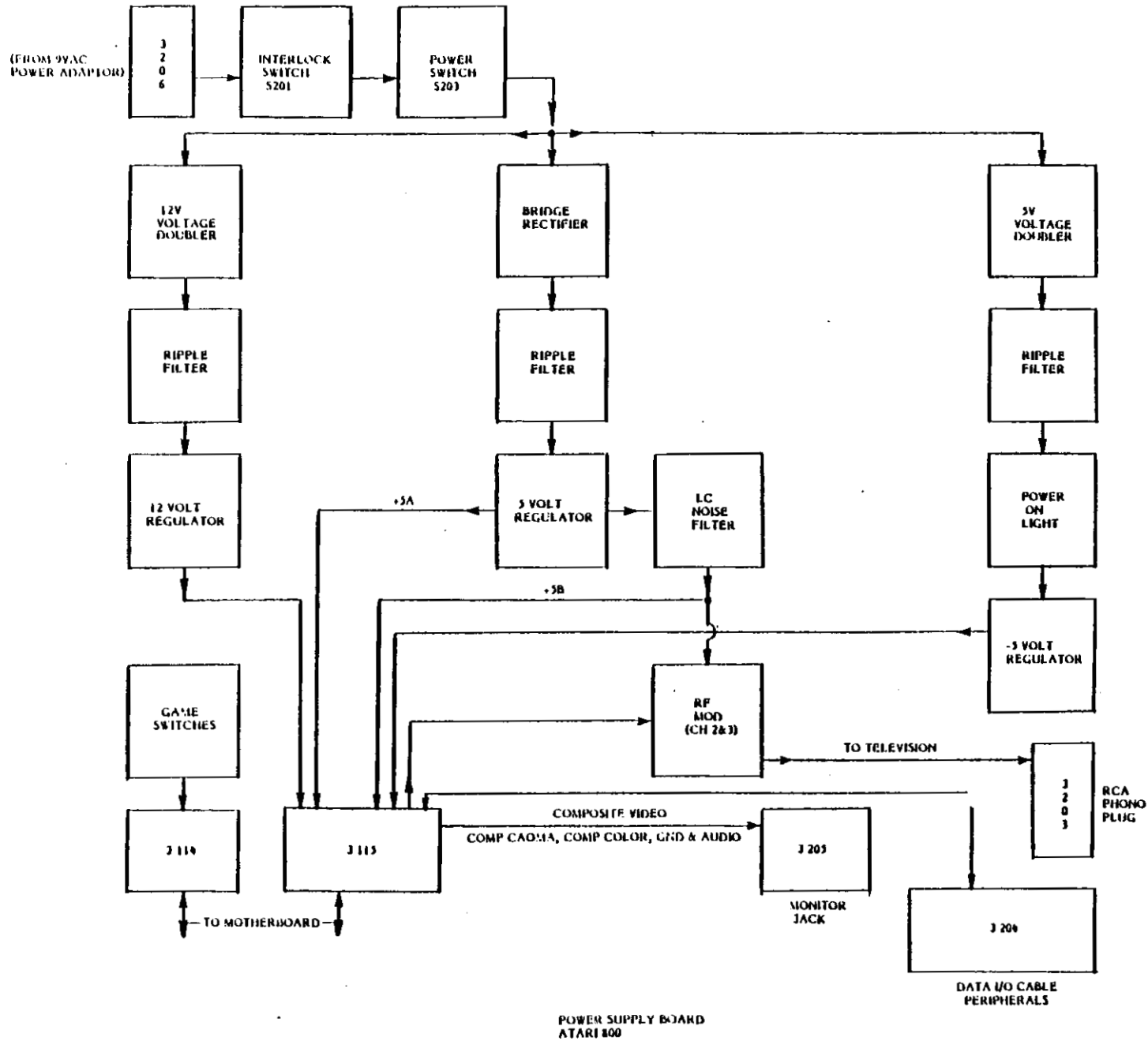
Figure 1-11. 800 Power Supply Flow Diagram
