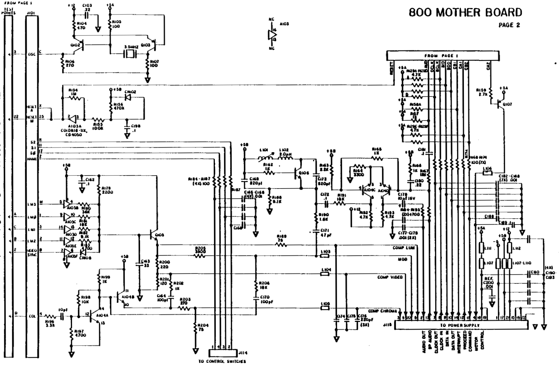
Figure 2-6. 800 Mother Board Schematic
