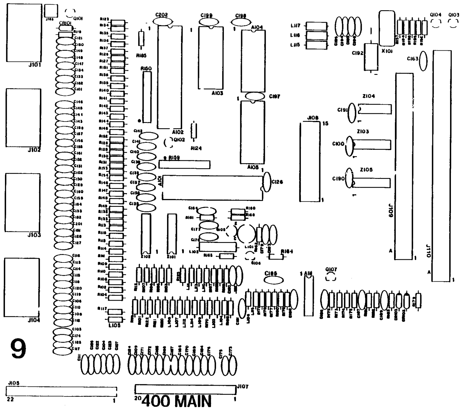
Figure 2-1. 400 Motherboard Silkscreen
