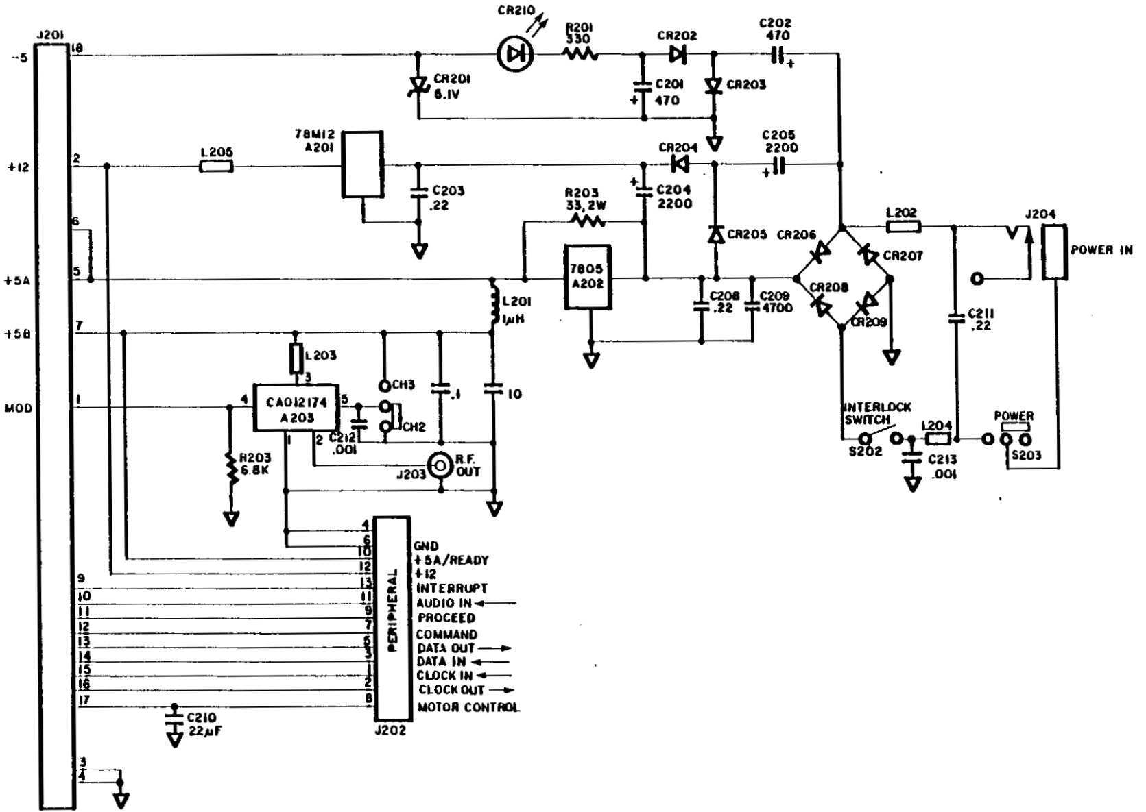
Figure 2-4. 400 Power Supply Schematic
