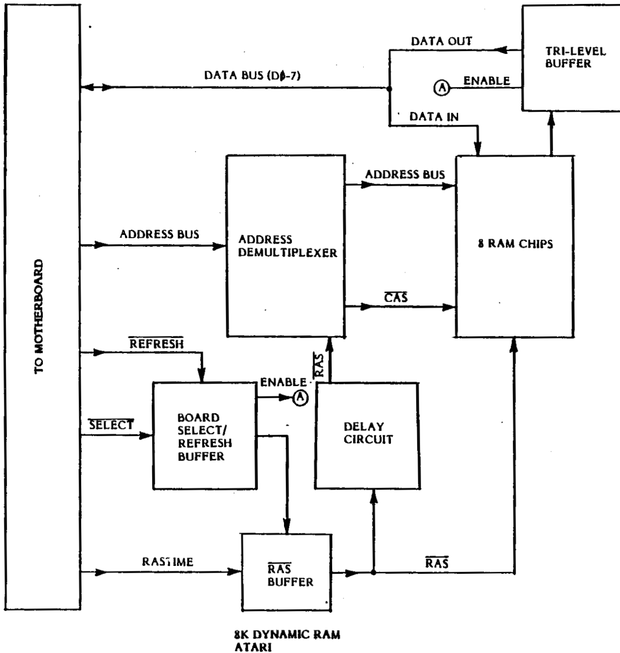
Figure 1-14. 8K Dynamic RAM Flow Diagram
