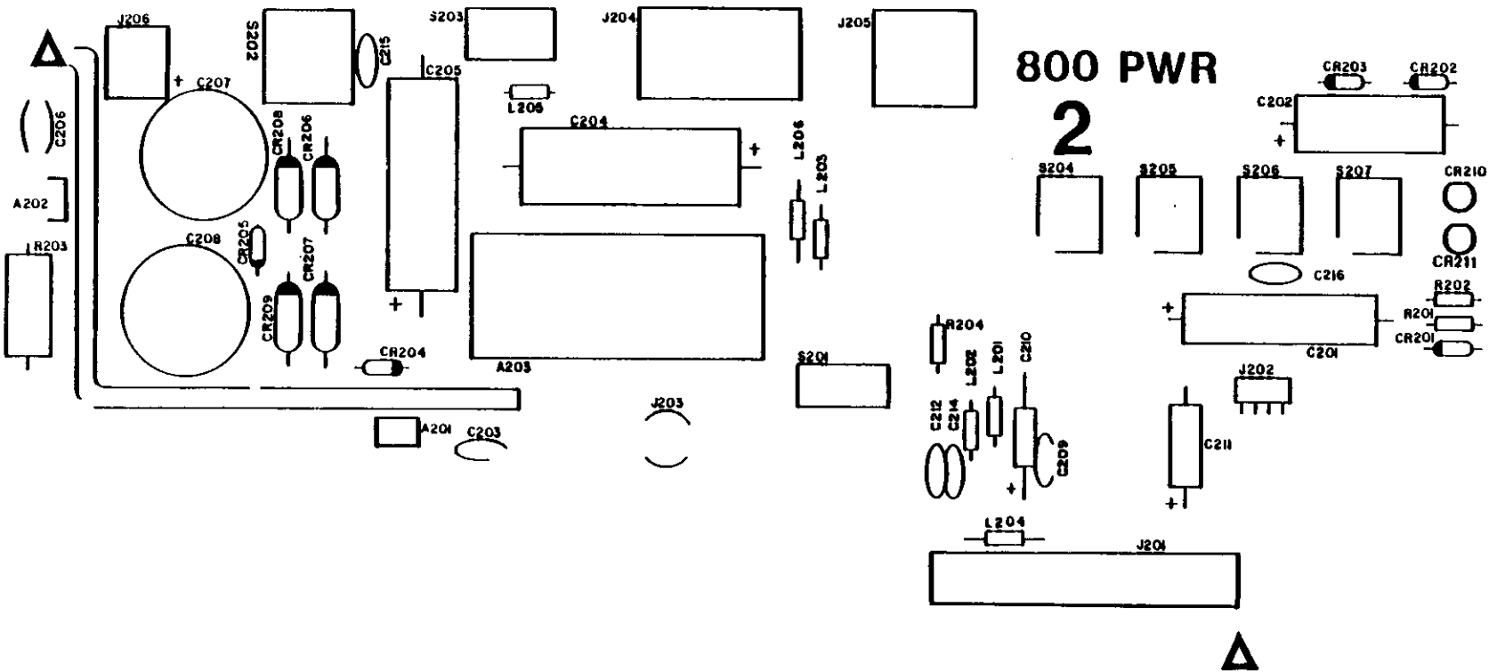
Figure 2-7. 800 Power Supply Silkscreen
