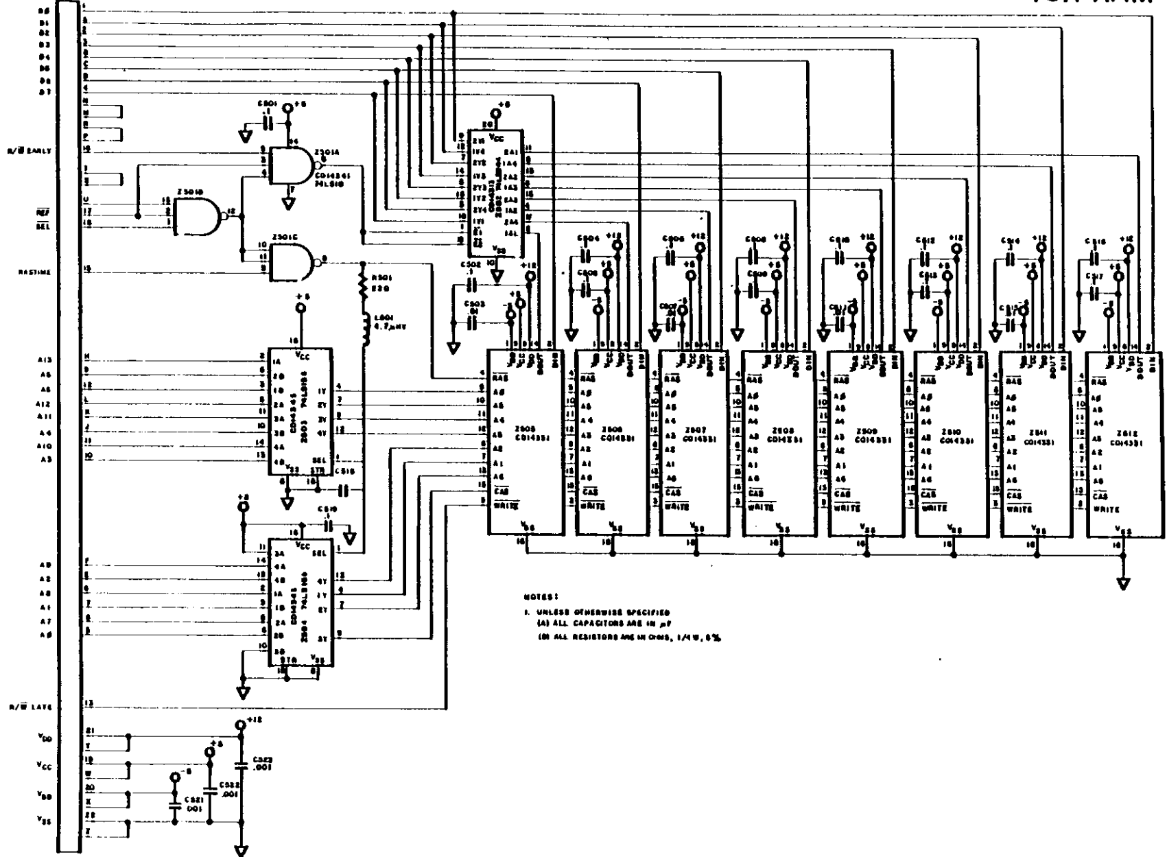
Figure 2-16. 16K RAM Board Schematic
