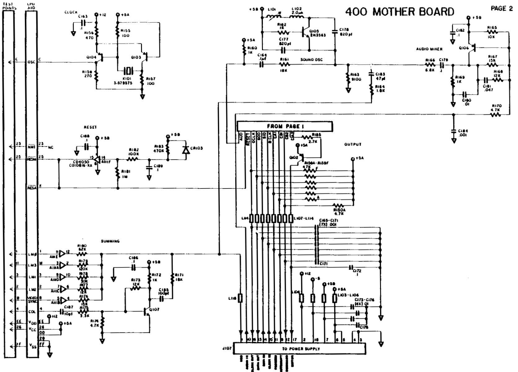
Figure 2-2. 400 Motherboard Schematic Page 2 of 2
