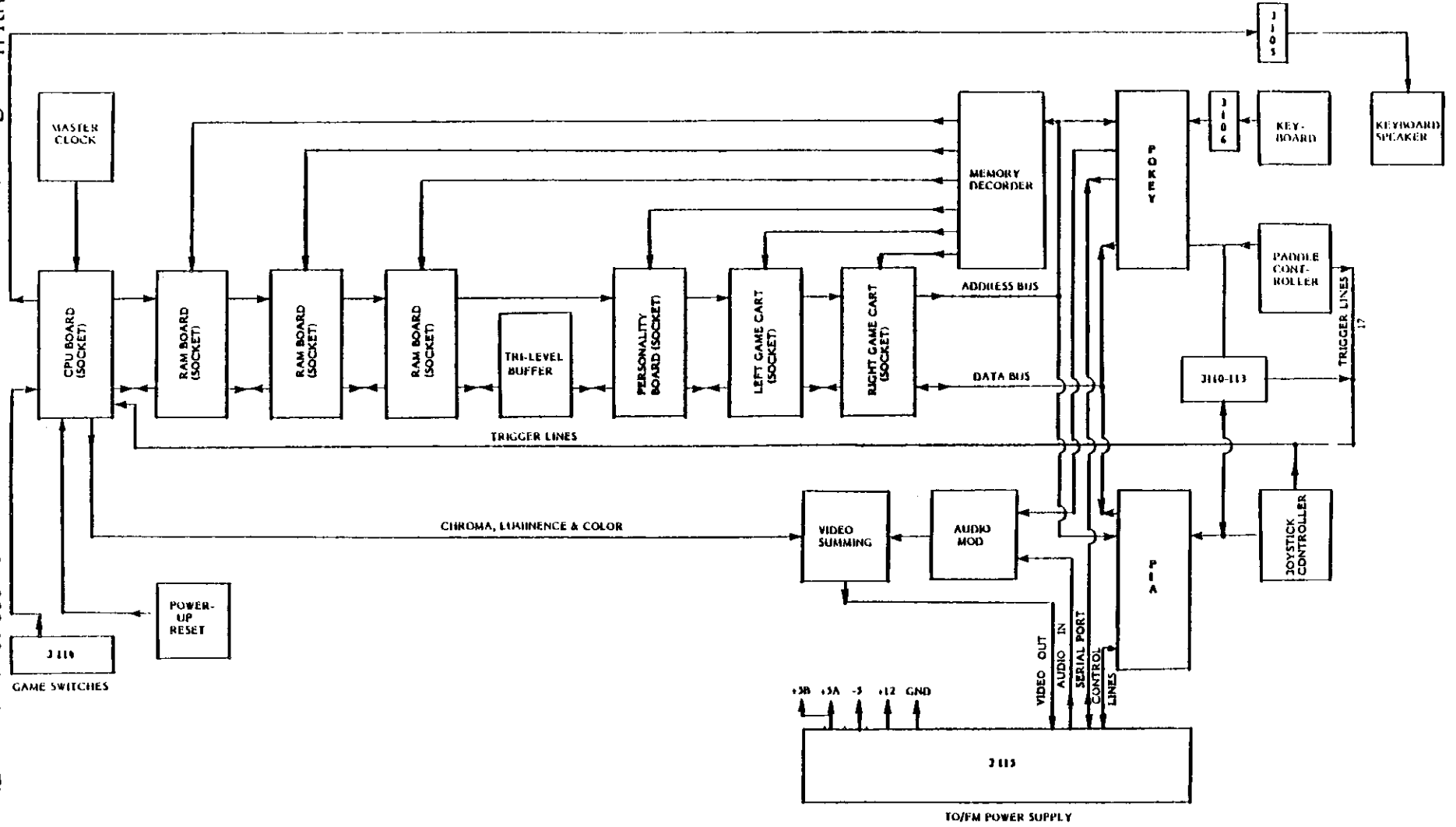
Figure 1-10. 800 Motherboard Flow Diagram
