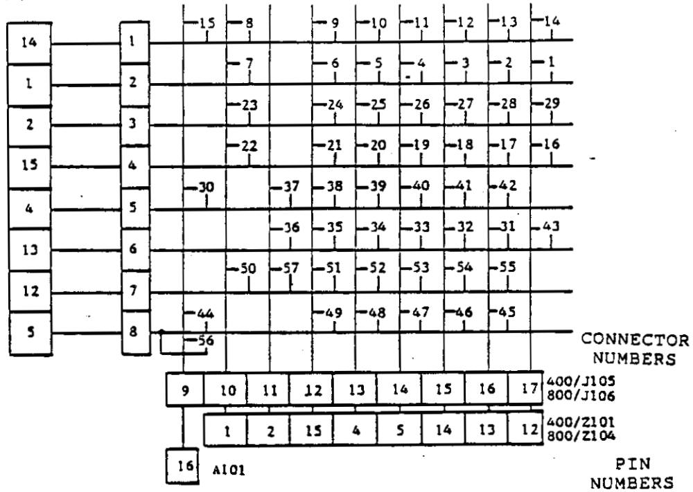
Keyboard Connection Chart
