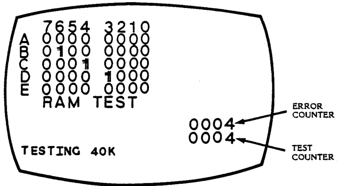
Defective RAM Identifier
