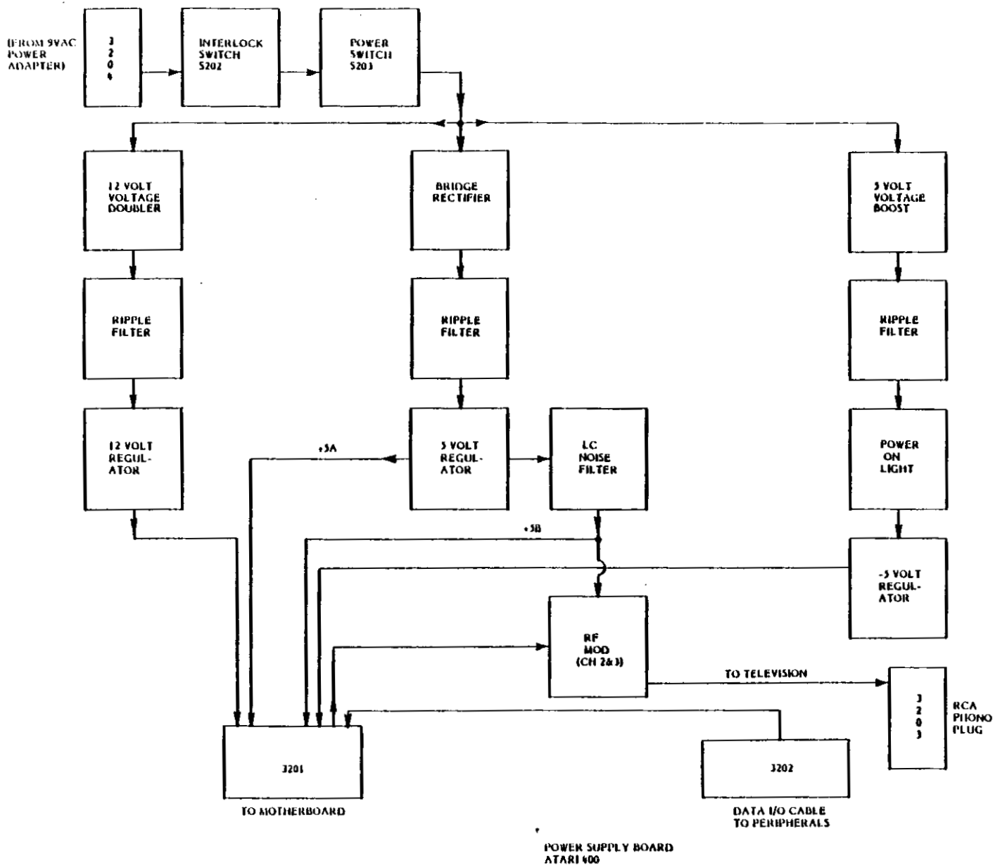
Figure 1-9. 400 Power Supply
