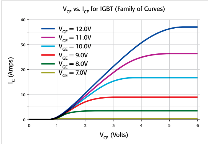
Figure 3. Measured output characteristics for commercially available IGBT.
