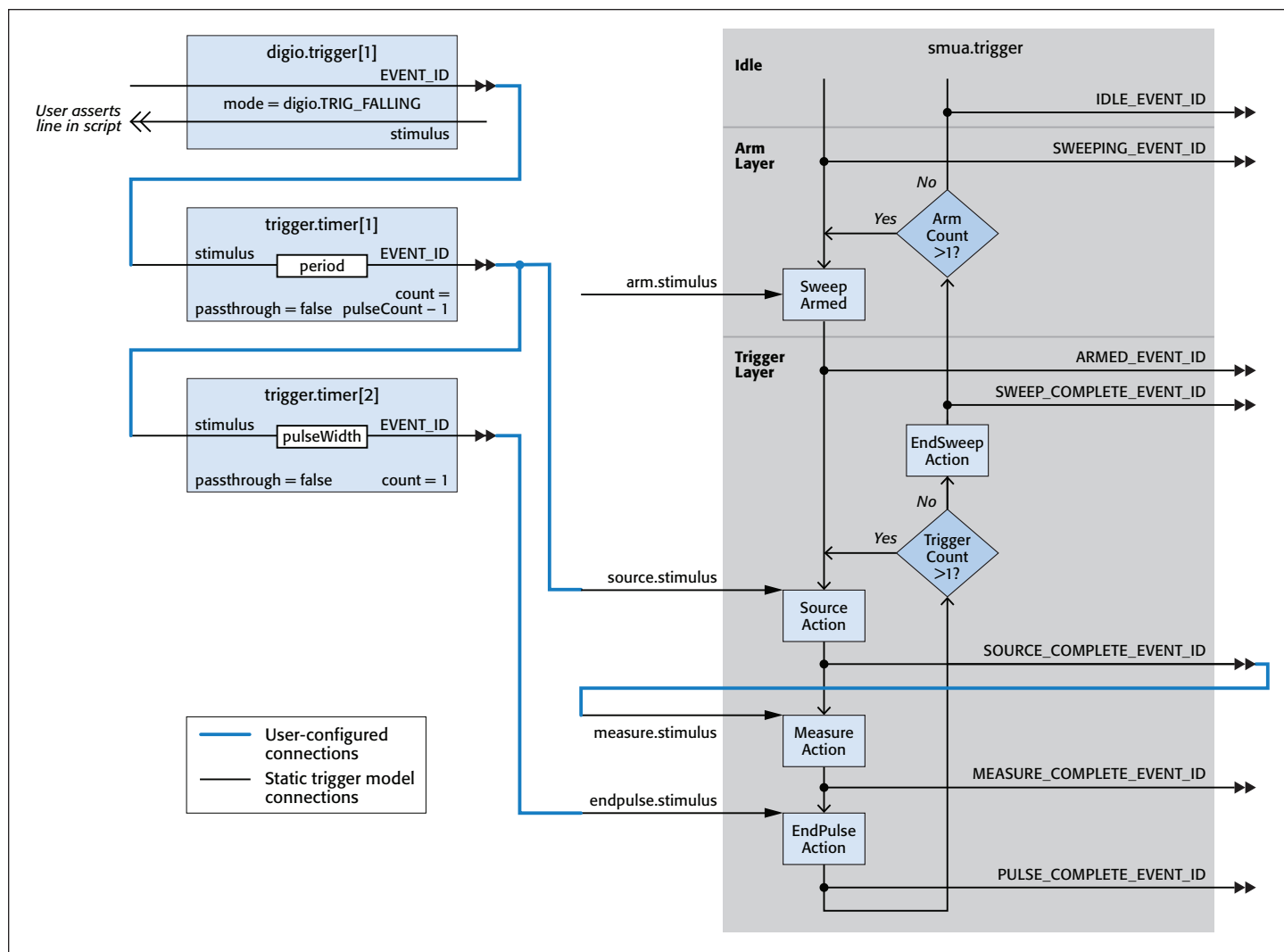
Figure 5. Trigger model configuration for Examples #1 and #2.
