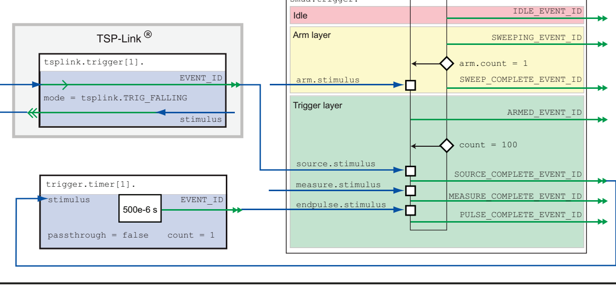
Figure 11: Example of a complete trigger model for Rds(on) sweep up to 100A.
