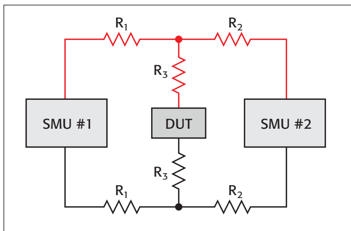
Figure 5: Model for test lead resistances.
