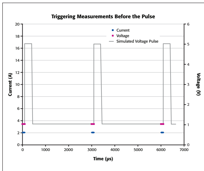
Figure 10. Results from Example #4. There is a 0.5\Omega resistive load.
