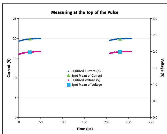
Figure 6. Results of Examples #1 and #2. The load is a 0.1\Omega resistor.
