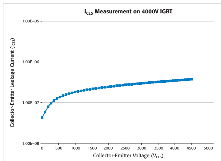
Figure 6. I CES measurements of 4000V IGBT. V CES is applied with the Model 2290-5 Power Supply, and I CES is measured with the Model 263xB SourceMeter SMU instrument. Gate and source terminals are shorted.
