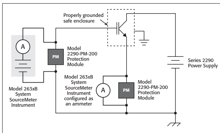
Figure 7b. Test setup using a Series 2290 Power Supply and two Model 263xB SourceMeter SMU instruments to measure the cutoff current (I CES ) of an IGBT. The SMU instrument connected to the gate terminal can be used to place a certain bias on the gate, e.g., to drive the device into hard cutoff.
