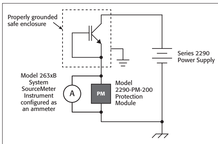
Figure 7a. Test setup using a Series 2290 Power Supply and the Model 263xB SourceMeter SMU Instrument to measure the cutoff current (I CES ) of an IGBT. The short between the gate and emitter terminals keeps the device in the off-state.
