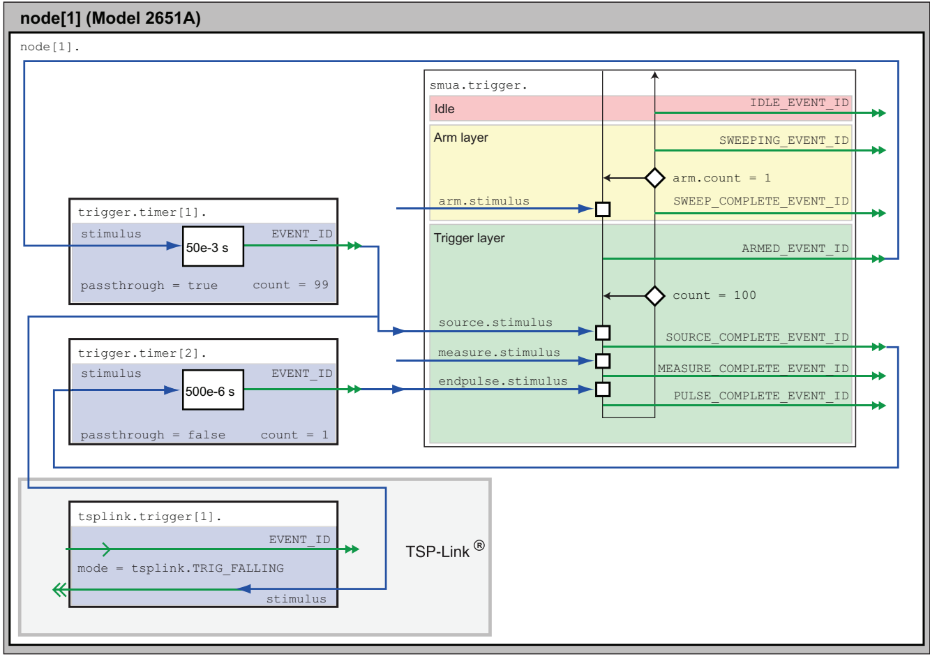
Figure 12: Example of a trigger model for 2651A #1 for Rds(on) sweep up to 100A.
