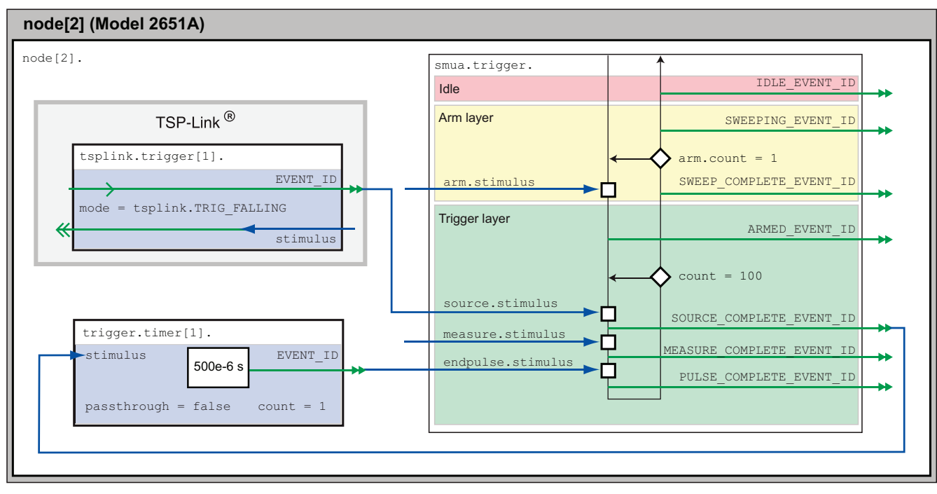
Figure 13: Example of a trigger model for 2651A #2 for Rds(on) sweep up to 100A.
