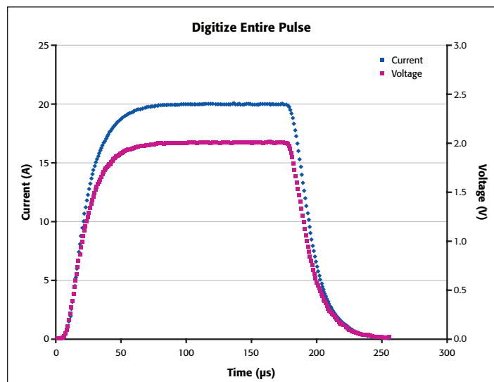
Figure 8. Results from Example #3 showing the voltage and current measurements as performed by the high speed ADCs. There is a 0.1Ω resistive load.
