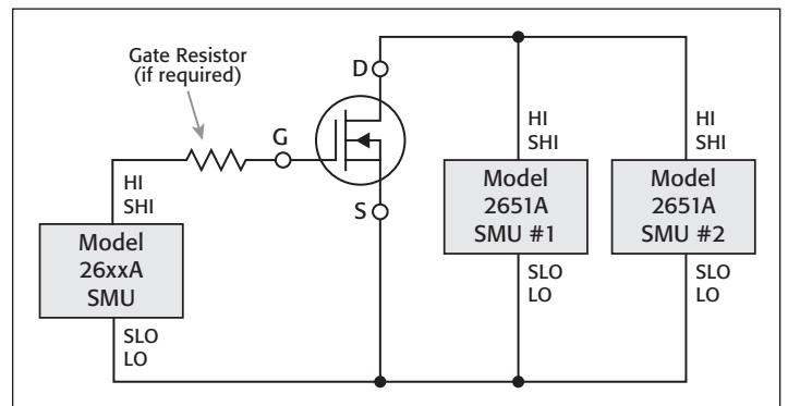
Figure 10: Connections for dual SMU Rds(on) sweep.
