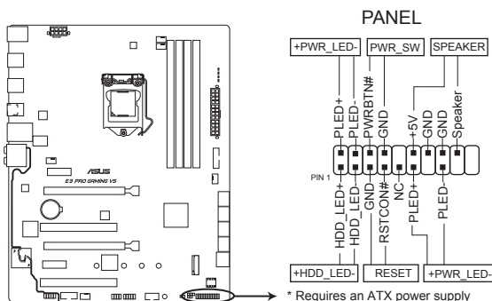
E3 PRO GAMING V5 System panel connector
