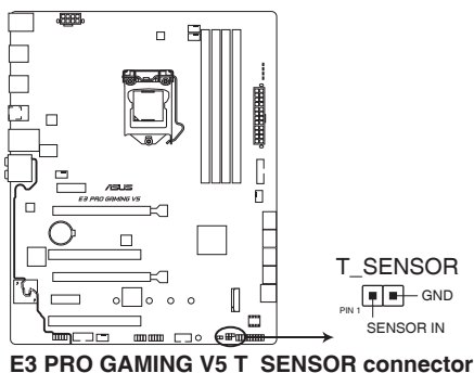
E3 PRO GAMING V5 T_SENSOR connector
