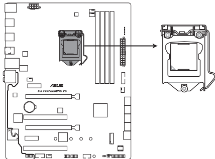
E3 PRO GAMING V5 CPU socket LGA1151
