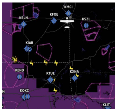
Lightning Data
