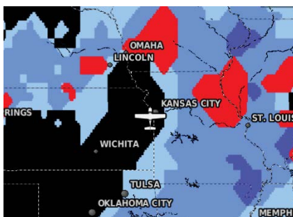
Icing Potential
