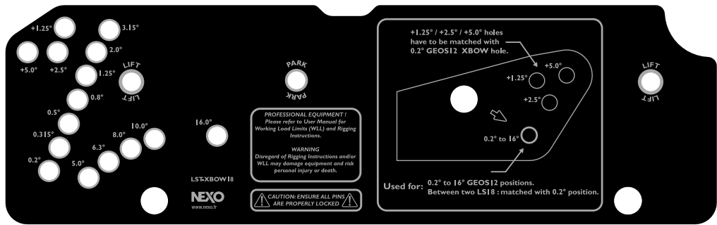
LS18 XBOW ANGLE SETTINGS PLATE
