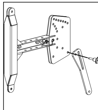
INSERTING PIN - STACKED SETUPS
