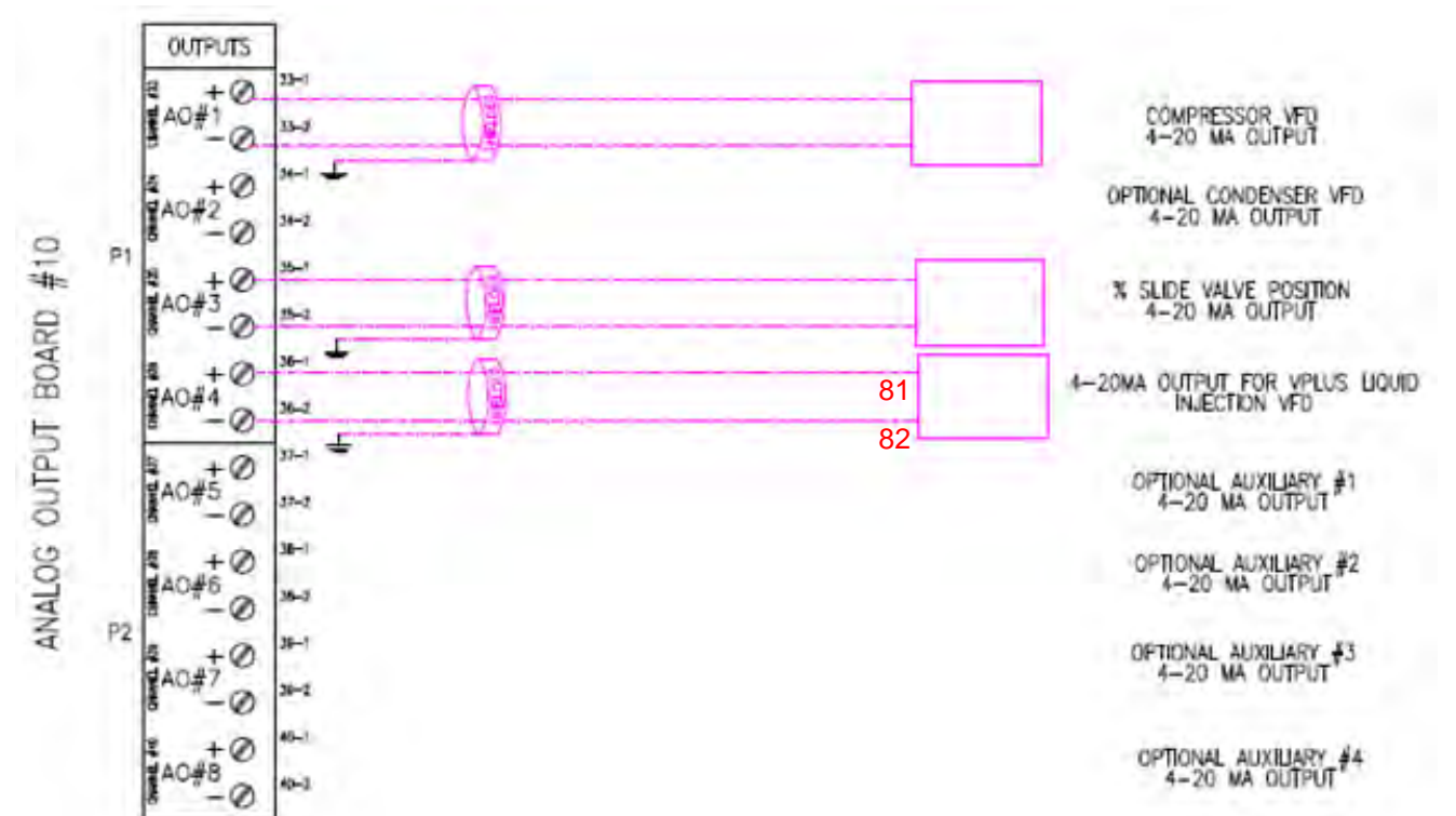
Figure B-22. Analog Output card wiring to VPLUS VFD controller
