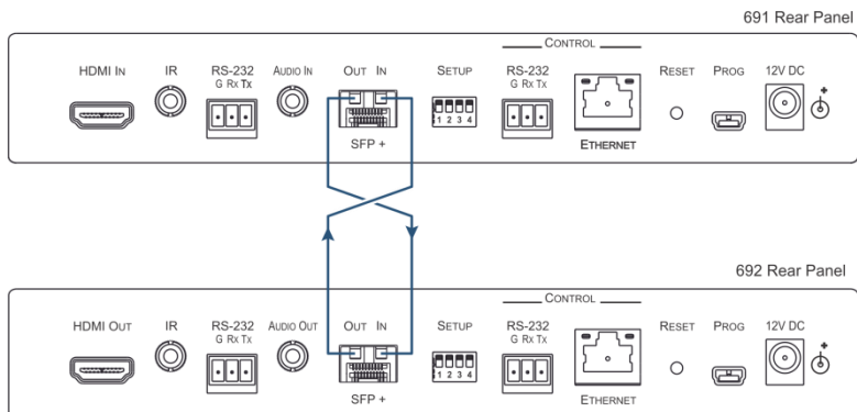
Figure 4: Connecting the Fiber Optic Cable
