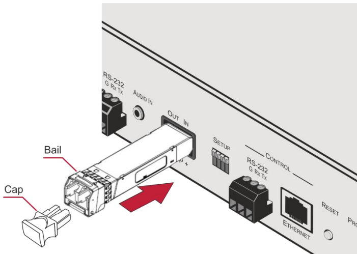
Figure 6: Inserting the Transceiver Module
