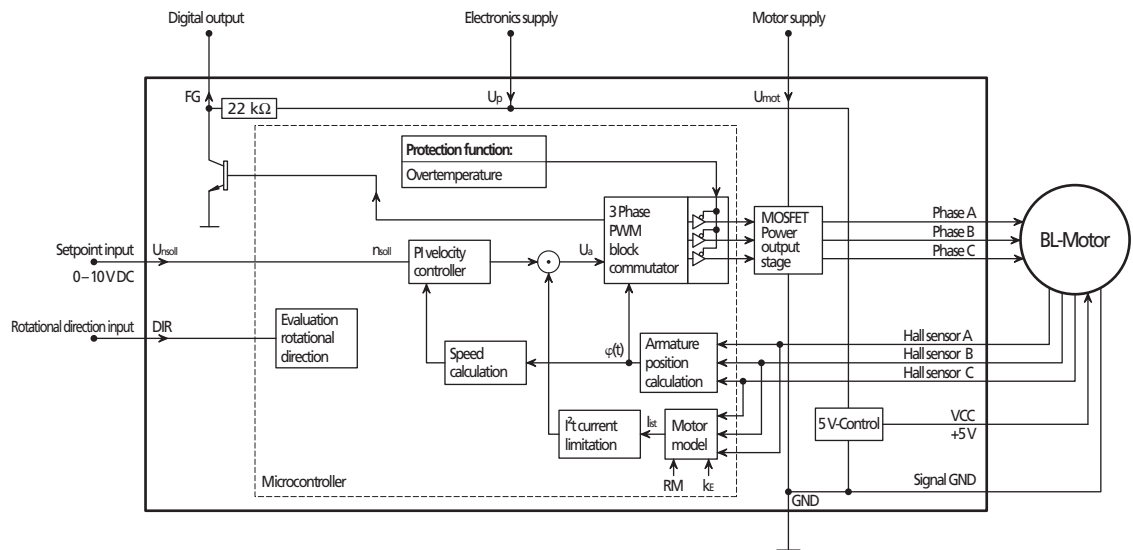
Block diagram
