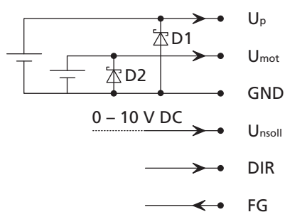
Circuit diagram 2
