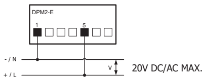
DC/AC 20V RANGE CONNECTION
