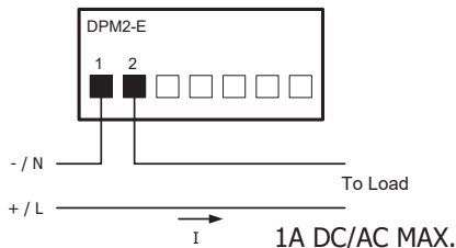
DC/AC DIRECT CONNECTION
