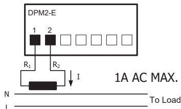
CONNECTION USING AN AC CURRENT TRANSFORMER
