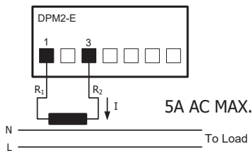
CONNECTION USING AN AC CURRENT TRANSFORMER
