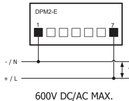
DC/AC 600V RANGE CONNECTION
