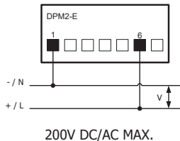
DC/AC 200V RANGE CONNECTION
