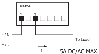
DC/AC DIRECT CONNECTION
