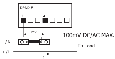
DC/AC SHUNT CONNECTION
