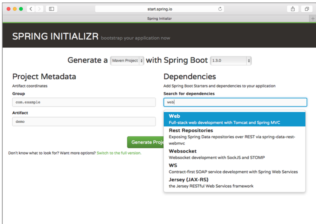
Figure 1.1 Spring Initializr is a web application that generates empty Spring projects as starting points for development.
