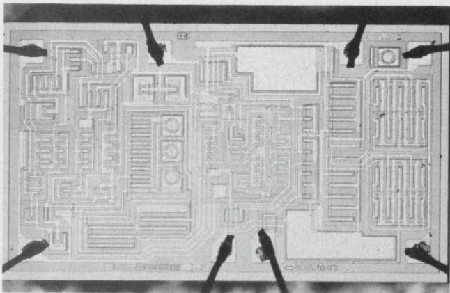
This monolithic JFET input op amp, National's LF 156, uses ion implantation to combine matched JFETs with bipolar transistors. It features very low noise and a low 1/f noise corner.
