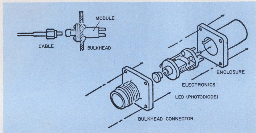
Fiber-optic connectors that use standard electrical connector shells are being used by the Navy to replace conventional wires with fiber optics.
