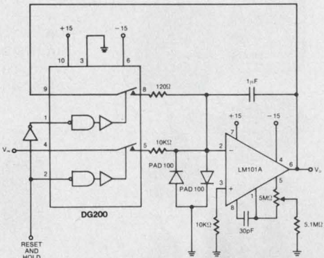
Typical Application: Integrator Reset & Hold
