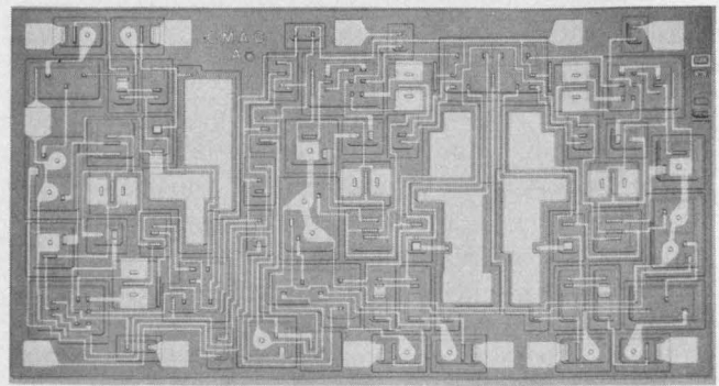
A new dual op amp designed for single-supply operation, Signetics' NE532, uses a Darlington input stage that can be driven slightly below ground ( -0.3 \text{ V} ).
