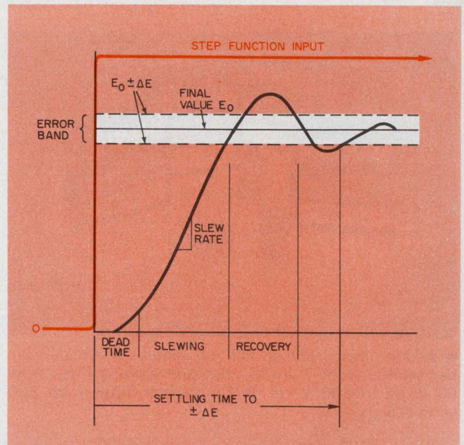
The most complete definition of settling time considers the dead time, slewing, recovery and settling of the output to within the tolerance of the error band.
