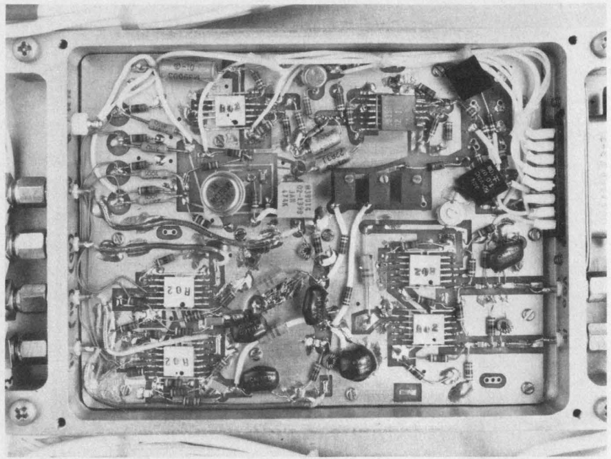
A 3 × 4-in. module contains a complete quadriphase demodulator, including the "IQ" loop, which provides carrier reconstruction. The compact unit employs 1-GHz bipolar-logic ICs developed by Motorola.
