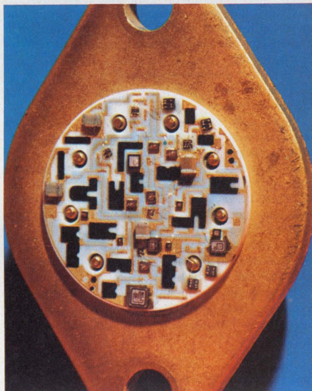
Hybrid technology makes possible this high-voltage op amp, the 3582J, by Burr-Brown. The device can provide 15 mA at \pm 145 V ac into a 2-k \Omega load, with a \pm 150 -V-dc supply.
