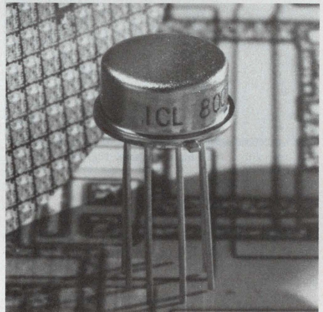
Very low input current of 1 pA max and low offset voltage of 2 mV max are features in this 8007 FET-input op amp by Intersil. Input impedance is 10^{12} ohms.
