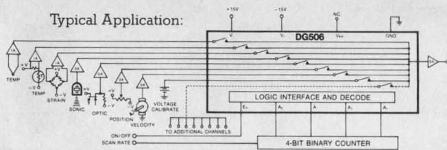
Sequential 16-Transducer Scanner (8 channels illustrated)
