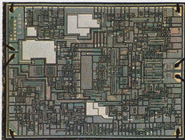
This monolithic chopper-stabilized amplifier, by Harris, has an offset voltage drift of only 0.2 \mu V/ ^{\circ} C. Open loop gain is 5 \times 10^8 , bandwidth is 3 MHz and slew rate is 2.5 V/ \mu s.
