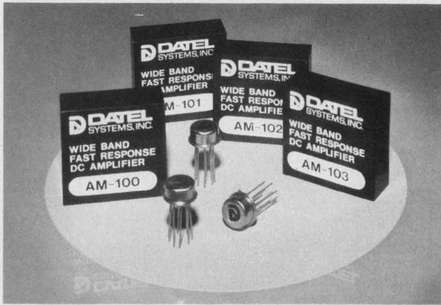
Wideband, fast settling FET op amps, by Datel, have bandwidths from 7 to 45 MHz and slewing rates from 60 \text{ V}/\mu\text{s} to 400 \text{ V}/\mu\text{s} . Settling times range from 300 ns to 2.5 \mu\text{s} .
