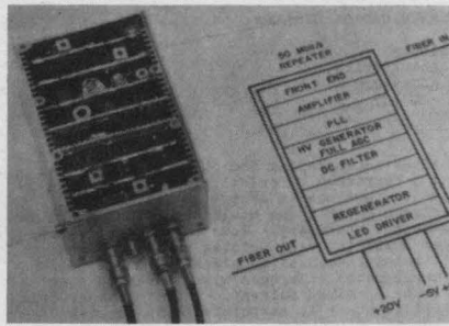
An experimental 50 Mb/s repeater developed by Bell Laboratories can be used to regenerate optical data.
