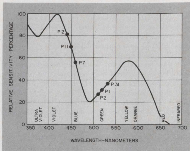
5. Relative sensitivity vs phosphor type for Polaroid 410 film. Note the difference in sensitivities for P11 at 450 nm and P31 at 530 nm.
