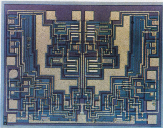
Dual high performance op amps on this chip, by Texas Instruments, are protected against shorts and against latchup. No external frequency compensation is needed.
