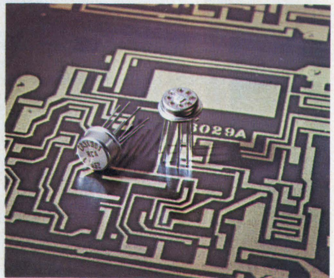
The first op amp to combine bipolar and CMOS on one chip, the RCA 3130, has a CMOS pair that is capable of swinging the output voltage to within 10 mV of either supply terminal.
