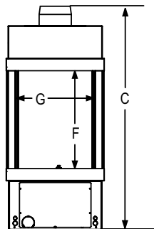
LEFT VIEW
