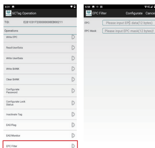
Figure 7-12 EPC Filter
