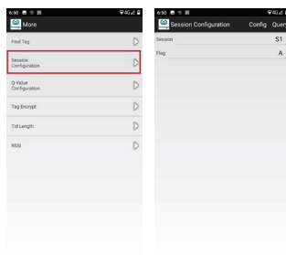
Figure 6-8 Session Configuration
