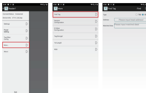
Figure 6-7 Search Tag
