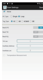
Figure 6-4 Scan settings
