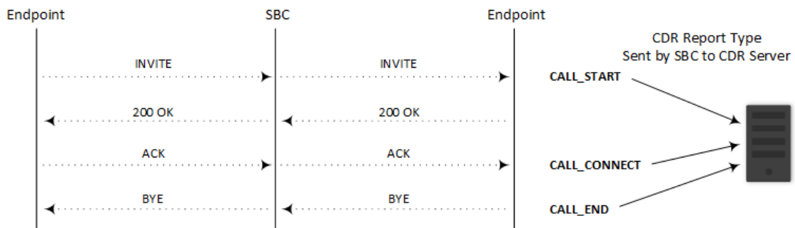
Figure 55-3: CDR Report Types for SBC Signaling
