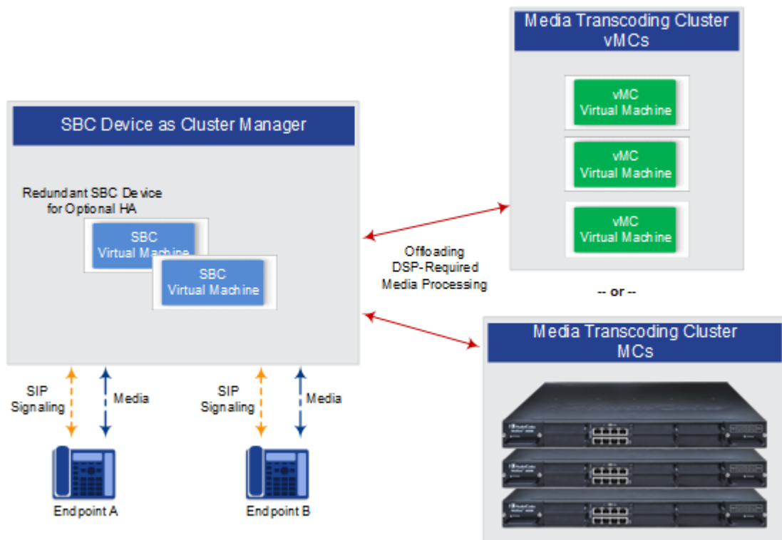
Figure 34-2: Overview of Media Transcoding Cluster Mode
