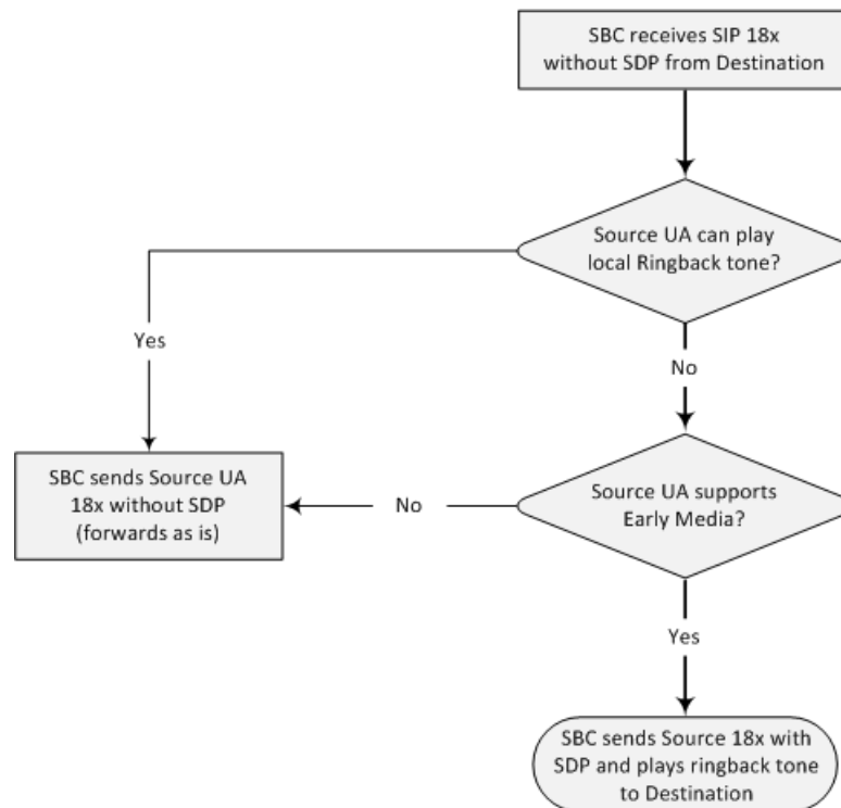
Figure 24-2: SBC Early Media RTP 18x without SDP
