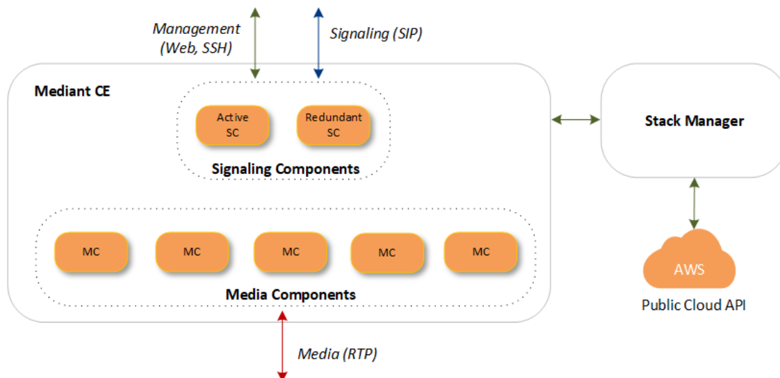
Figure 34-1: Mediant CE Architecture
