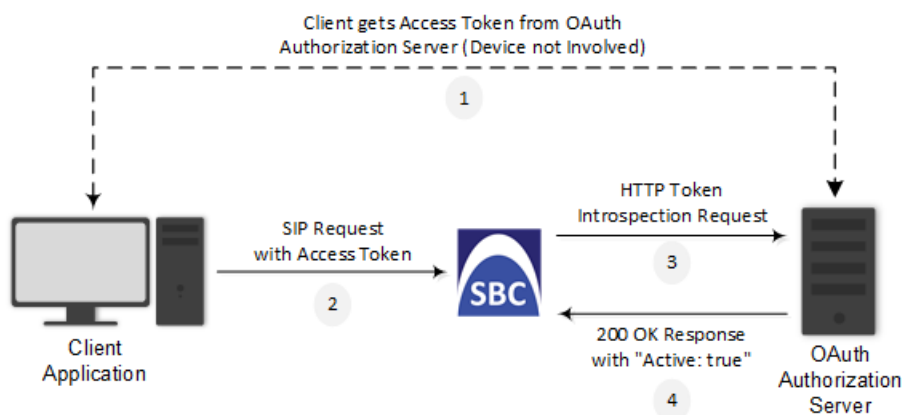
Figure 24-1: General Stages of OAuth-based Authentication
