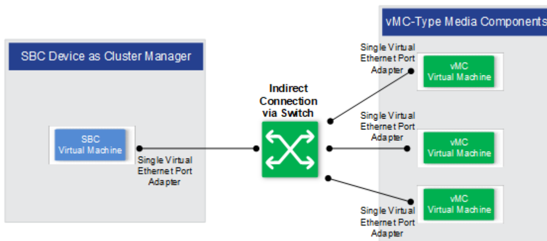
Figure 34-4: Indirect Connection between vMC Media Components and SBC Device
