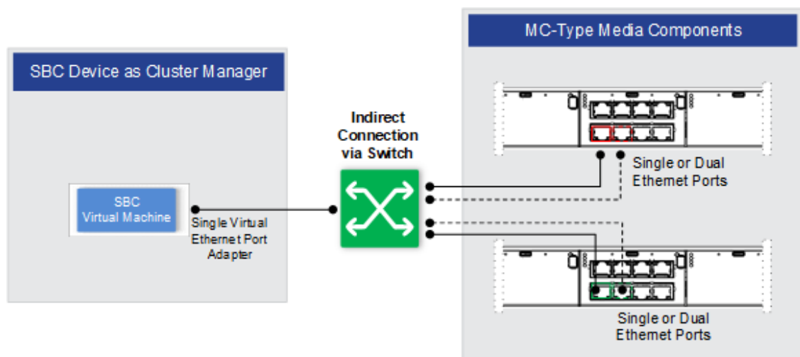
Figure 34-3: Indirect Connection between MC Media Components and SBC Device
