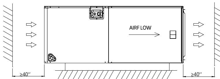
Indoor units installation space requirements in the horizontal position
