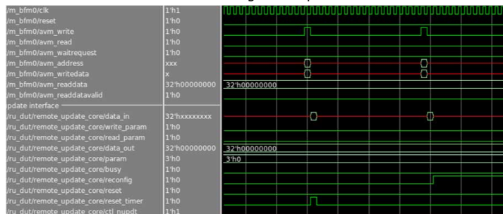
Figure 8. Waveform for Reset Timer and Reconfiguration Operation
