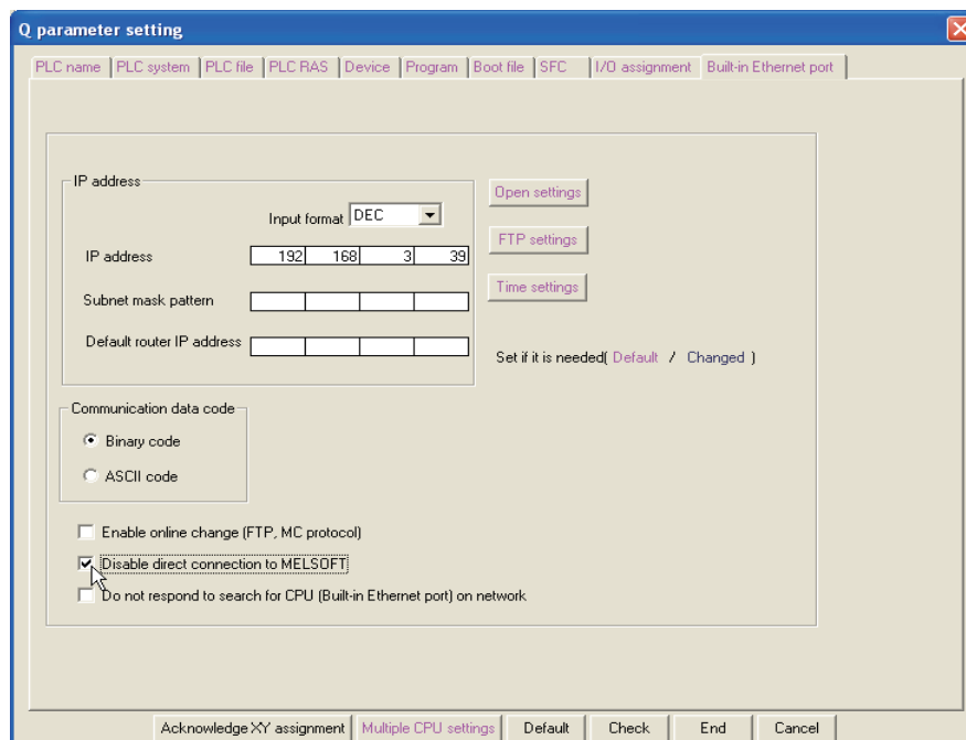
Figure 3.15 Setting for preventing direct connection
