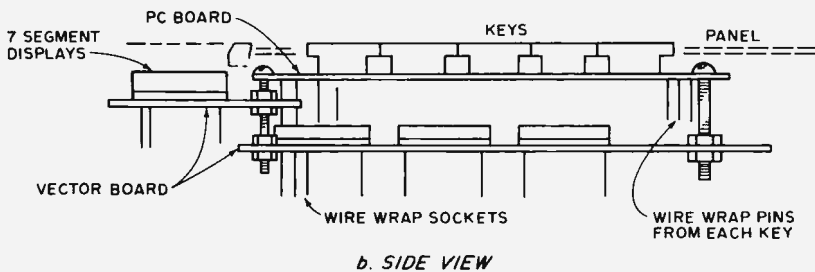
Figure 4: Mechanical Layout of the Author's Unit. The placement of parts is shown schematically in this illustration. The octal keys are at the lower left portion of the keyboard; the remaining keys are function buttons for the author's 6502 computer system.
