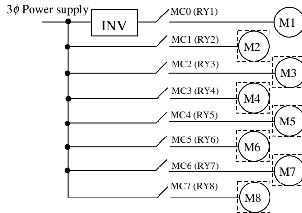
Fig 1 variable frequency pump fixed mode.
