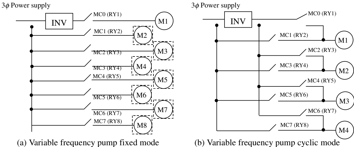
Fig 4 Variable pump driven mode
