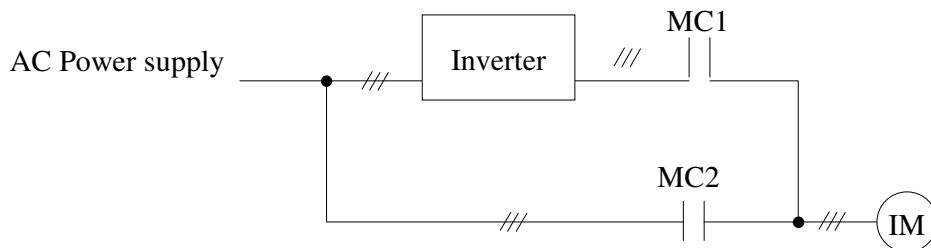
Fig 3 Switching of inverter driving to commercial AC power supply
