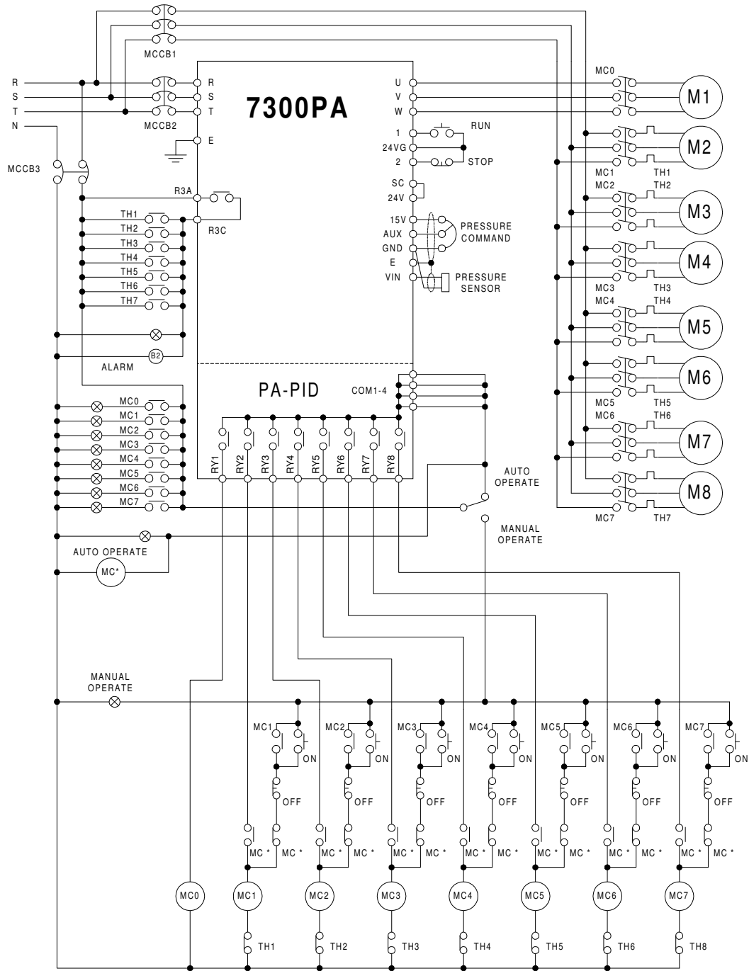
Fig 5 Fixed mode wiring diagram
