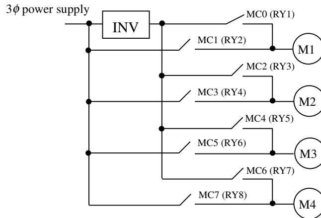
Fig 2 variable frequency pump cyclic mode.
