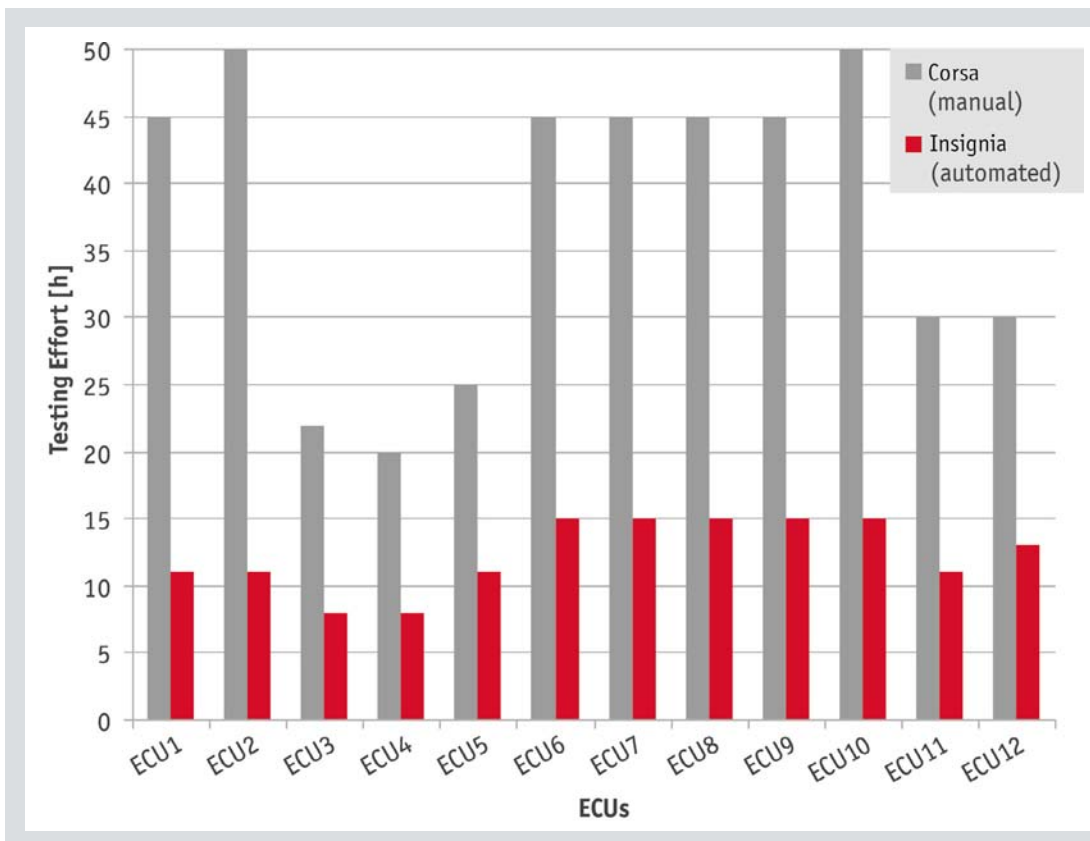
Figure 6: Test effort per ECU on the Opel Corsa with manual validation, compared to automated validation of diagnostic services on the Opel Insignia (execution and evaluation time)
