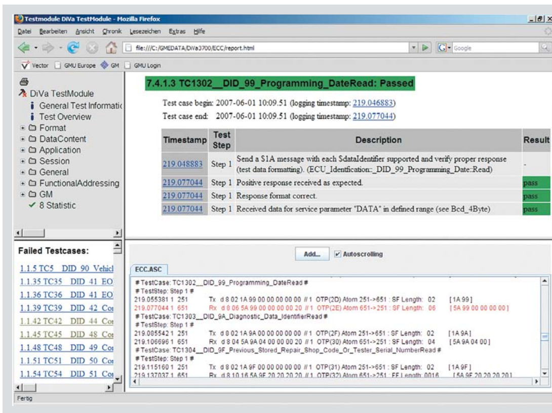
Figure 5: Automatically generated test report in DiVa
