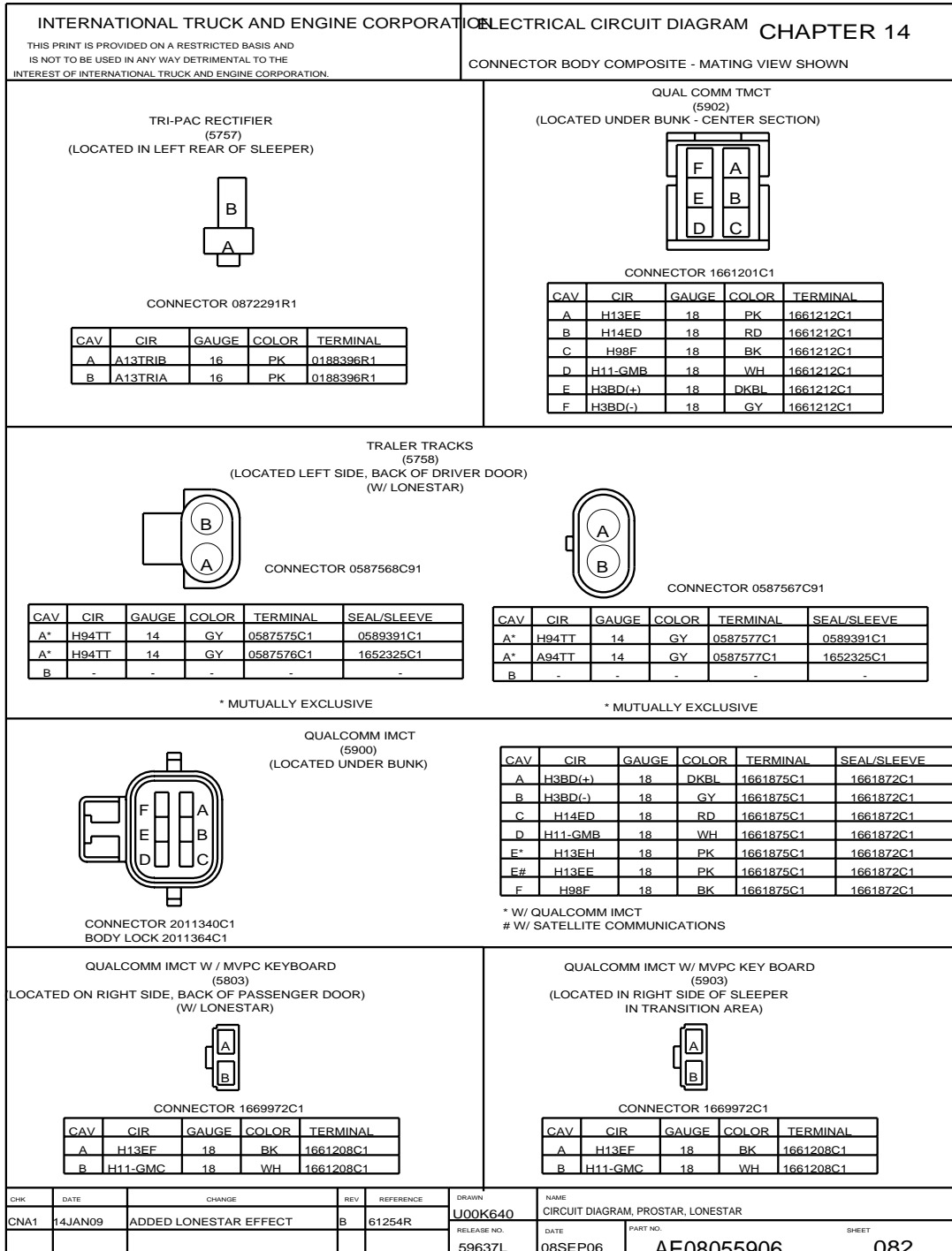
Figure 333 Connector Composites (5757), (5758), (5803), (5900), (5902), (5903)
