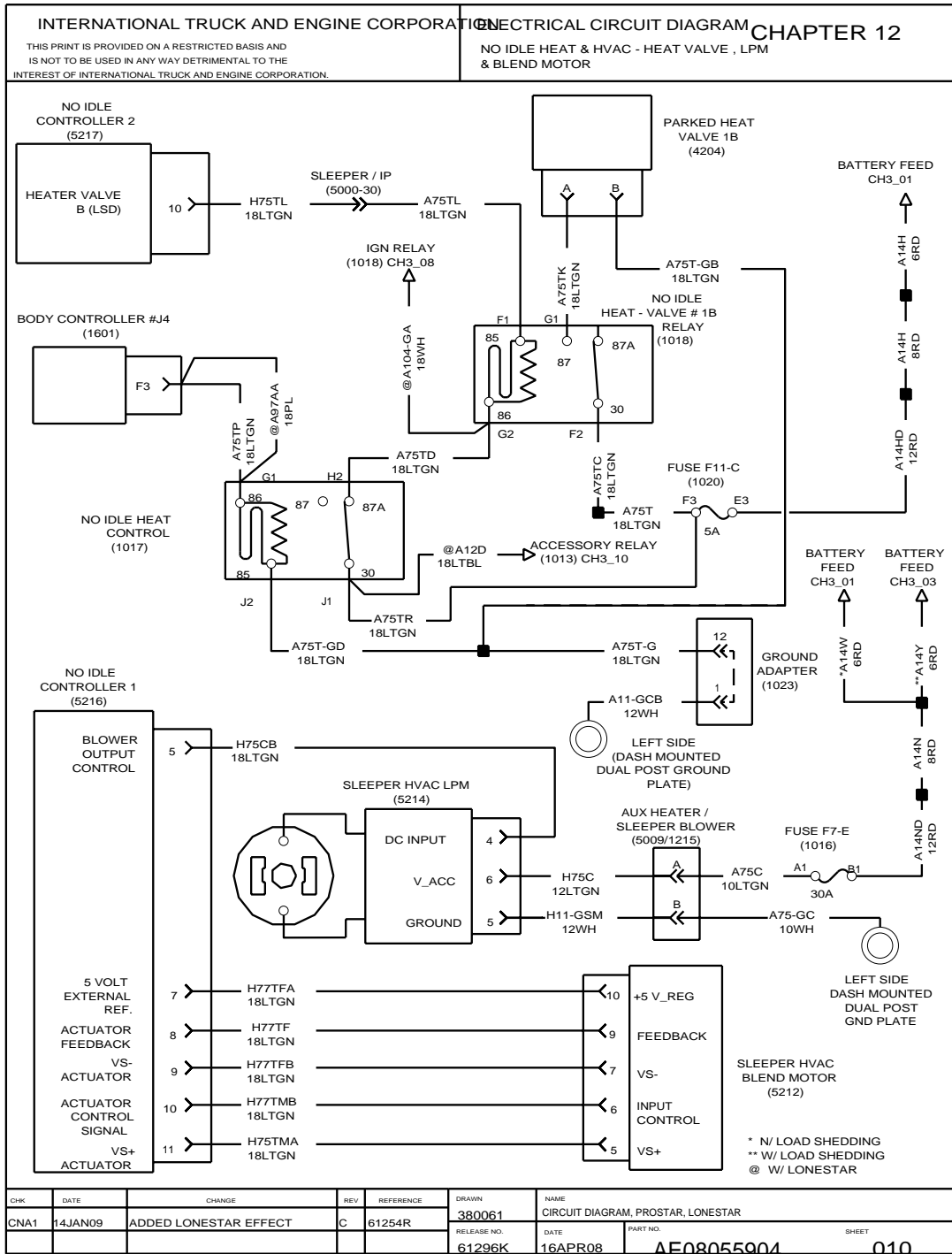
Figure 211 No Idle Heat and HVAC — Heat Valve, LPM and Blend Motor
