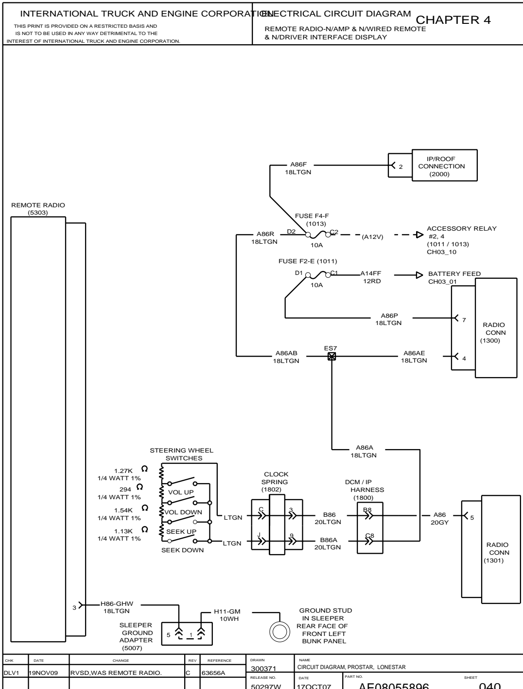
Figure 94 Remote Radio — N/AMP and N/Wired Remote and N/Driver Interface Display
