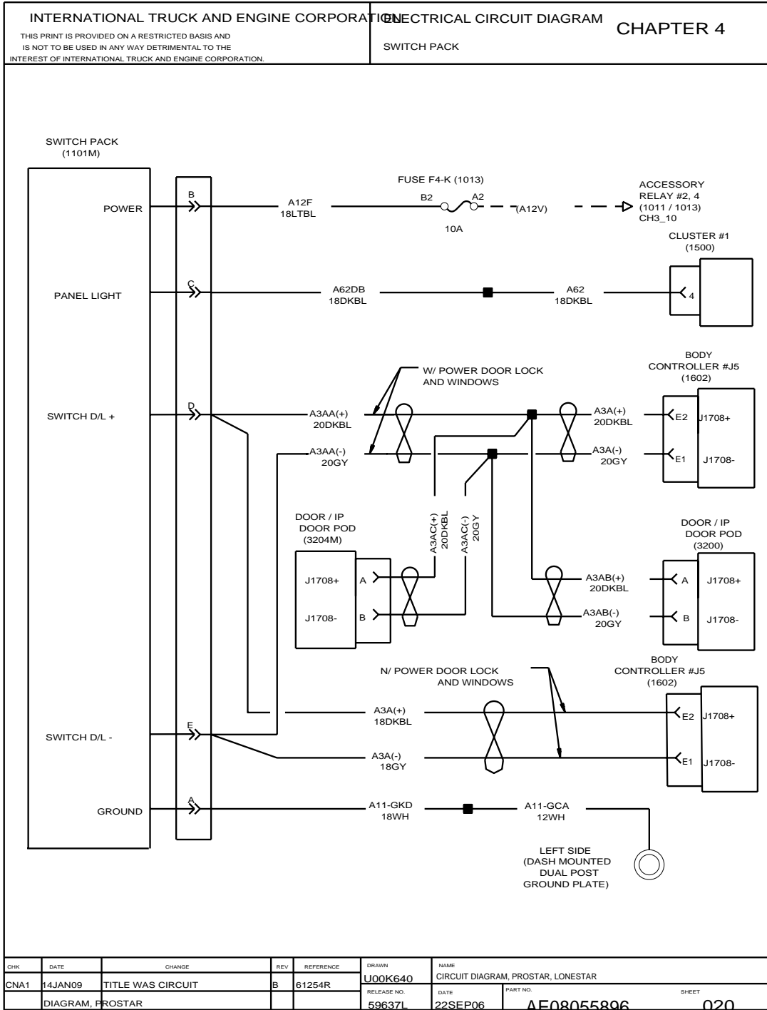
Figure 72 Switch Pack
