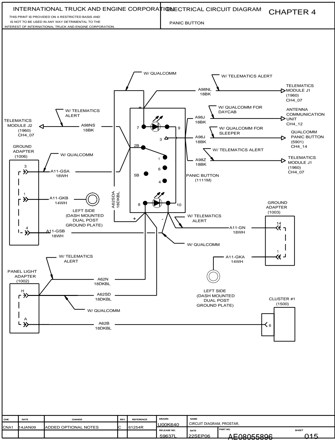
Figure 65 Panic Button
