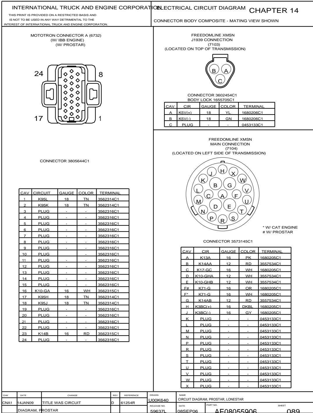
Figure 349 Connector Composites (6732), (7103), (7104)
