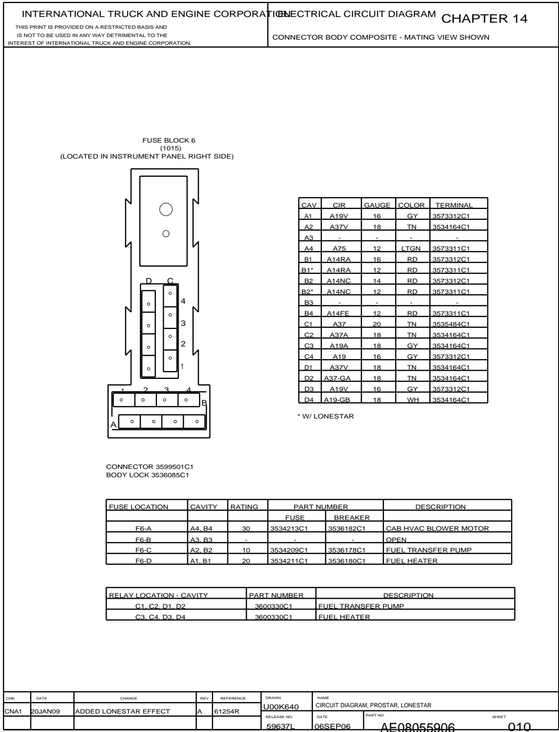
Figure 241 Connector Composite (1015)
