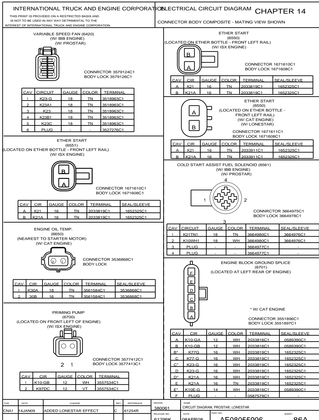
Figure 343 Connector Composites (6420), (6550), (6551), (6561), (6650), (6700), (6701)
