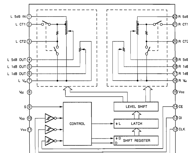
IC304 LC7535
