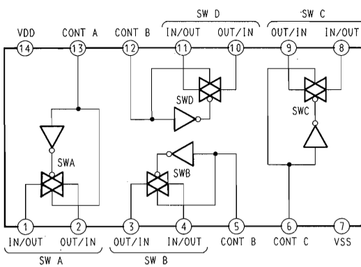
IC301 LC4966
