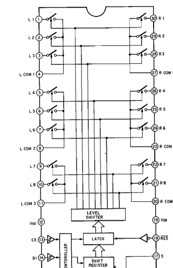
IC402 LC7822
