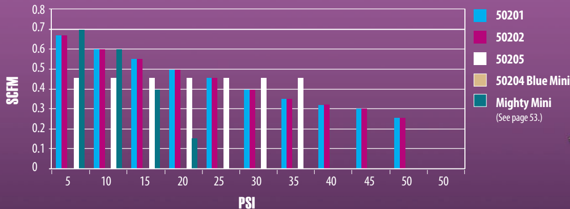
Compressor PSI Ratings at 60 psi
