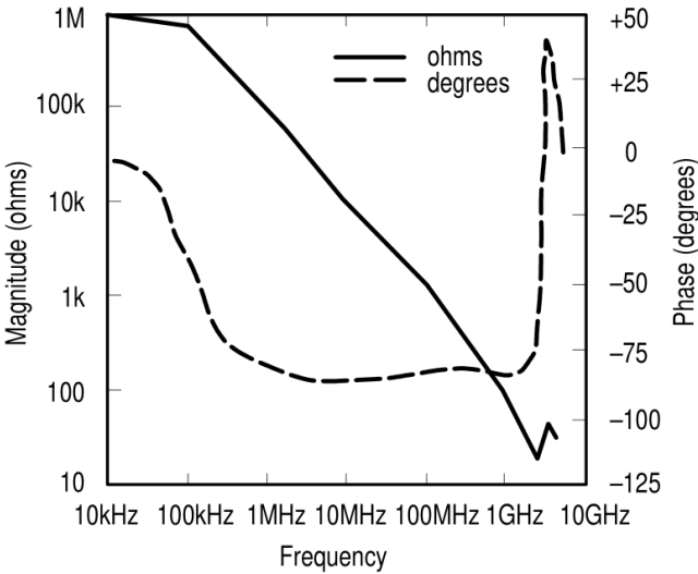
Figure 4.5. Typical input impedance versus frequency for an active probe.
