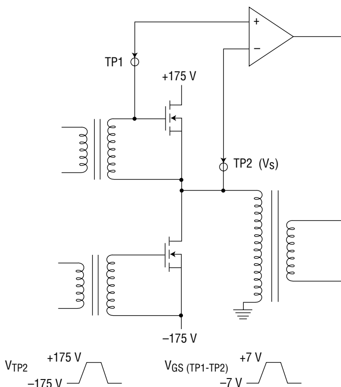
Figure 6.8. Differential amplifier used to measure gate to source voltage of upper transistor in an inverter bridge. Note that the source potential changes 350 volts during the measurement.
