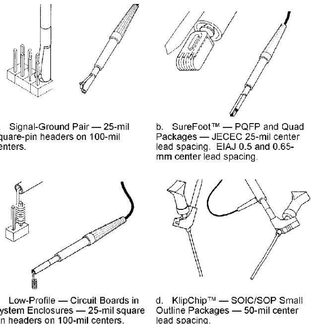
Figure 2.15. Some examples of probe tip adapters for small geometry probes. Such adapters make probing of small circuitry significantly easier and can enhance measurement accuracy by providing high integrity probe to test point connections.
