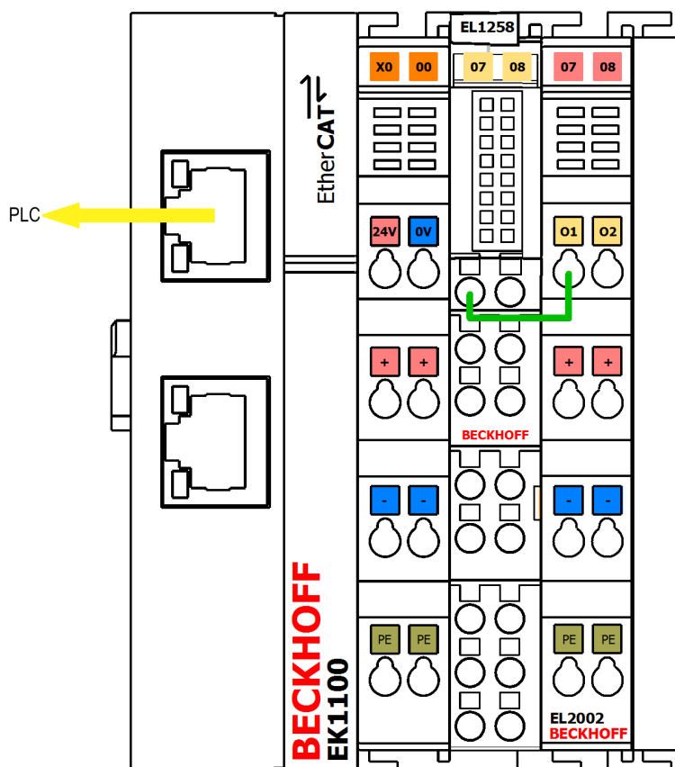
Fig. 181: Recommended structure for the EL1258 sample program
