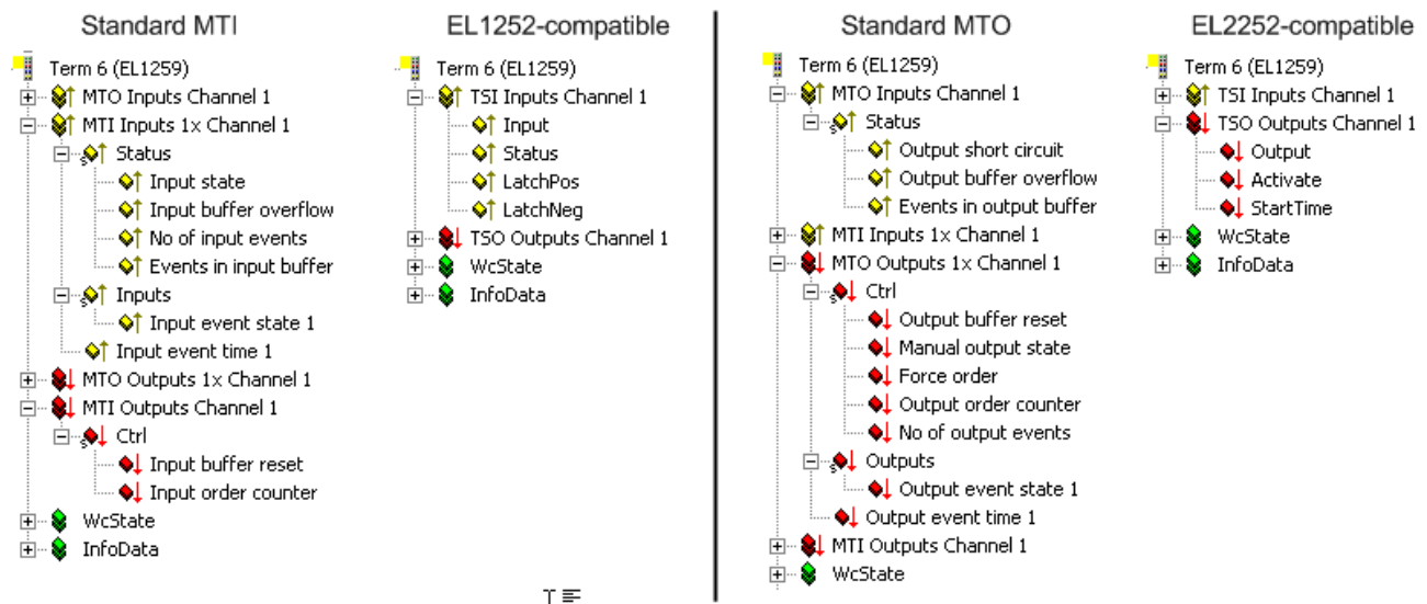
Fig. 155: Option for setting of compatibility modes in relation to EL1252/EL2252
