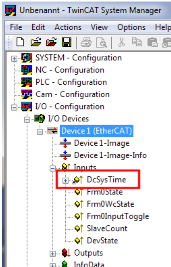
Fig. 176: Extended process image of the EtherCAT master
