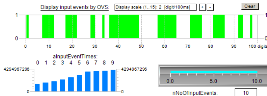
Fig. 184: Sample program EL1258 / Visualization_2: Display of incoming events in chronological order according to the timestamps of the EL1258
