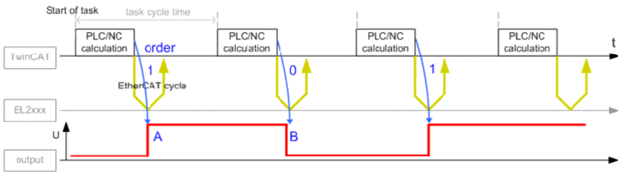
Fig. 17: Output of output channel information, standard
