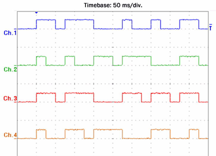
Fig. 180: Recording of four channels by the Multi-Timestamp program example
