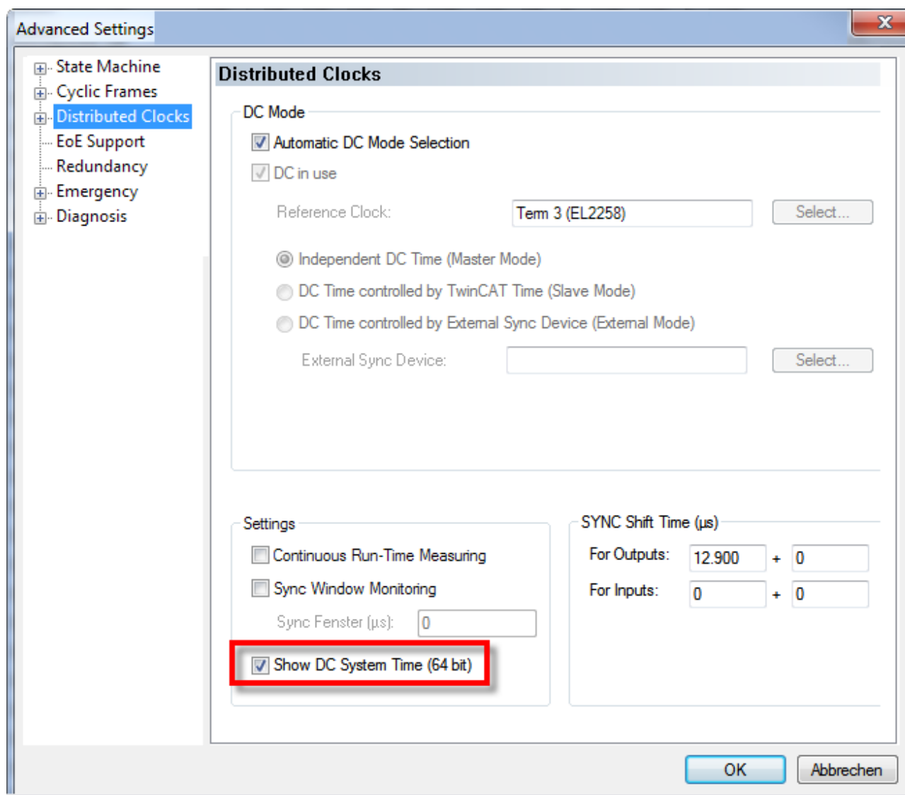
Fig. 175: Activation of the master distributed clock display
