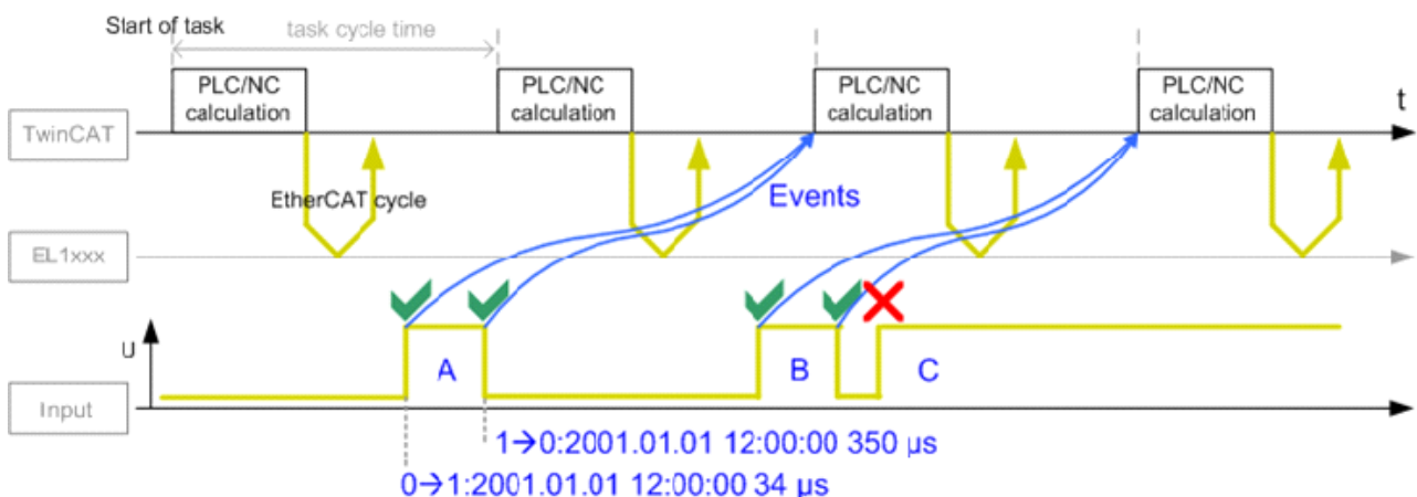
Fig. 16: Query of input channel information, with timestamp
