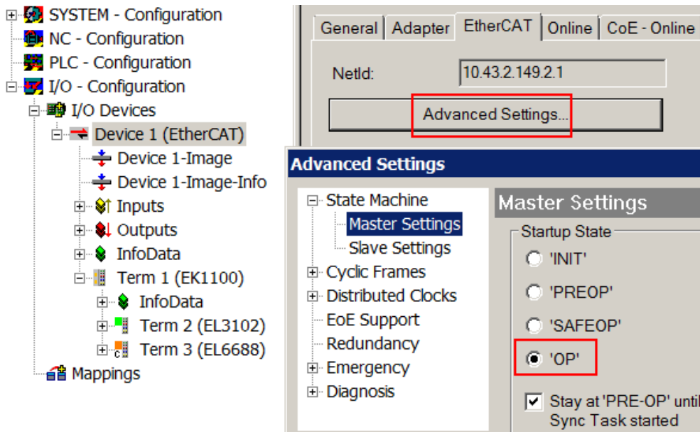
Fig. 148: Default behaviour of the System Manager
