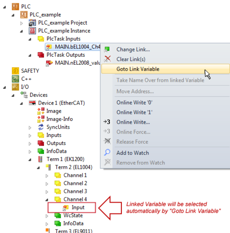
Fig. 81: Application of a “Goto Link” variable, using “MAIN.bEL1004_Ch4” as a sample
