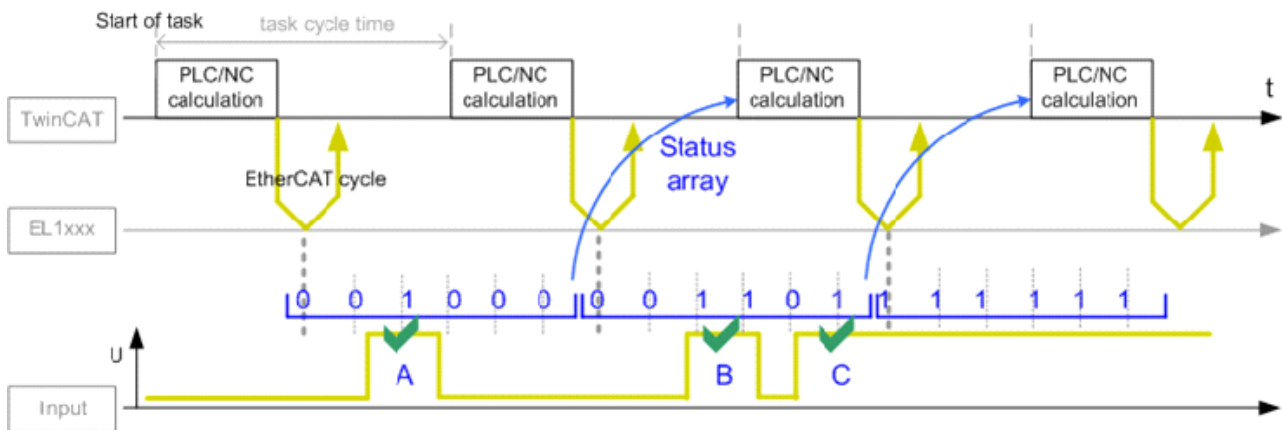
Fig. 15: Query of input channel information, oversampling
