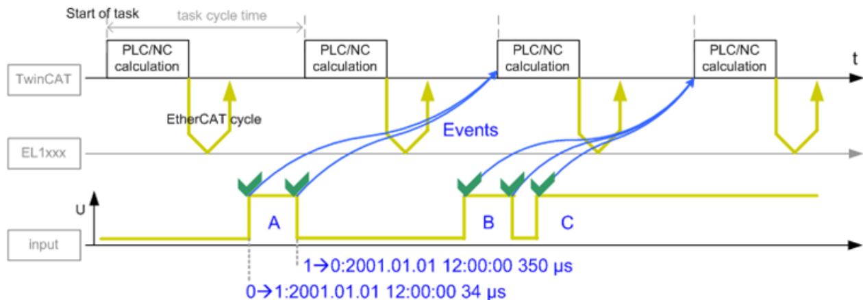
Fig. 20: Query of input channel information, with multi-timestamp
