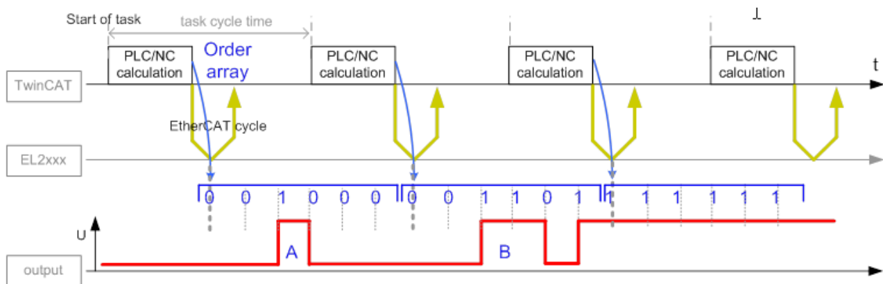
Fig. 18: Output of output channel information, oversampling
