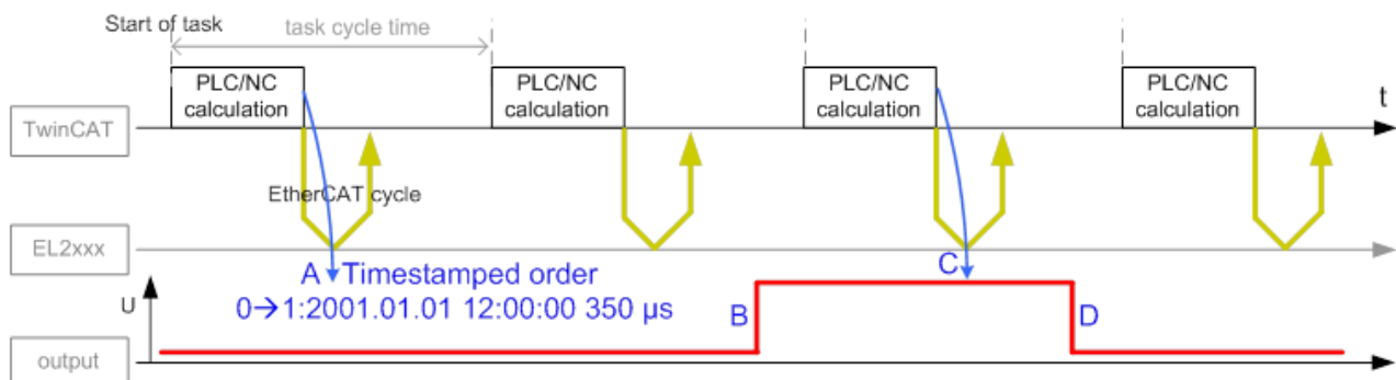
Fig. 19: Output of output channel information, with timestamp
