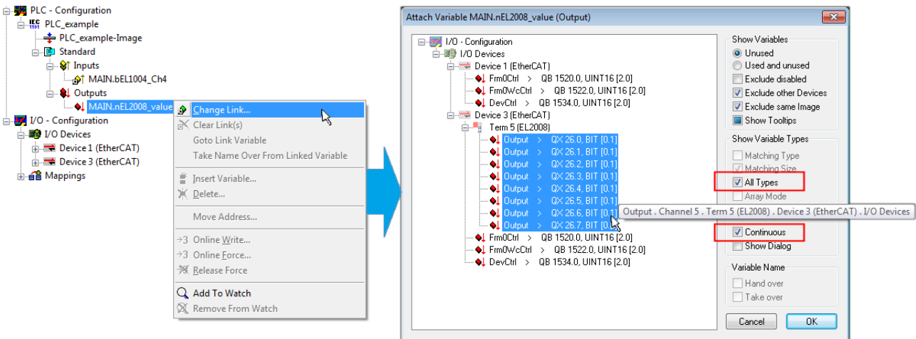
Fig. 60: Selecting several PDOs simultaneously: activate “Continuous” and “All types”
