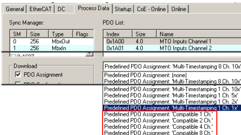
Fig. 167: Predefined PDOs for compatibility mode
