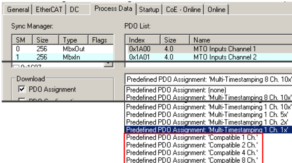
Fig. 174: Predefined PDOs for compatibility mode
