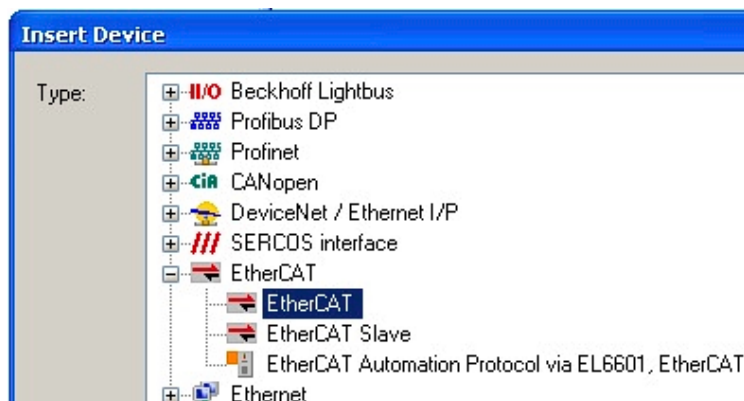
Fig. 104: Selecting the EtherCAT connection (TwinCAT 2.11, TwinCAT 3)
