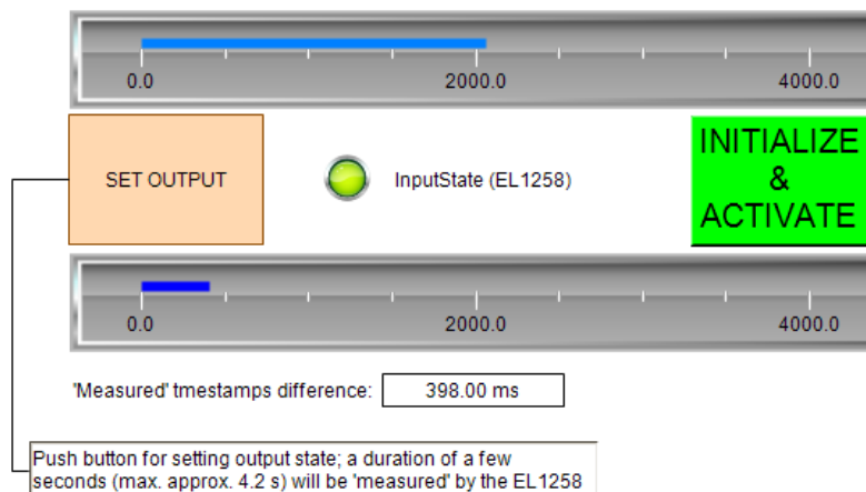
Fig. 183: Sample program EL1258 / Visualization_1: simple time measurement based on two state changes
