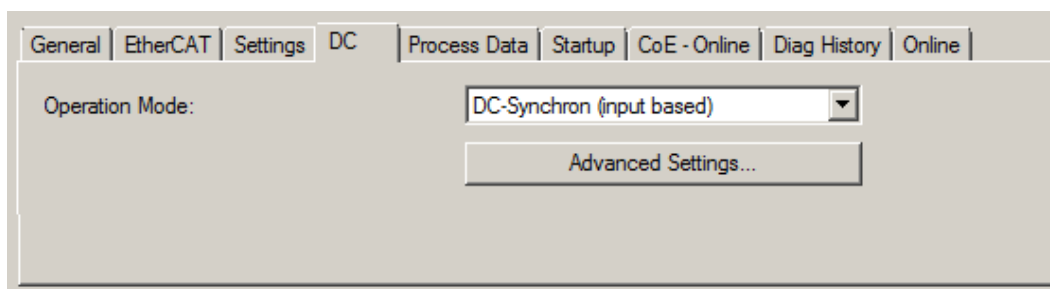
Fig. 143: "DC" tab (Distributed Clocks)
