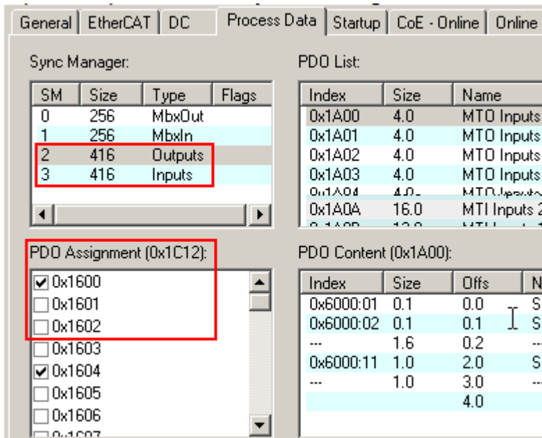
Fig. 157: Free selection of the PDO
