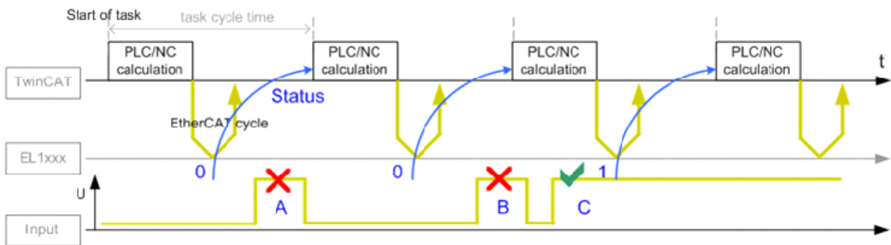
Fig. 14: Query of input channel information, standard
