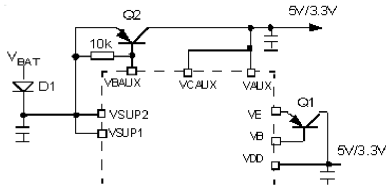
Figure 32. V AUX increased current capability without current limit schematic
