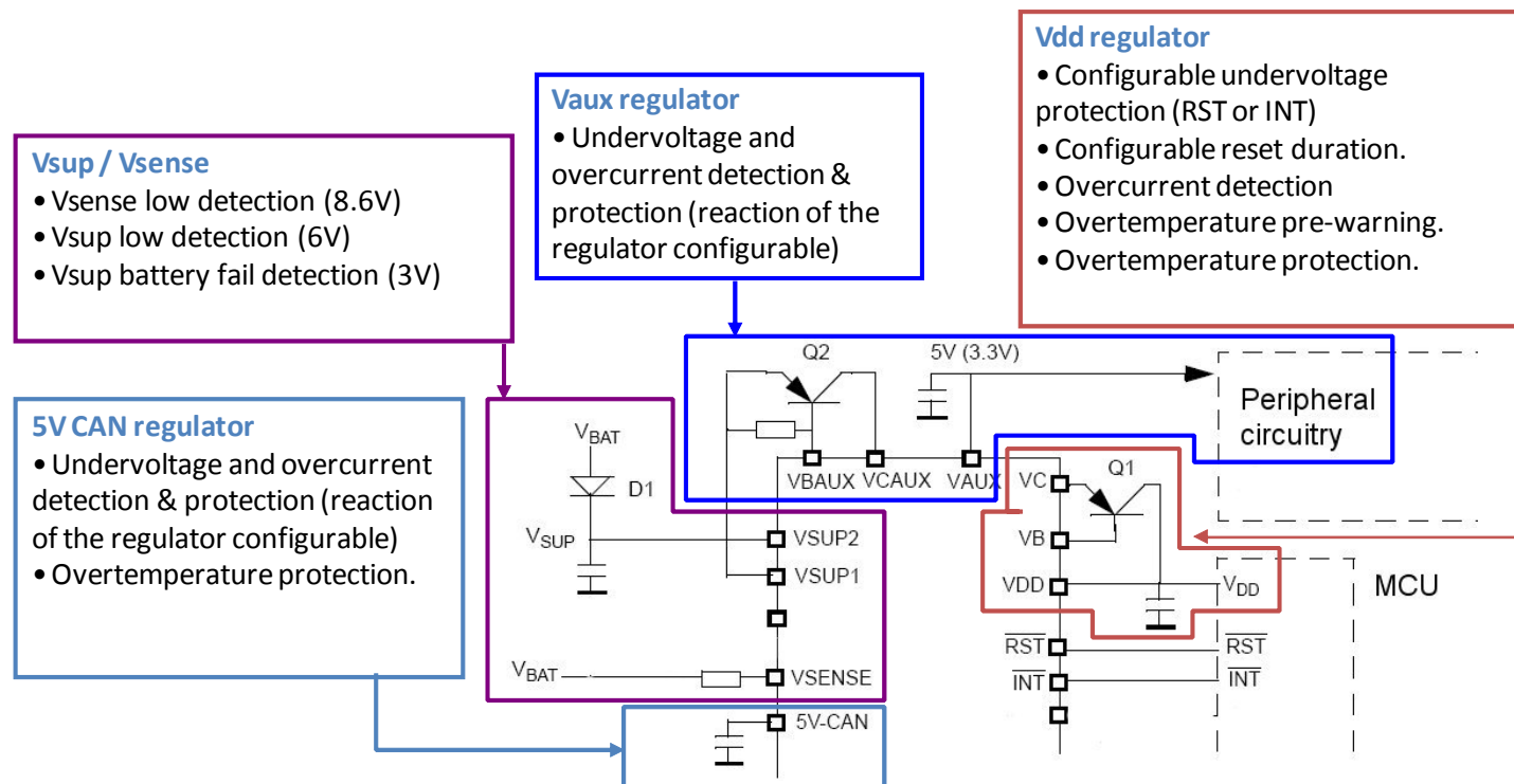
Figure 75. Supply monitoring
