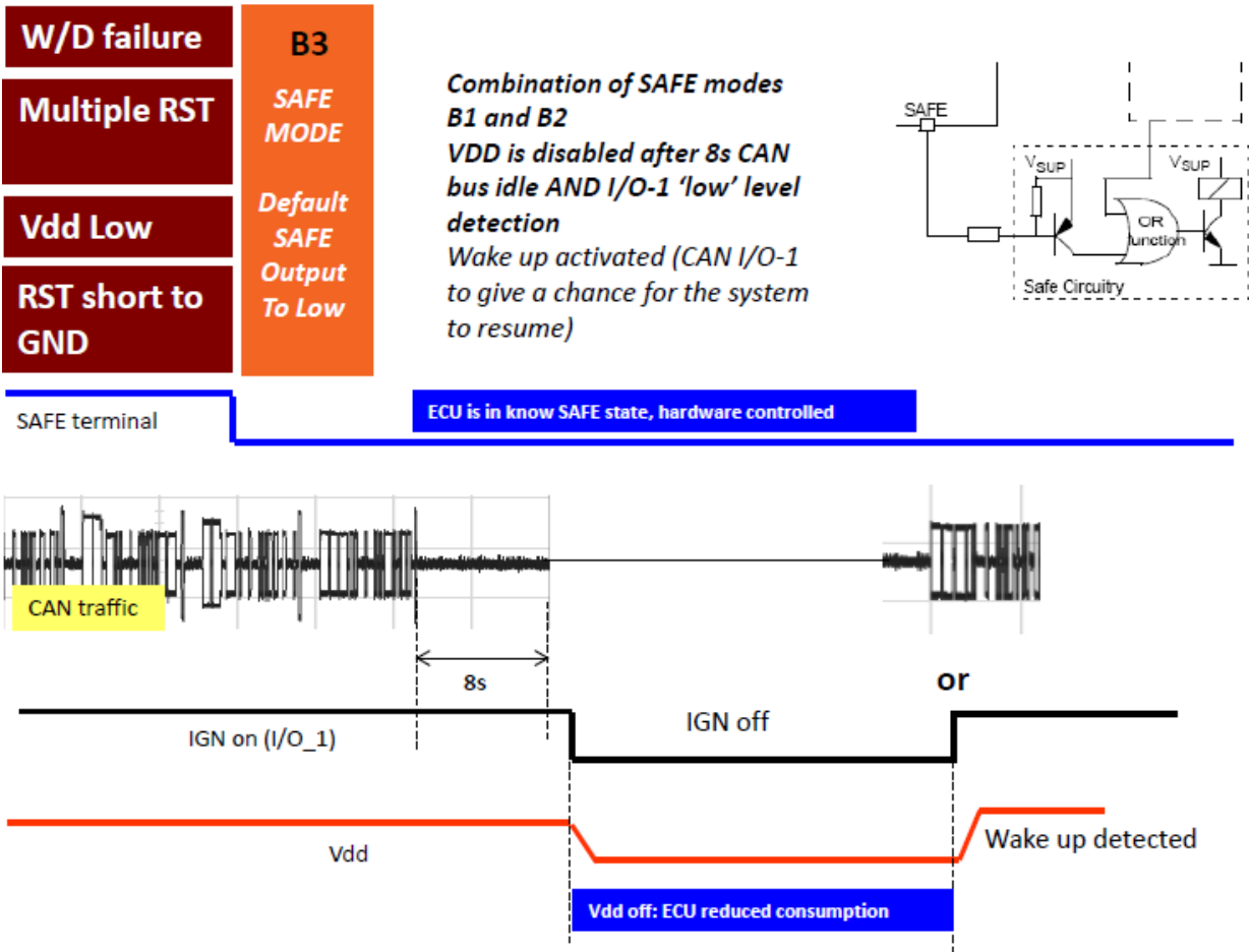
Figure 71. SAFE mode B3
