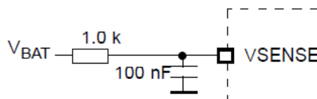
Figure 18. VSENSE typical application schematic
