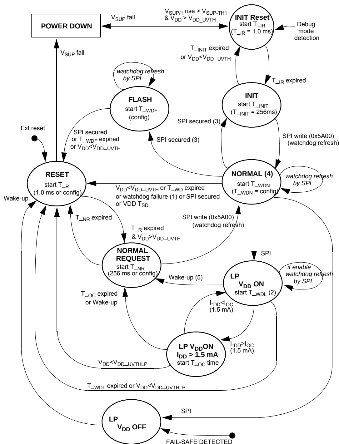
Figure 65. State diagram
