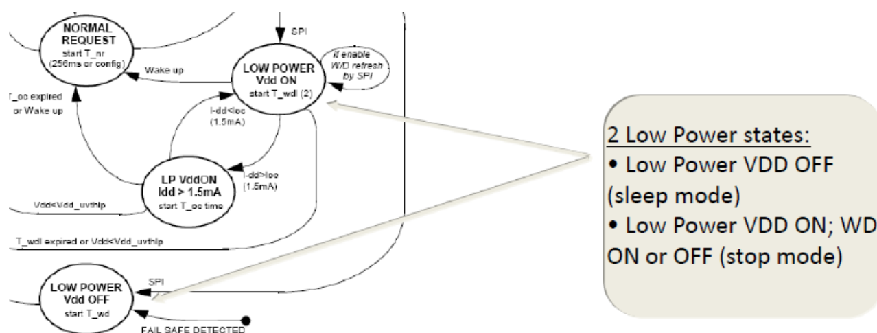
Figure 80. Low power states diagram
