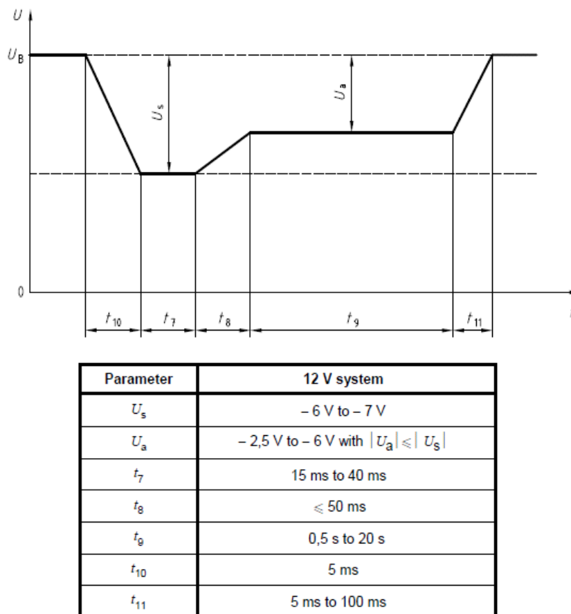
Figure 19. Crank pulse parameters
