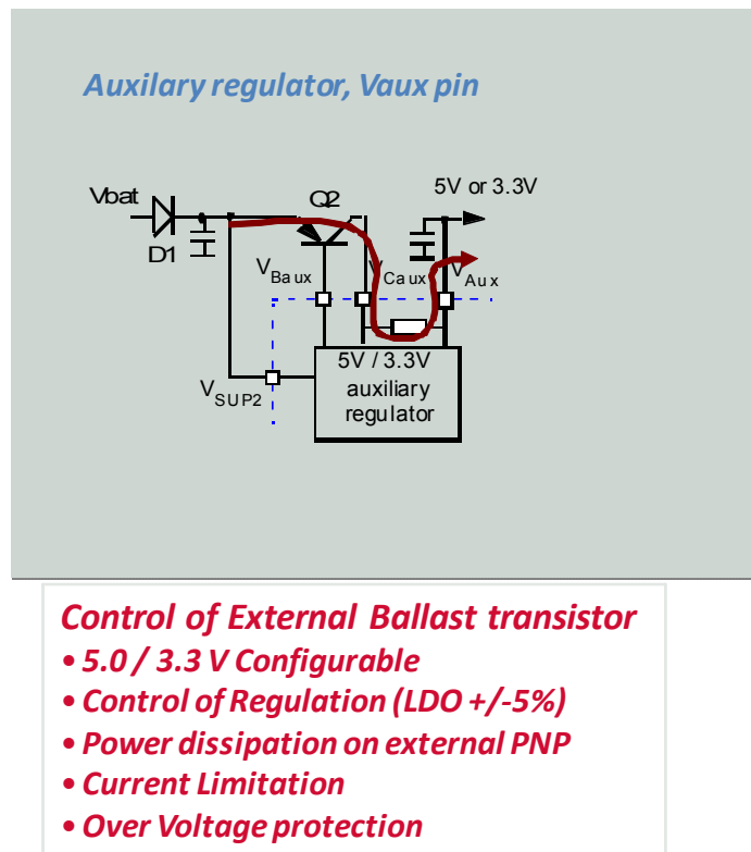
Figure 31. V AUX nominal application characteristics
