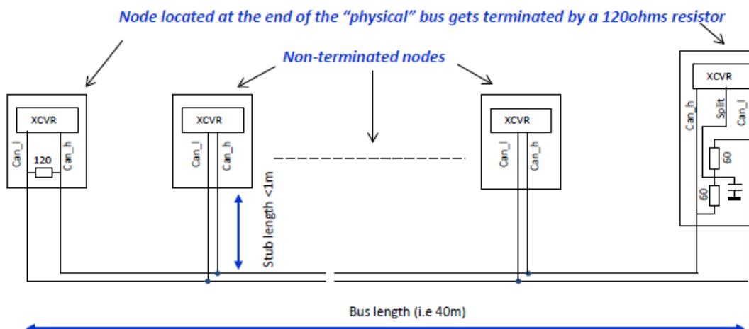
Figure 56. High speed CAN network topology
