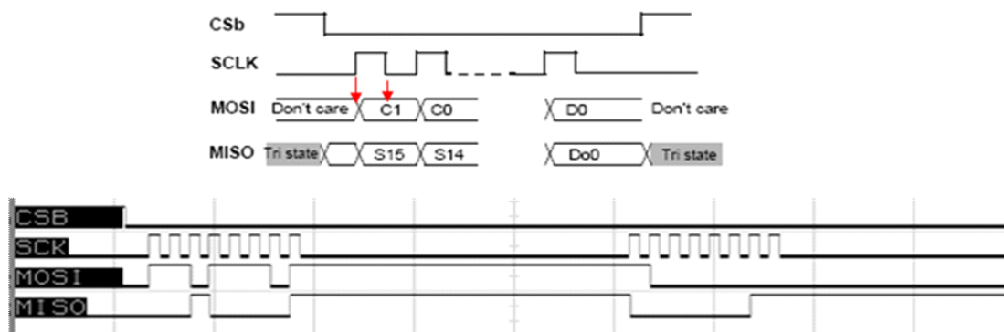
Figure 63. Serial peripheral interface
