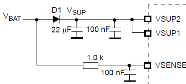
Figure 15. VSUP1 and VSUP2 typical application schematic
