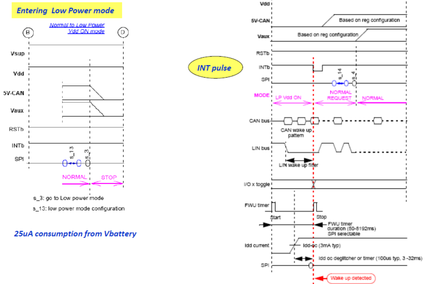
Figure 85. Transitioning into and out of low power VDD on mode
