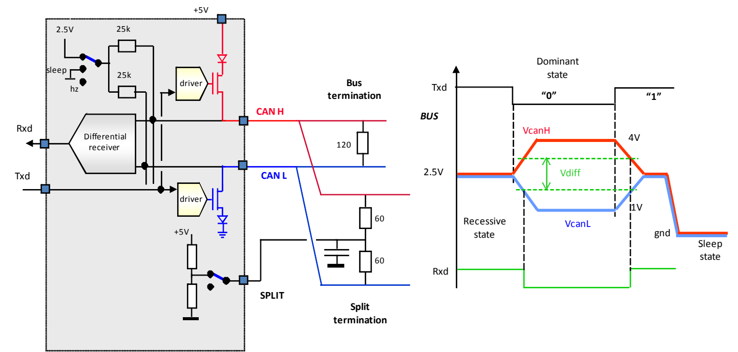
Figure 54. High speed CAN physical interface
