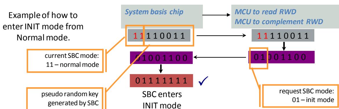
Figure 89. Secured SPI operation
