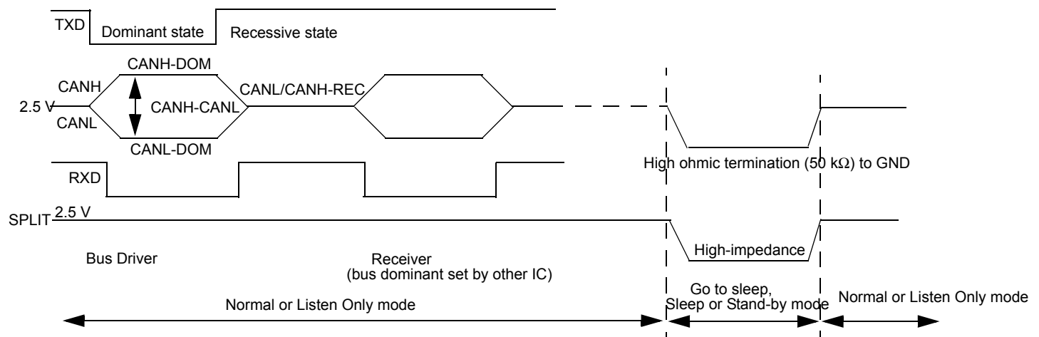
Figure 76. Bus signal in transmit/receive and low power mode
