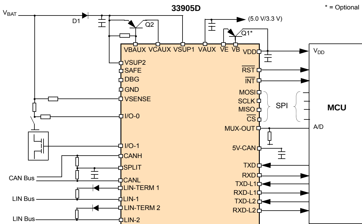
Figure 14. 33905D simplified application diagram
