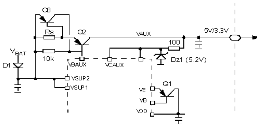
Figure 35. V_{AUX} routed outside module with +20 V protection and external current limit
