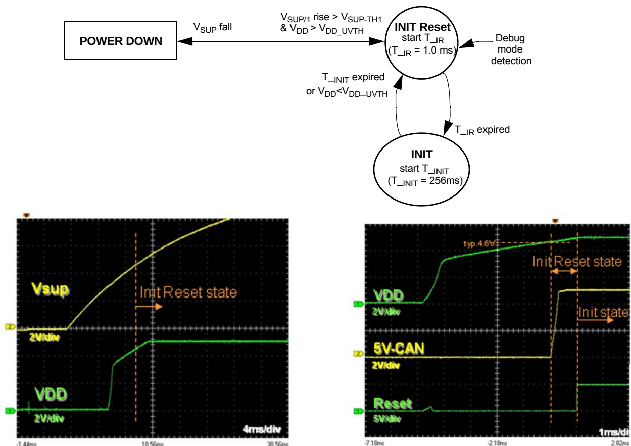
Figure 72. Initialization after power-up
