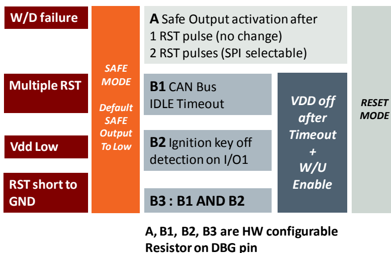
Figure 67. Fail-safe modes
