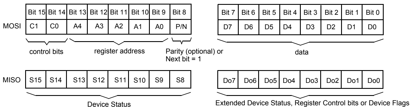
Figure 64. SPI read and write functionality
