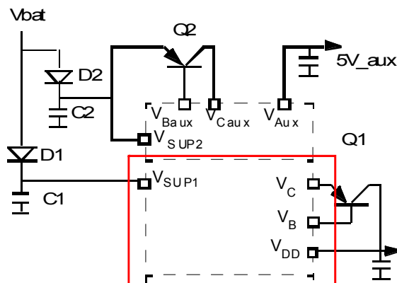
Figure 7. V_{SUP1} and V_{SUP2} Voltage supplies
