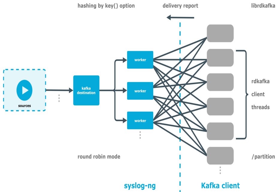
Figure 11: How the C implementation of the kafka destination works with syslog-ng OSE
