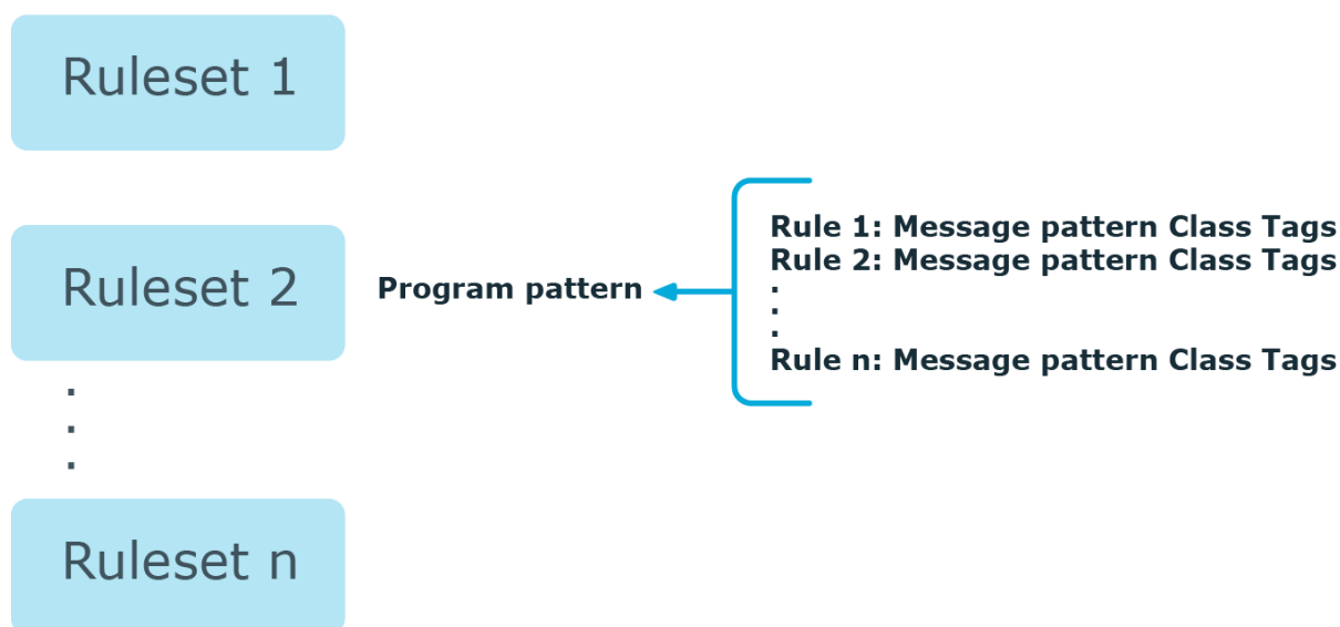
Figure 19: The structure of the pattern database Pattern database
