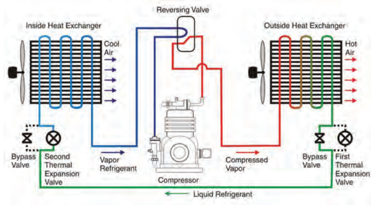
Figure 12.1. Heat Pump in Cooling Mode [2]
