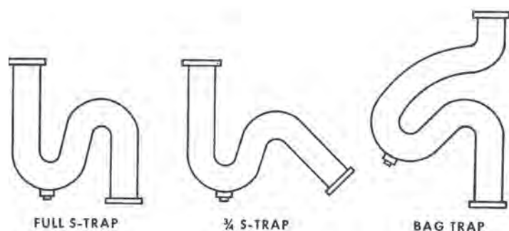
Figure 9.7. Types of S-traps
