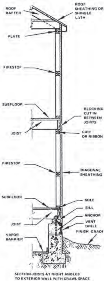
Figure 6.9. Wall Framing [4]
