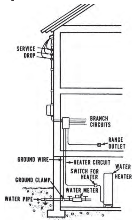
Figure 11.7. Typical Service Entrance [2]
