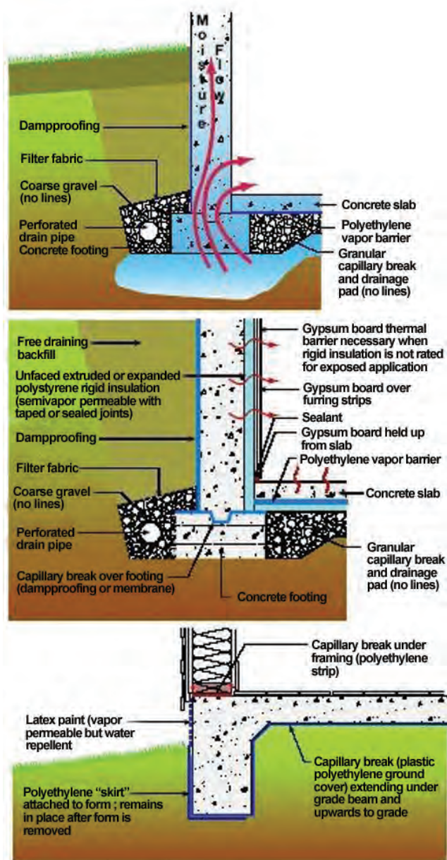
Figure 6.3. Foundation [3]
