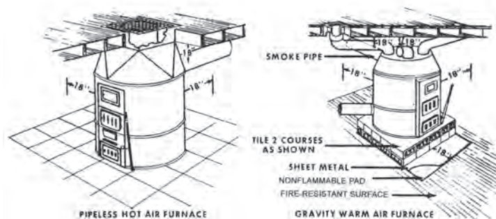
Figure 12.4. Minimum Clearance for Pipeless Hot Air and Gravity Warm Air Furnace [4]
