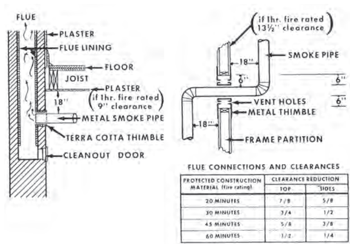
Figure 12.17. Wall and Ceiling Clearance Reduction [4]
