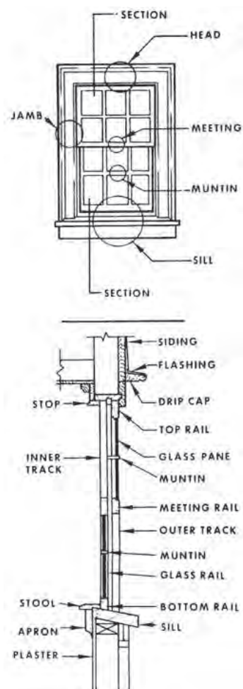
Figure 6.8. Window Details [3]
