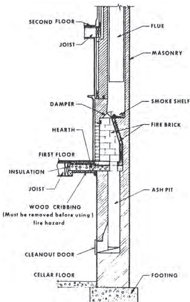
Figure 12.23. Fireplace Construction [4]
