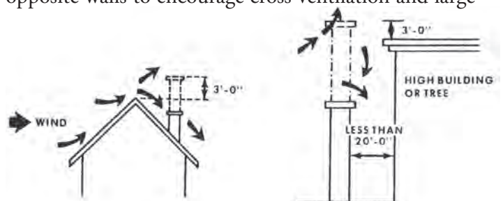
Figure 12.18. Draft Relation to Height of Chimney [4]
