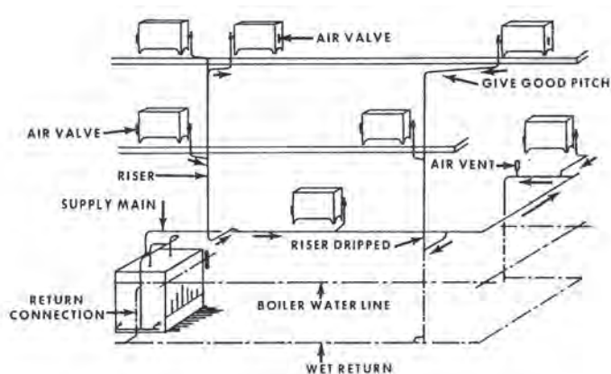
Figure 12.10. Typical Gravity One-pipe Heating System [4]
