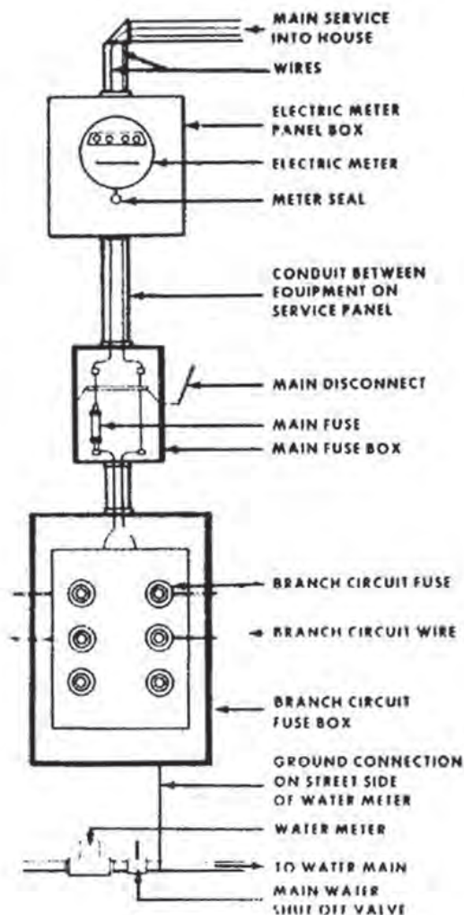
Figure 11.10. Three-wire Service [2]
