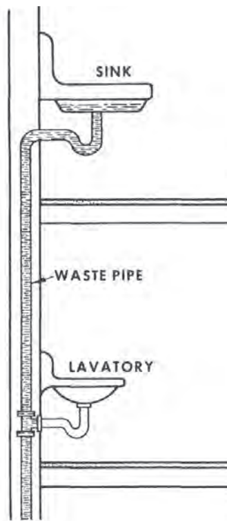
Figure 9.9. Loss of Trap Seal in Lavatory Sink [1]
