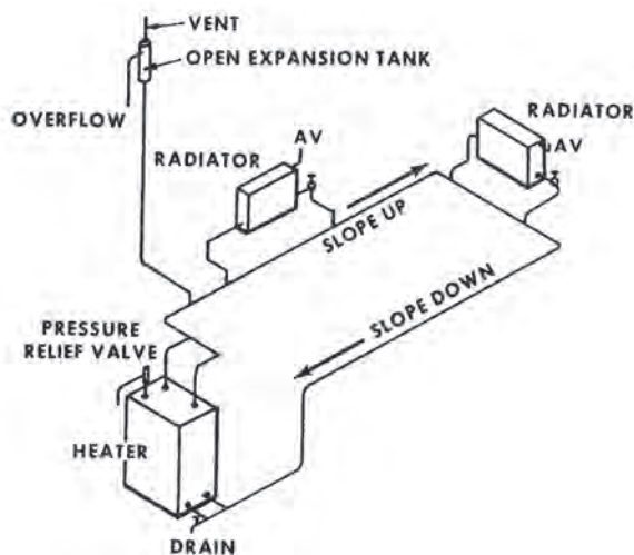
Figure 12.11. One-pipe Gravity Water Heating System [4]
