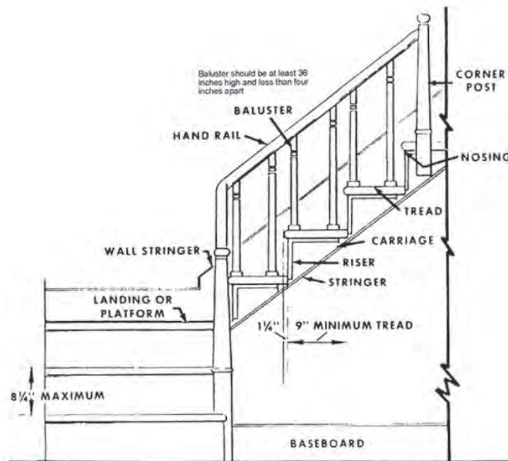
Figure 6.5. Interior Stairway [4]
