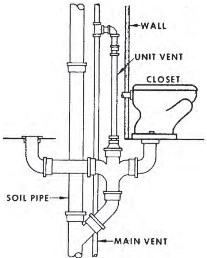
Figure 9.10. Back-to-back Venting [Toilet]
