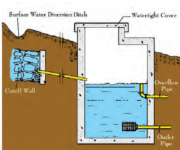
Figure 8.10. Spring Box [5]
