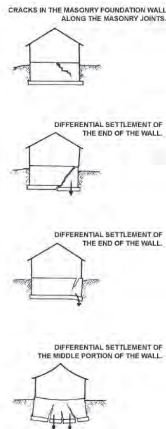
Figure 6.4. Foundation Cracks [4]
