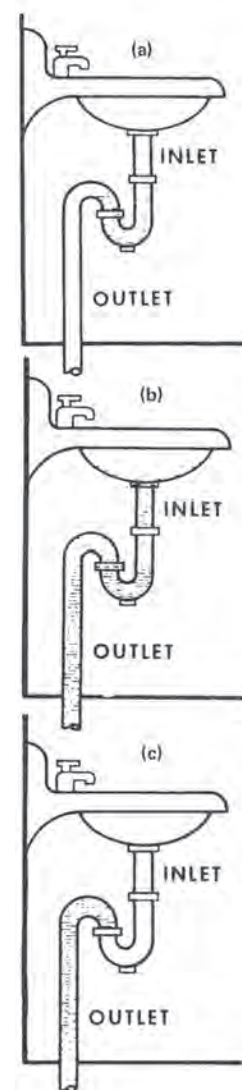
Figure 9.8. Trap Seal: [a] Seal Intact; [b] Fixture Draining; [c] Loss of Gas Seal [1]
