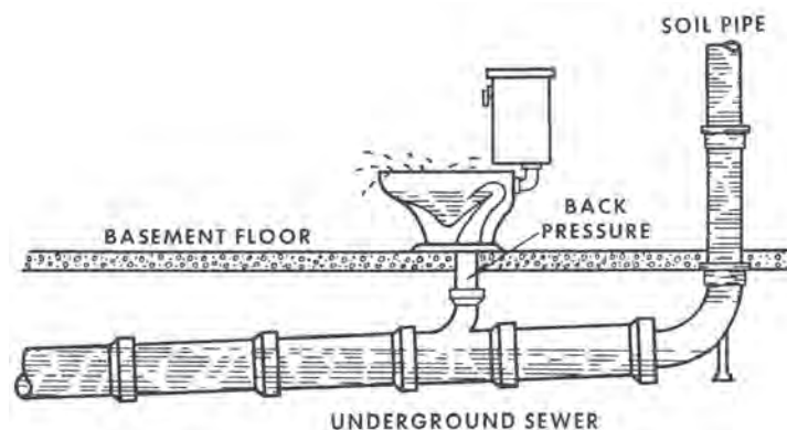
Figure 9.14. Toilet Venting
