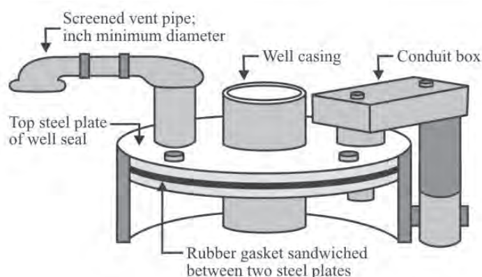
Figure 8.3. Well Seal
