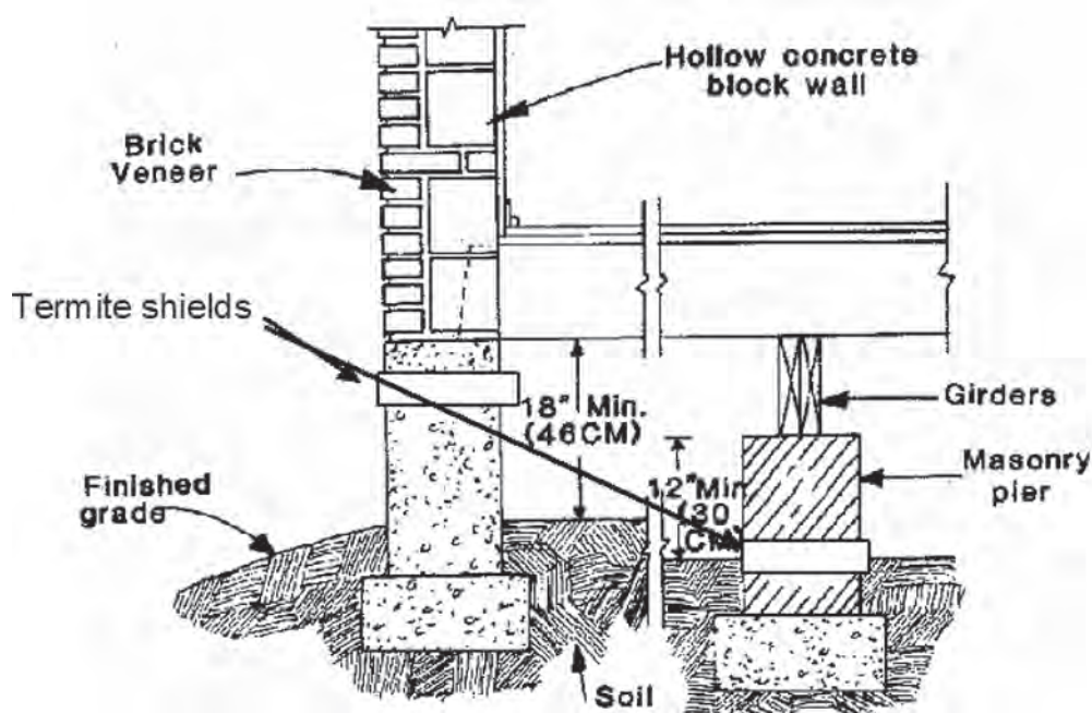
Figure 4.24. Construction Techniques That Discourage Termite Attacks: Thin Metal Termite Shield Should Extend 2 Inches Beyond Foundation and 2 Inches Down [2]
