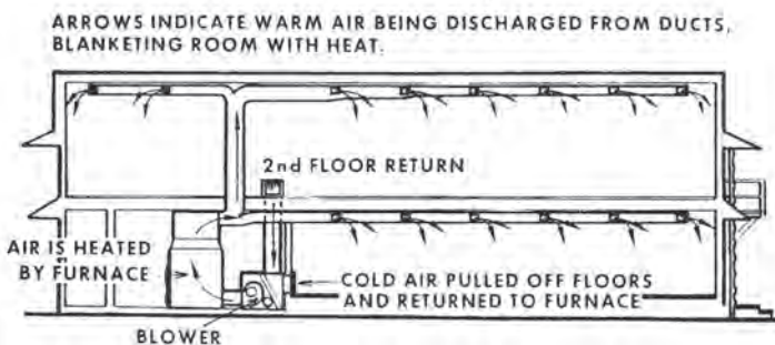
Figure 12.14. Cross-sectional View of Building Showing Forced Warm-air Heating System [4]
