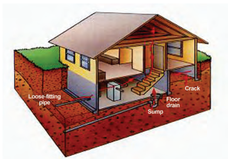
Figure 5.6. Radon Entry [30]
