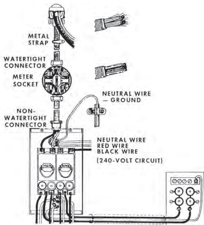
Figure 11.3. Armored Cable Service Entrance [2]
