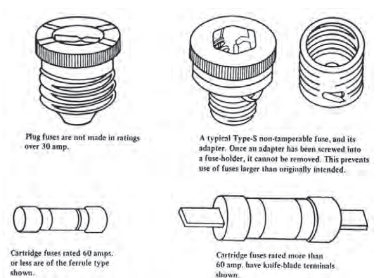
Figure 11.18. Types of Fuses
