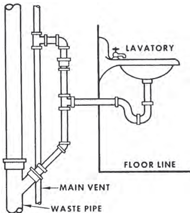
Figure 9.12. Wall-hung Fixtures
