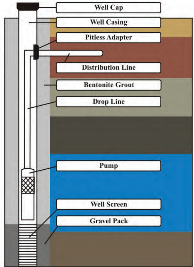
Figure 8.6. Drilled Well [4]
