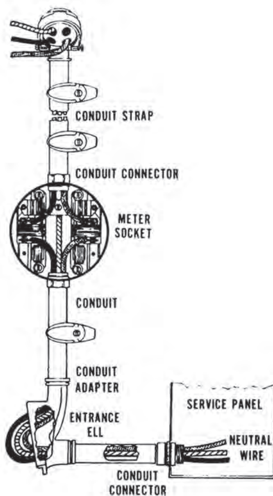
Figure 11.5. Thin-wall Conduit [2]
