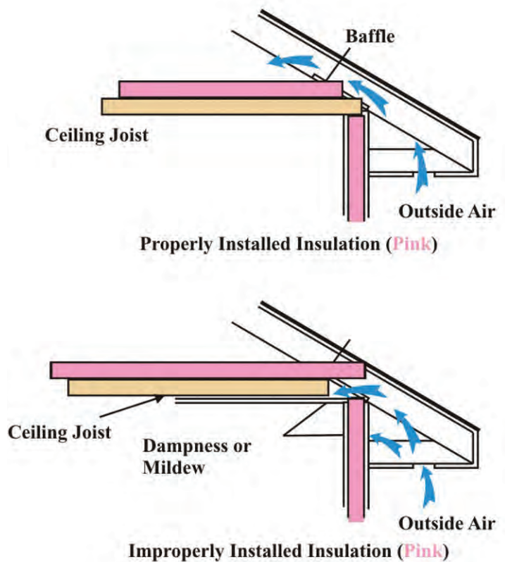
Figure 7.4. Attic ventilation
