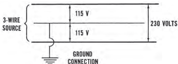
Figure 11.9. Grounding [2]
