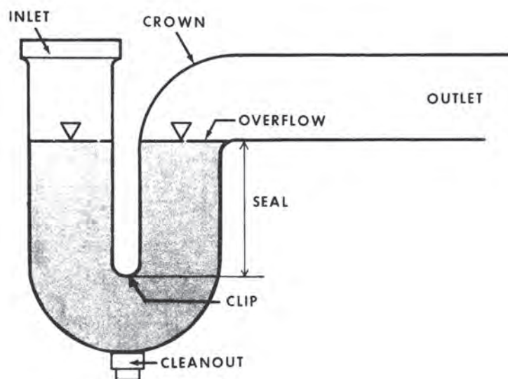
Figure 9.6. P-trap [1]
