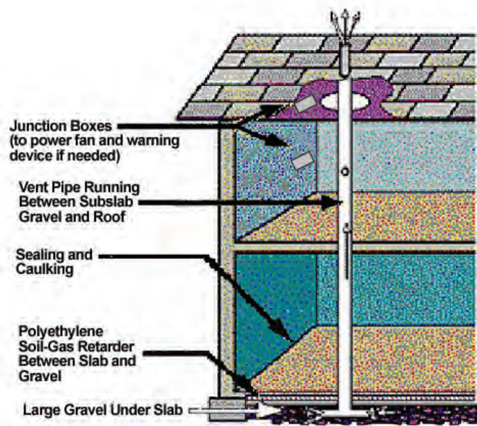
Figure 5.8. Radon-resistant Construction [50]
