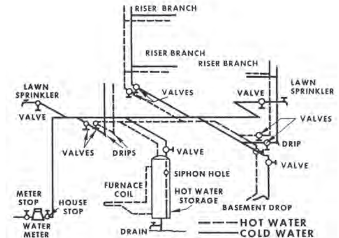
Figure 9.1. Typical Home Water System [1]
