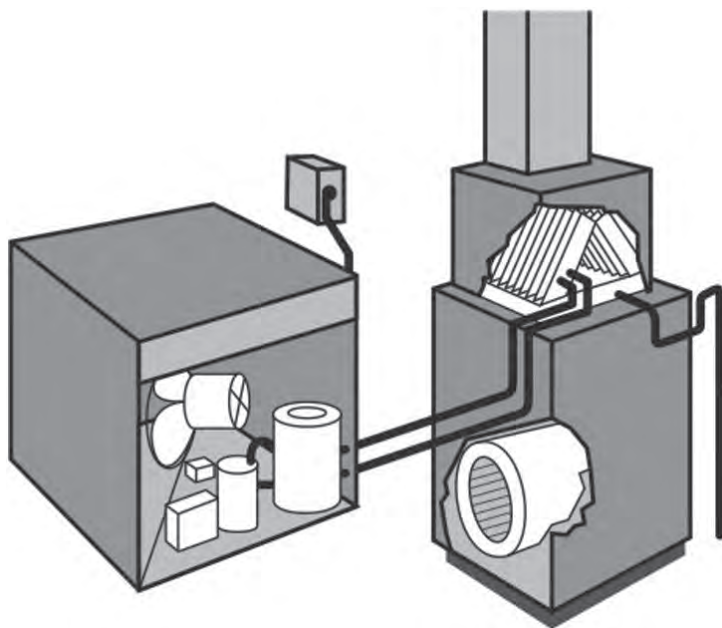
Figure 12.20. Split-system Air Conditioner
