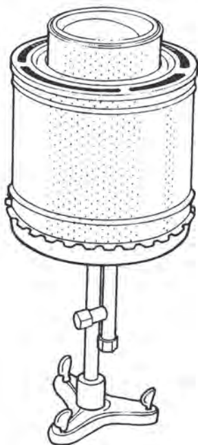
Figure 12.15. Perforated-sleeve Burner
