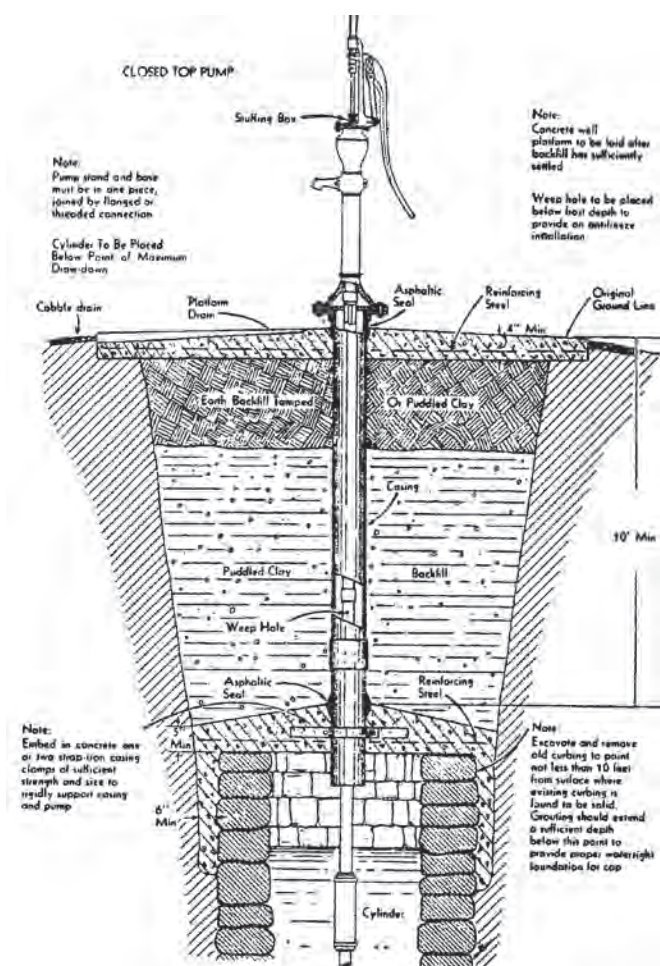
Figure 8.4. Converted Dug Well [1]
