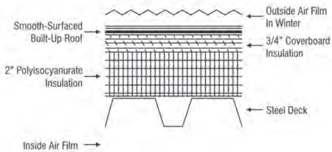
Figure 13.1. Roof Components [2]
