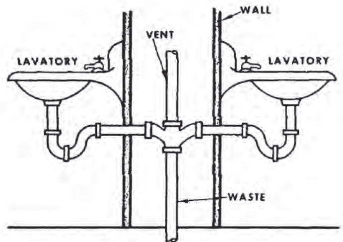
Figure 9.11. Back-to-back Venting [Sink]
