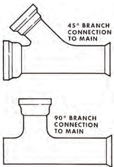
Figure 9.5. Branch Connections
