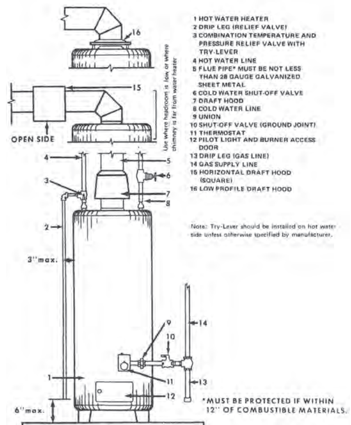
Figure 9.3. Gas Water Heater [1]
