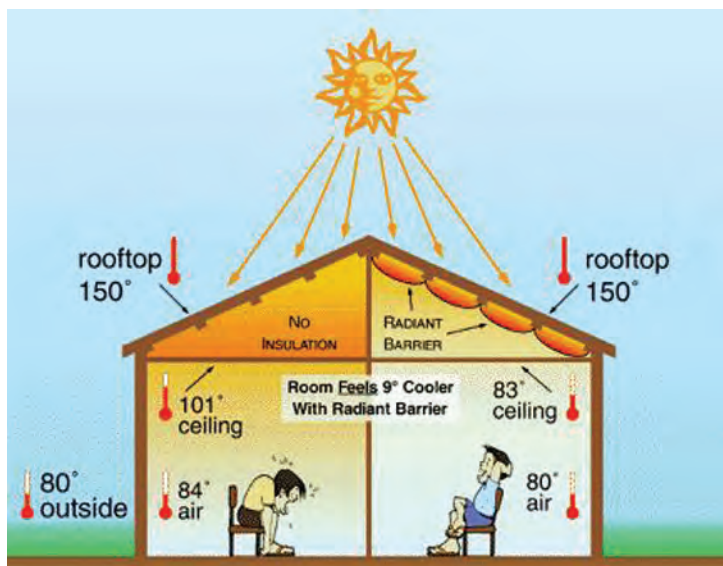
Figure 13.2. Potential Effects of Radiant Barriers [3]
