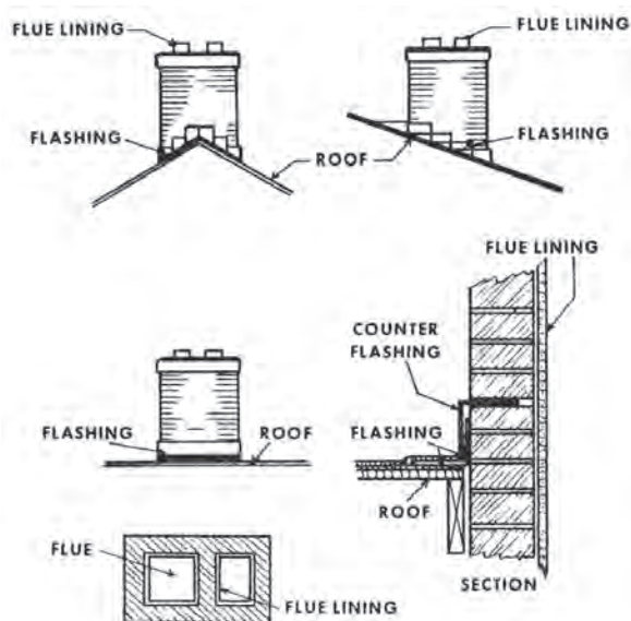
Figure 12.22. Chimney Plan [4]
