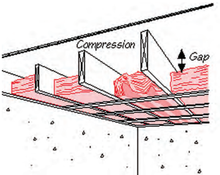
Figure 13.3. Common Floor Insulation Flaws [4.] Two common flaws in floor insulation are gaps above the batt and compression of the batt in the cavity.
