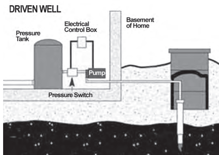
Figure 8.2. Cross Section of a Driven Well
