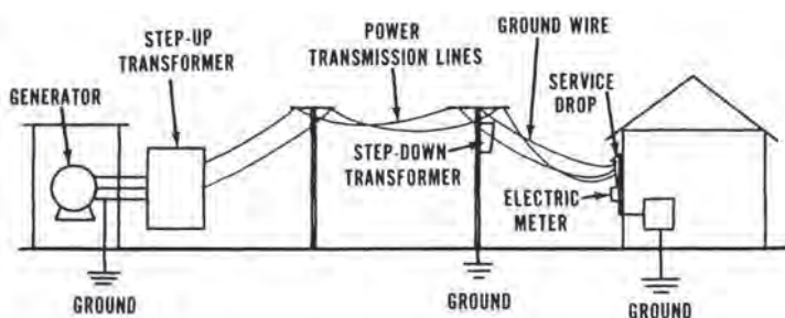
Figure 11.1. Utility Overview [2]
