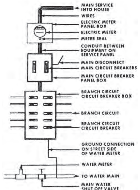
Figure 11.11. Two-wire Service [2]
