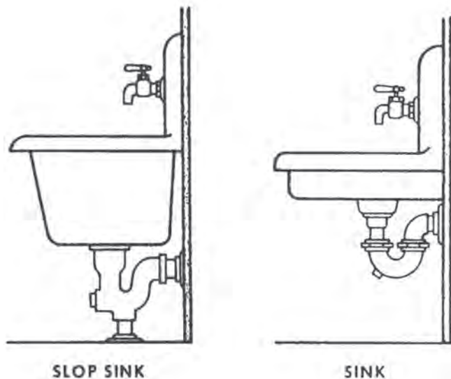
Figure 9.15. Janitor's Sink
