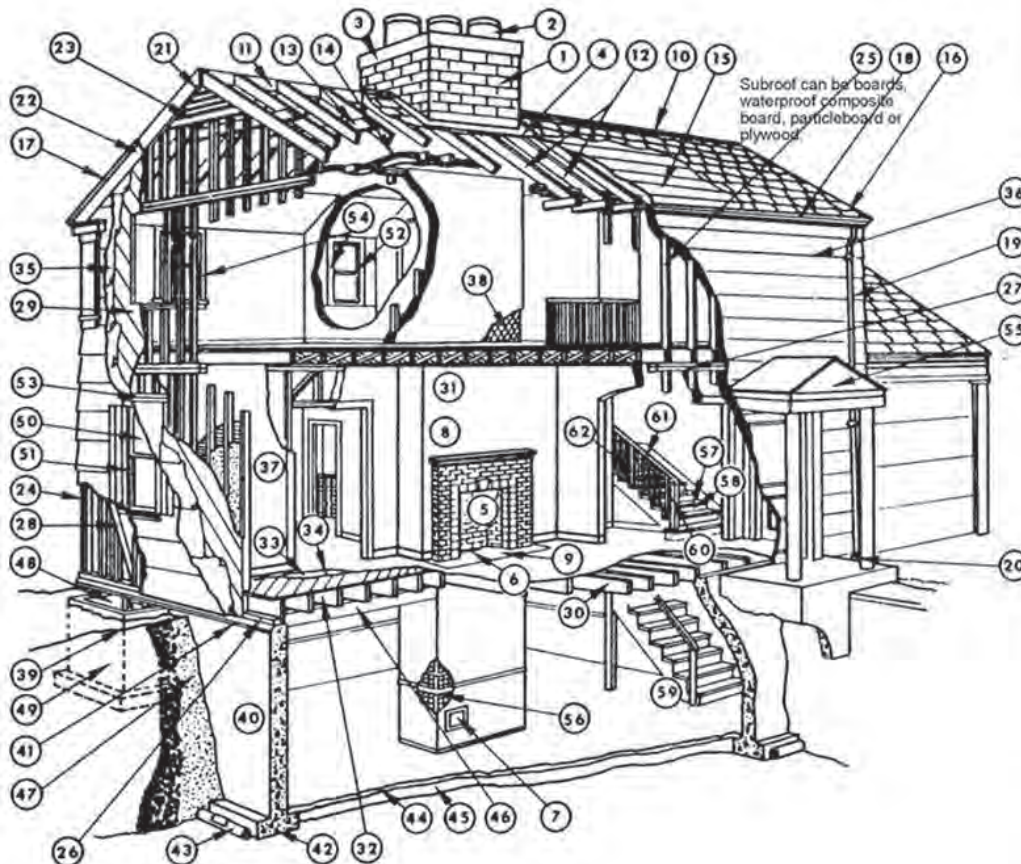
Figure 6.2. Housing Structure and Terminology, Typical House Built Between 1950 and 1980 [2]
