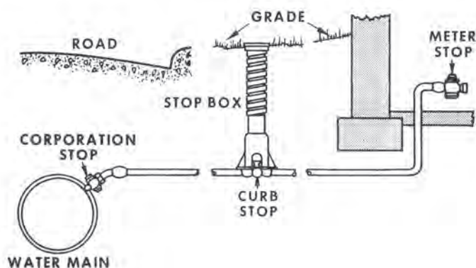
Figure 9.2. House Service Installation [1]
