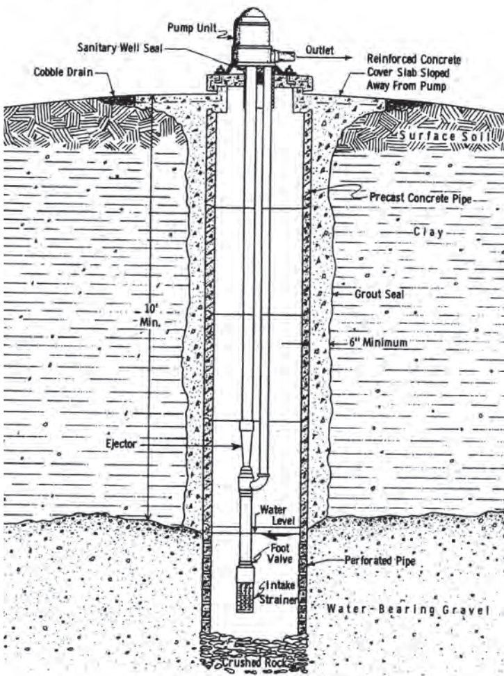
Figure 8.5. Recapped and Sealed Dug Well [1]
