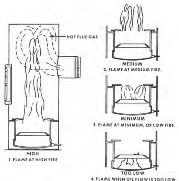
Figure 12.16. Condition of Burner Flame with Different Rates of Fuel Flow [4]
