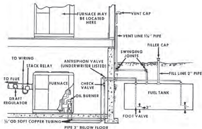
Figure 12.3. Piping Hookup for Buried Outside Tank [4]
