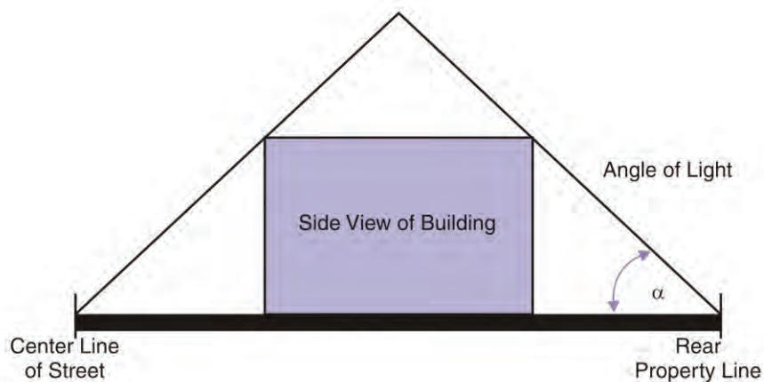
Figure 3.2. Example of an Angle of Light Obstruction
