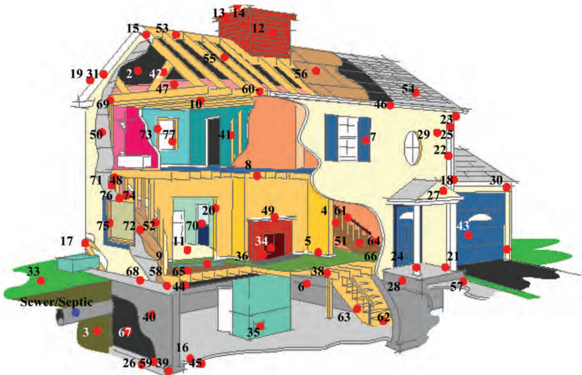
Figure 6.1. Housing Structure Terminology, Typical House Being Built Today [1]
