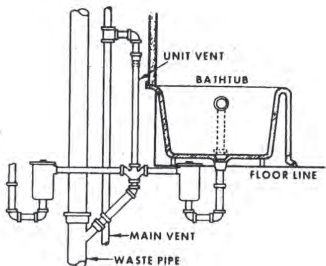
Figure 9.13. Unit Vent Used in Bathtub Installation
