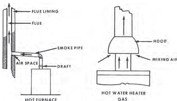
Figure 12.19. Location and Operation of Typical Backdraft Diverter [4]
