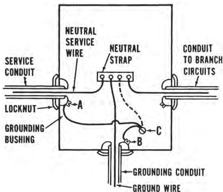
Figure 11.8. Grounding Scheme [2]
