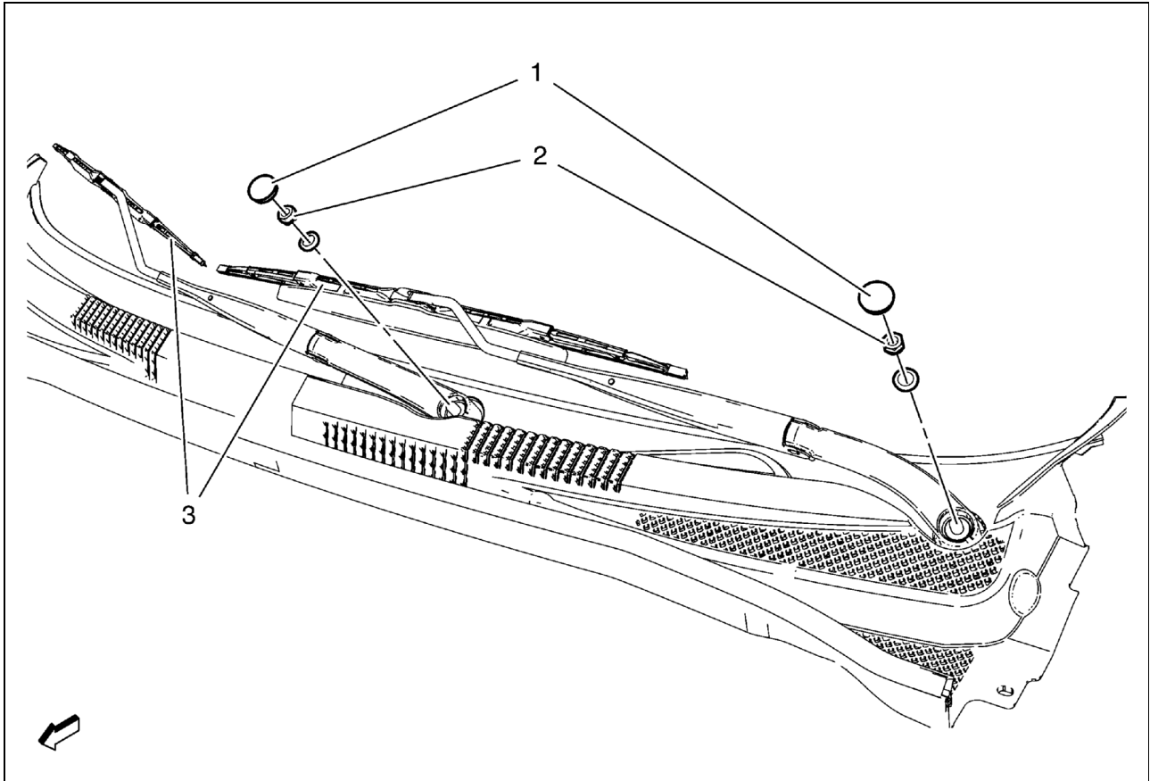
Fig 1: Windshield Wiper Arm Components
