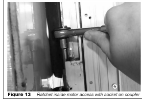
Figure 13 Ratchet inside motor access with socket on coupler
