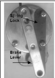
Brake lever released
