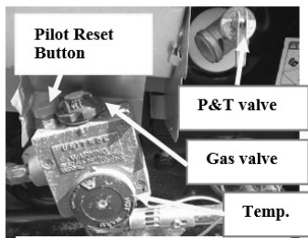
Water Heater pilot ignition
