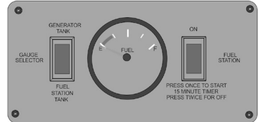
Dual Tank Fuel Gauge & Selector Switch
