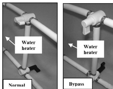
Two Valve Water Heater Bypass
