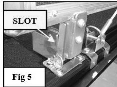
Side Rail & Bracket
