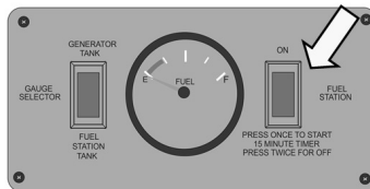
Typical Fuel Pump Switch Locations on the Command Center
