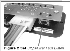
Figure 2 Set Stops/Clear Fault Button
