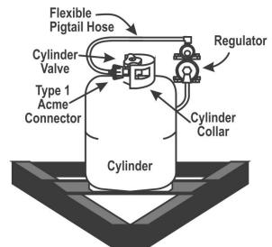
Single Cylinder
