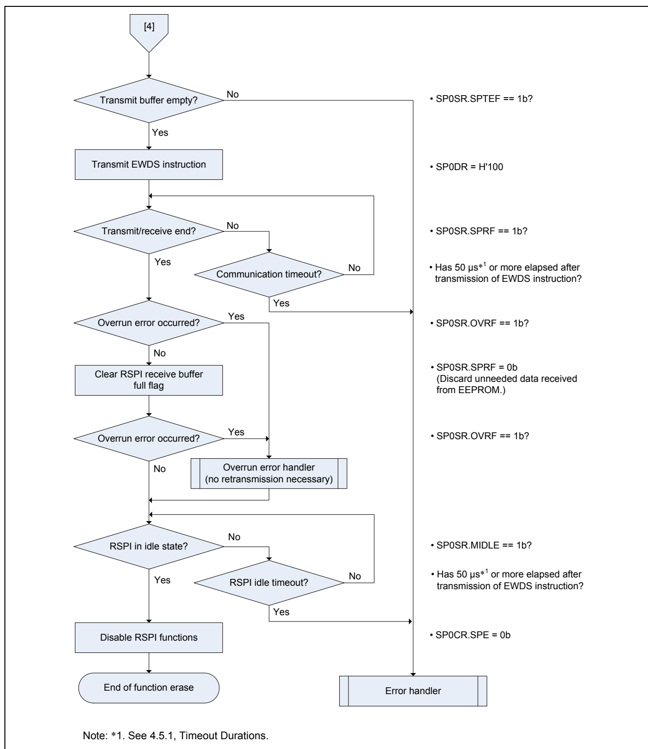
Figure 4.10 Function erase (4/4)
