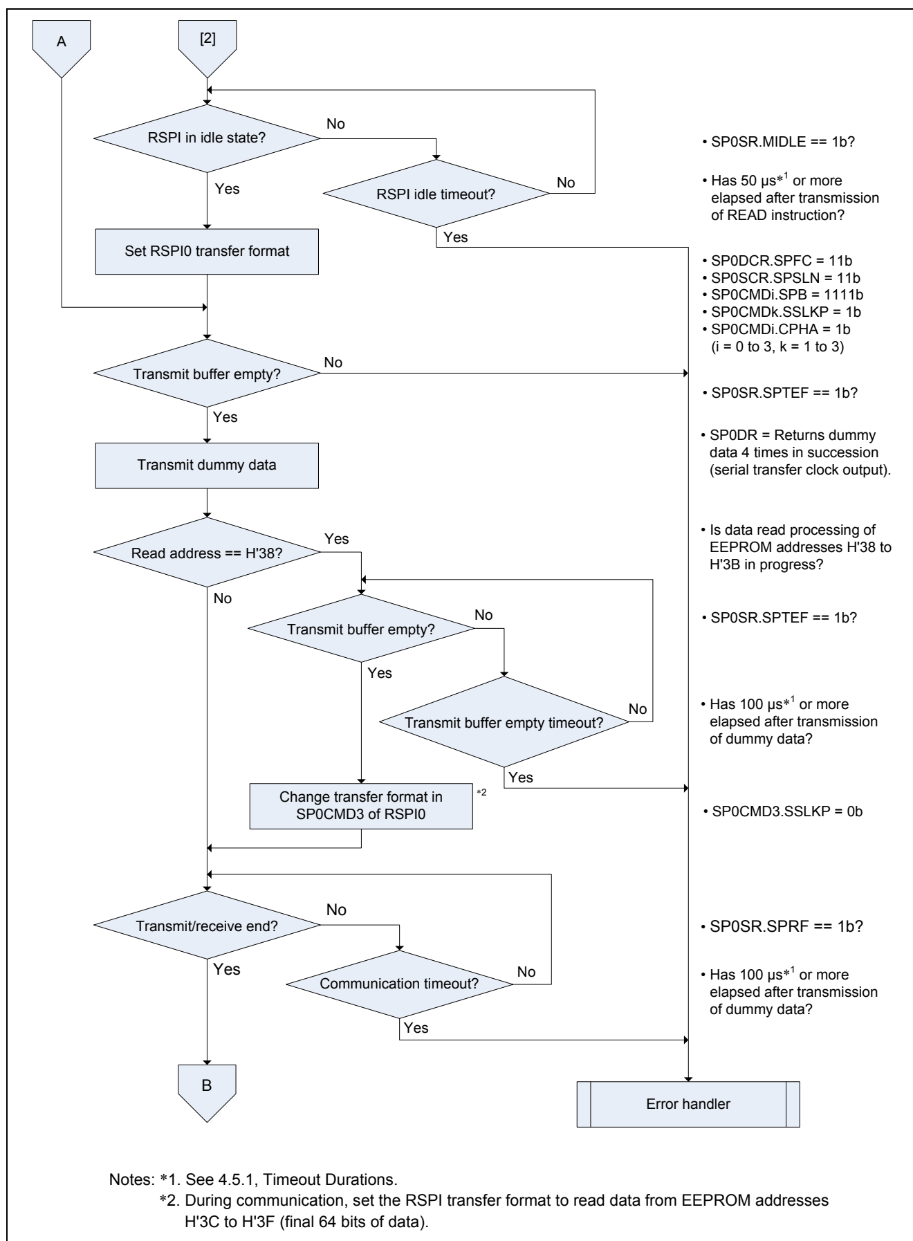
Figure 4.4 Function read (2/3)
