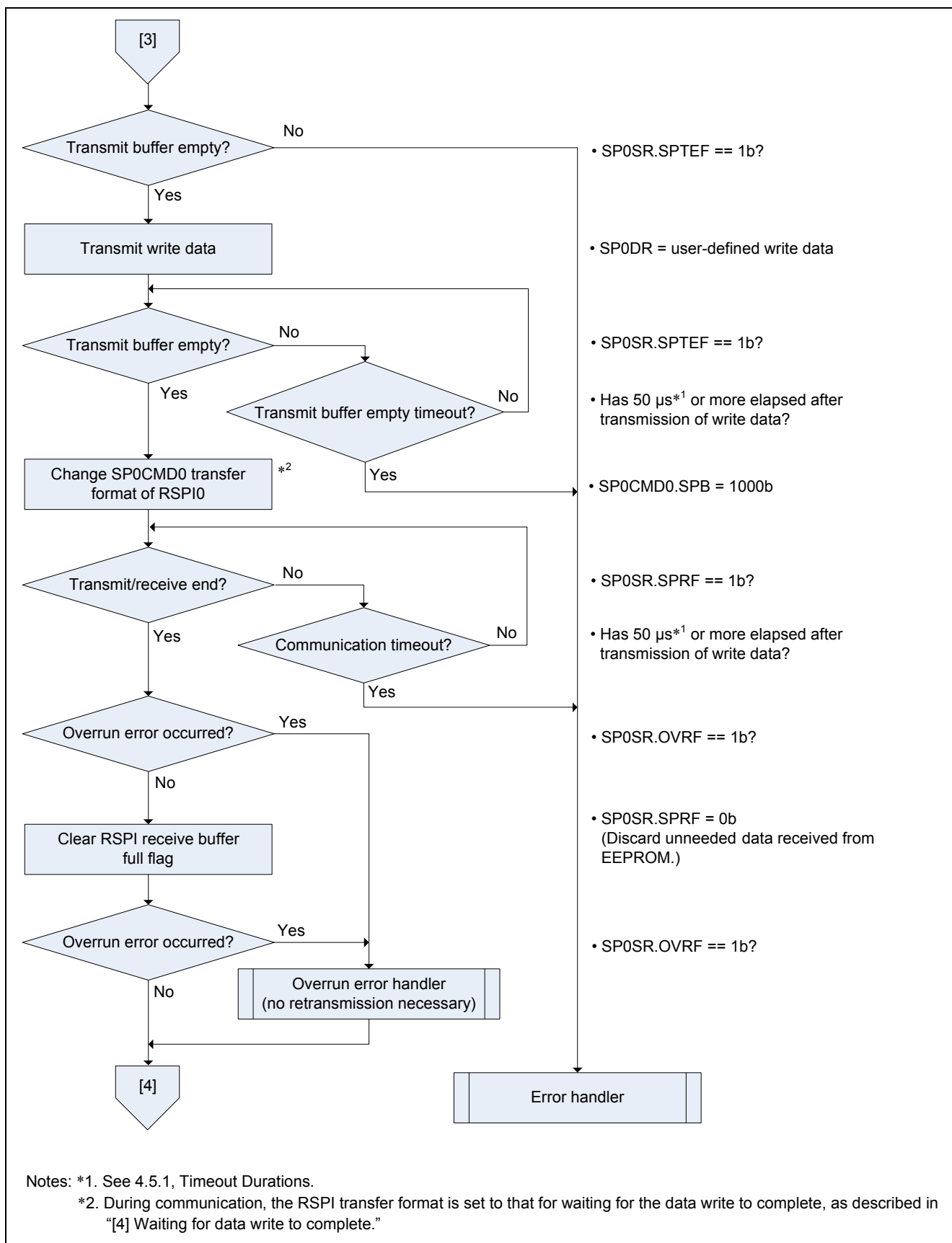
Figure 4.14 Function write (3/6)
