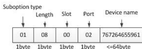
Figure 4- 16 Option82-remote-id
