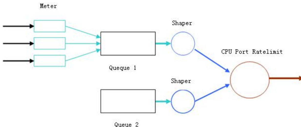
Figure 13-3 Level Rate Limit of the CPP
