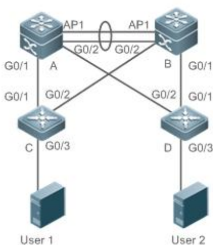
Figure 7- 1 MSTP+VRRP Dual-Core Topology
