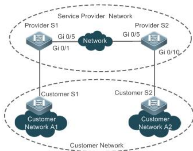
Figure 7- 2 BPDU Tunnel Topology
