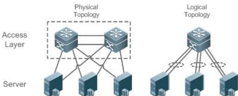
Figure 7- 6 Access layer stacking
