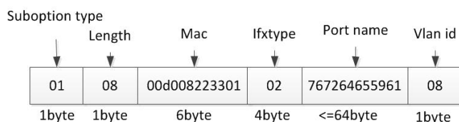
Figure 4- 16 Option82-remote-id
