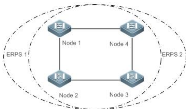
Figure 11- 4 Single-Ring Load Balancing
