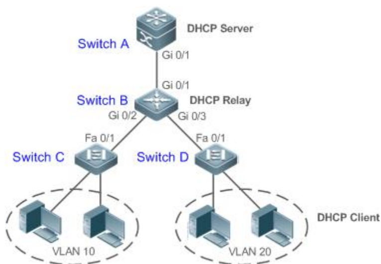
Figure 4- 5 DHCP Relay
