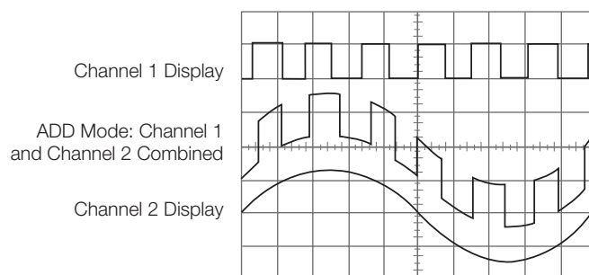
Figure 39. Adding channels.
