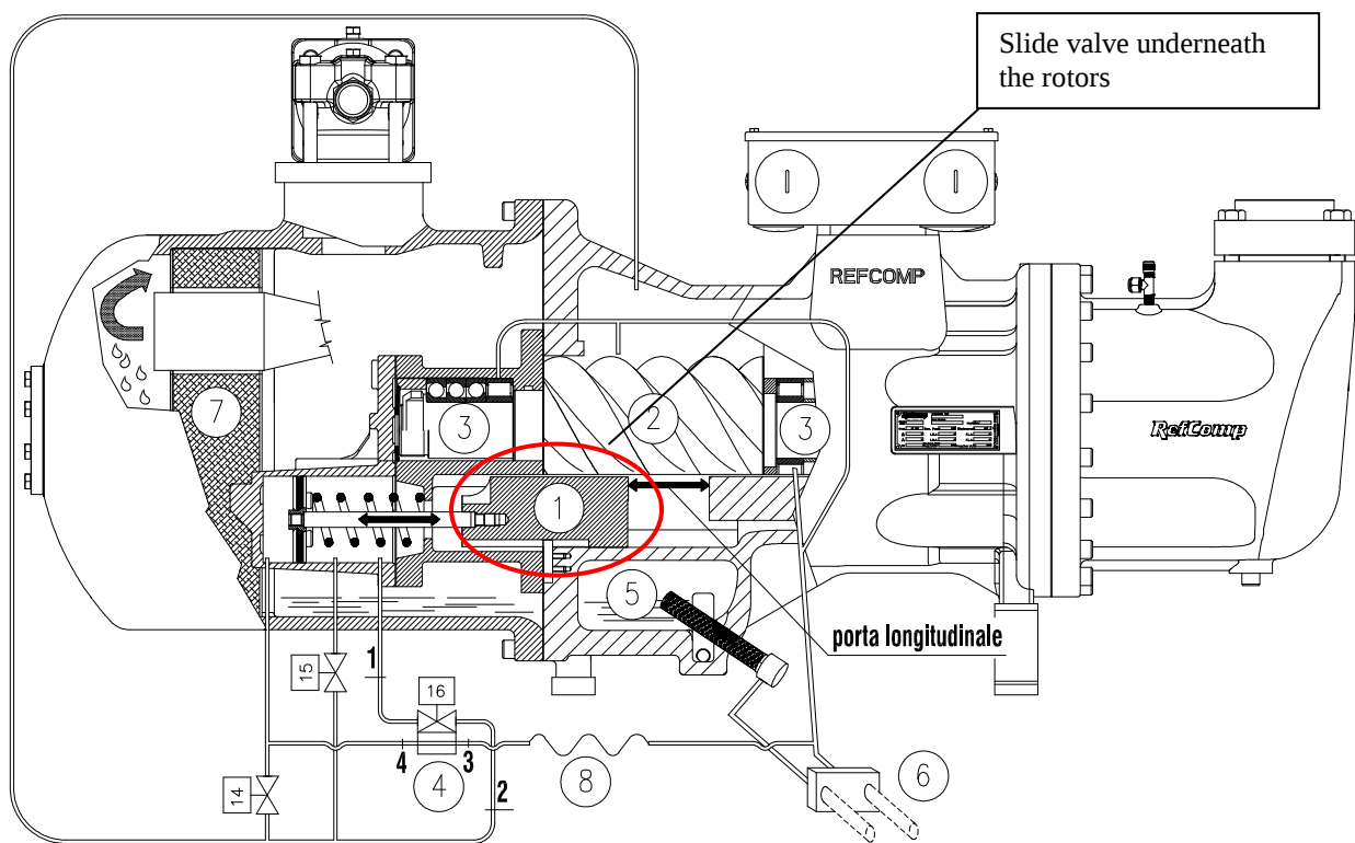
Picture 2-A: diagram of the internal oil circuit for lubrication and operation of the slide valve;
