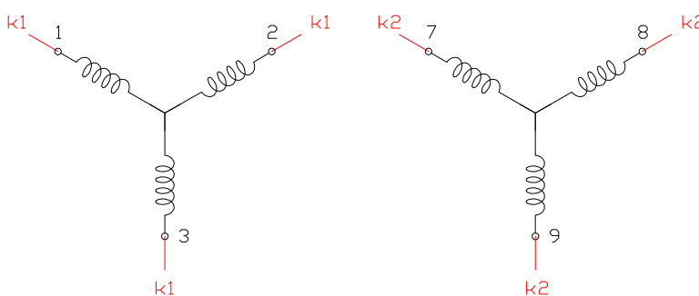
STAR CONFIGURATION: Y-YY
