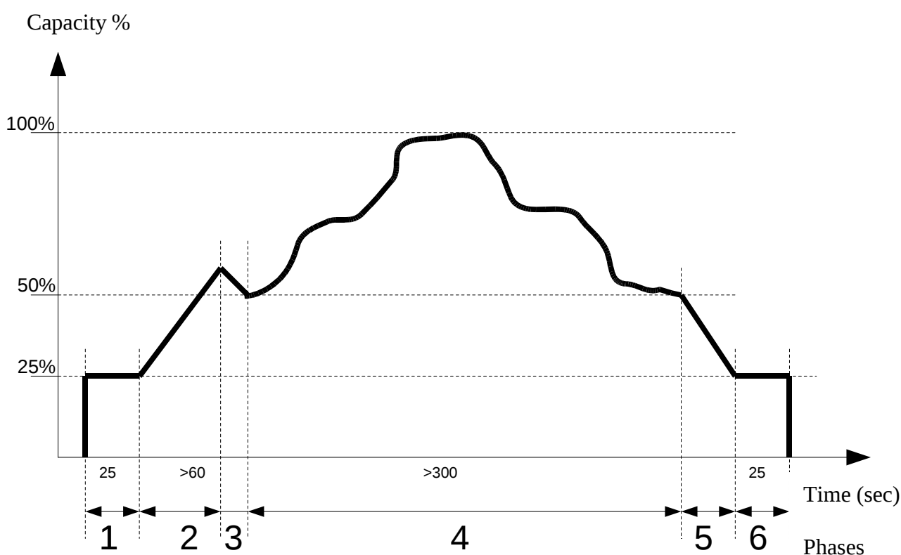
Figura 3-P Logic control of solenoid valves for stepless configuration
