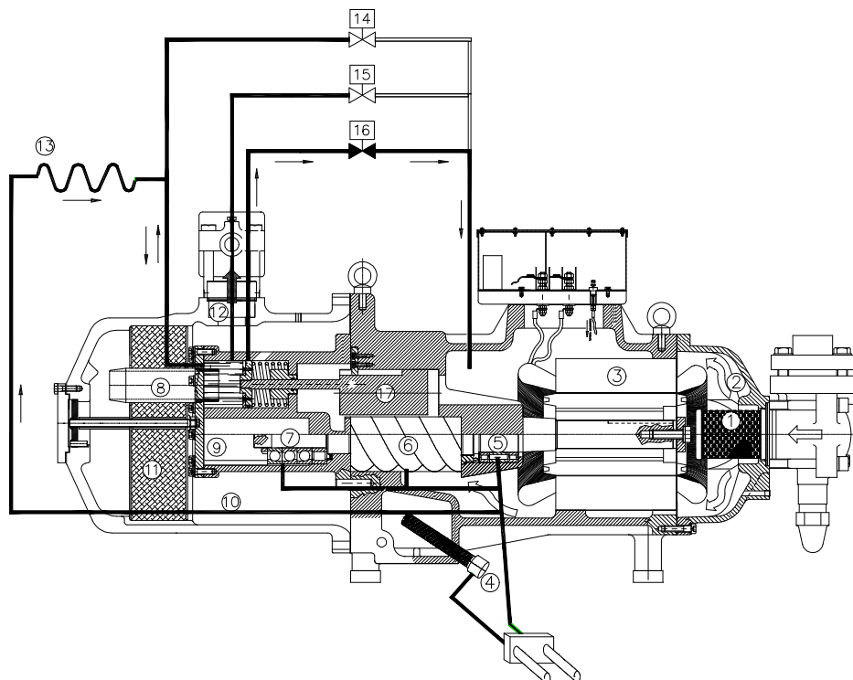
Picture 3-G: capacity control at 75% step: models 113/133/163/183/213/253/303/353/413/463/503/553/603;
