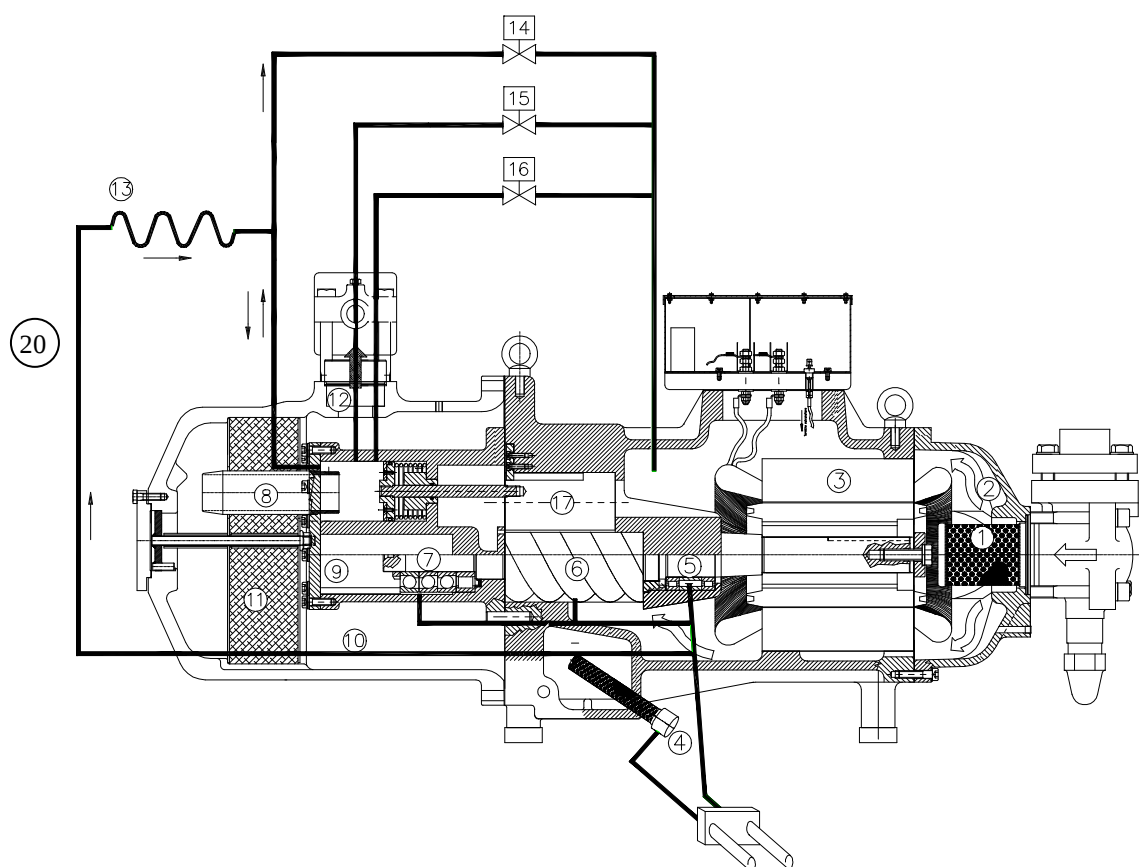
Picture 3-A: step capacity control oil circuit for the models: SRC-S-113/133/163/183/213/253/303/353/413/463/503/553/603; 14, 15, 16: capacity control solenoid valves; 17: capacity control slide valve and operation piston; 13: capillary tube (external to the compressor);
