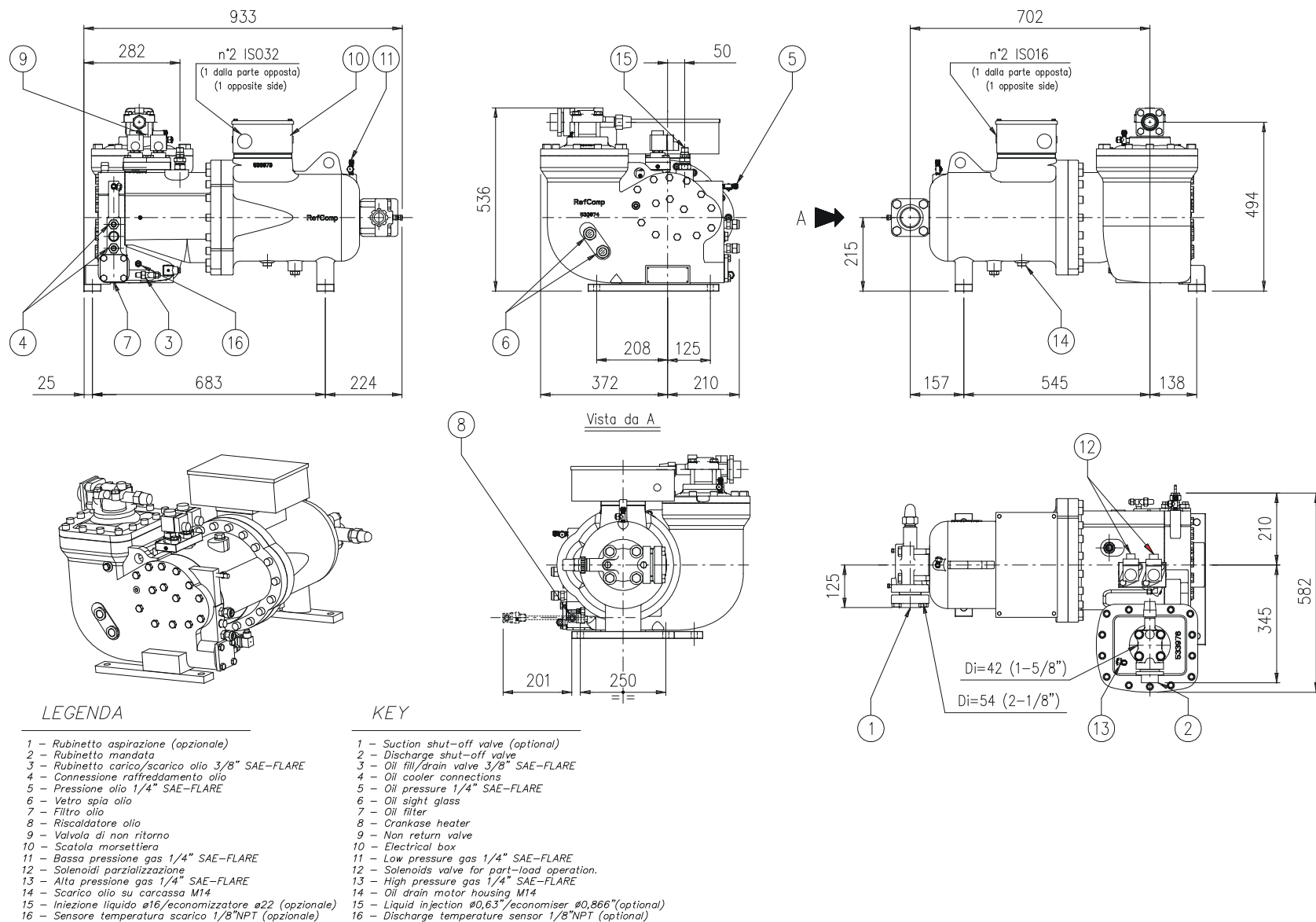
Picture 8-J: dimensional drawing of the models: SRC-XS-40/50/60 (drawing code: MSI042 r.01);
