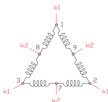
DELTA CONFIGURATION: \Delta - \Delta\Delta
