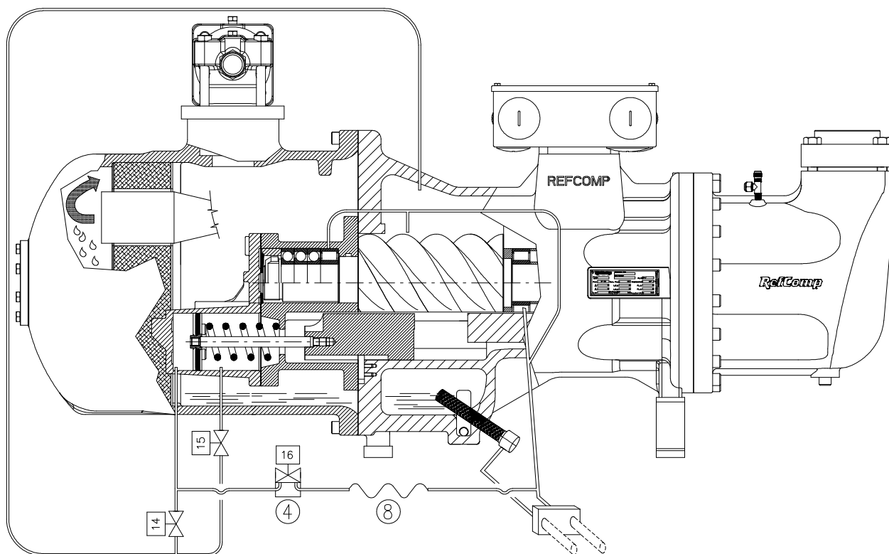
Picture 3-O: infinite capacity control oil circuit (step less configuration): models SRC-S-255/285/305/755/785/885/985;
