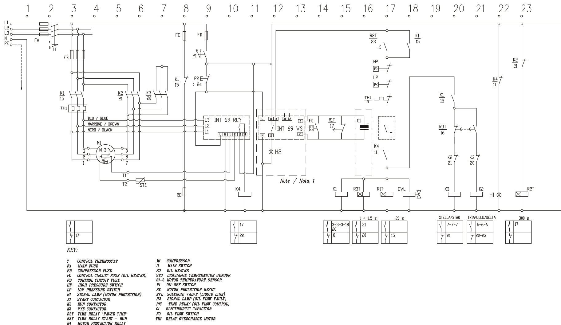
Picture 4-Z: wiring diagram for the connection of the flow switch; electric motor with star-delta configuration YΔ (MCE008$2);
