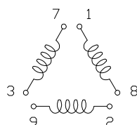
MOTOR WINDING
