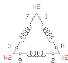
DELTA CONFIGURATION
