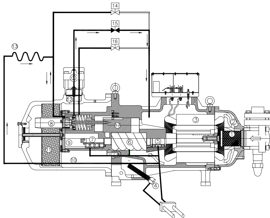
Picture 3-E: capacity control at 50% step: models 113/133/163/183/213/253/303/353/413/463/503/553/603;
