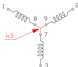
STAR CONFIGURATION
