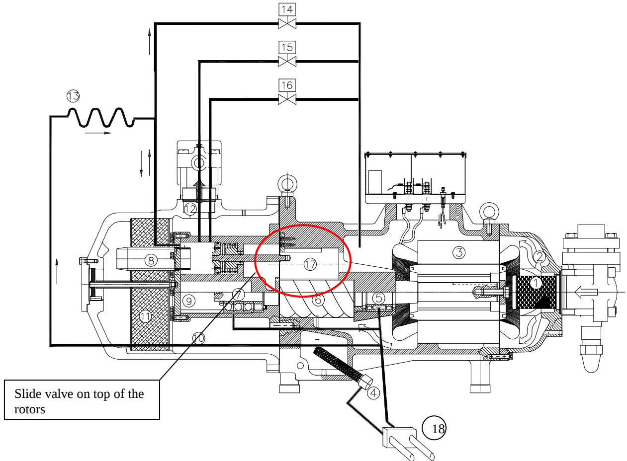
Picture 2-B: diagram of the internal oil circuit for lubrication and operation of the slide valve;
