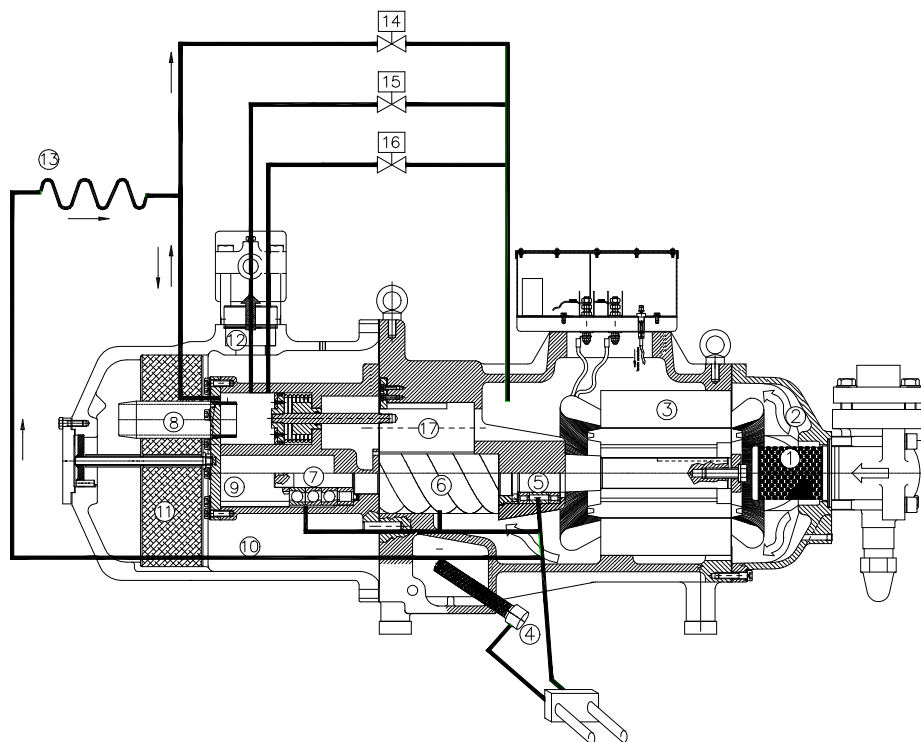
Picture 3-I: capacity control at 100% step: models 113/133/163/183/213/253/303/353/413/463/503/553/603;
