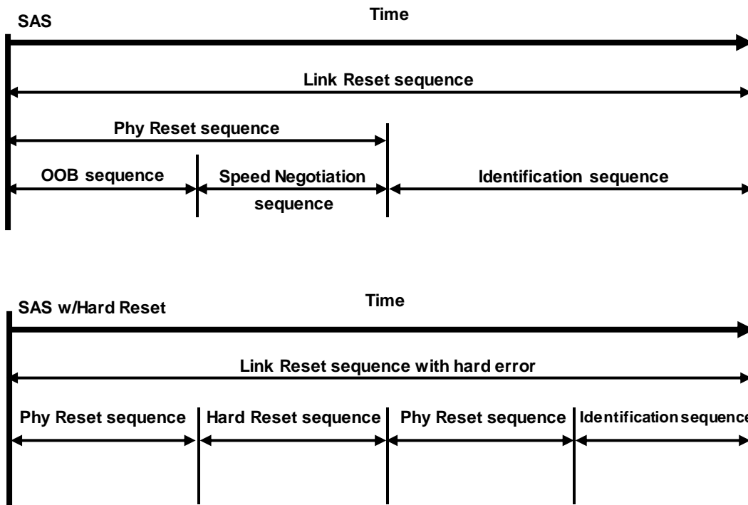
Figure 9 Link Reset Sequence
