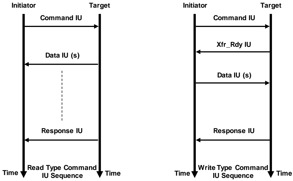
Figure 10 SSP Information Unit Sequences
