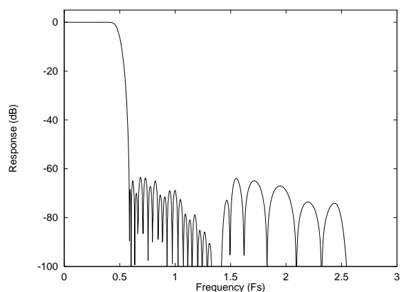
Figure 19 ADC Digital Filter Frequency Response – Type A
