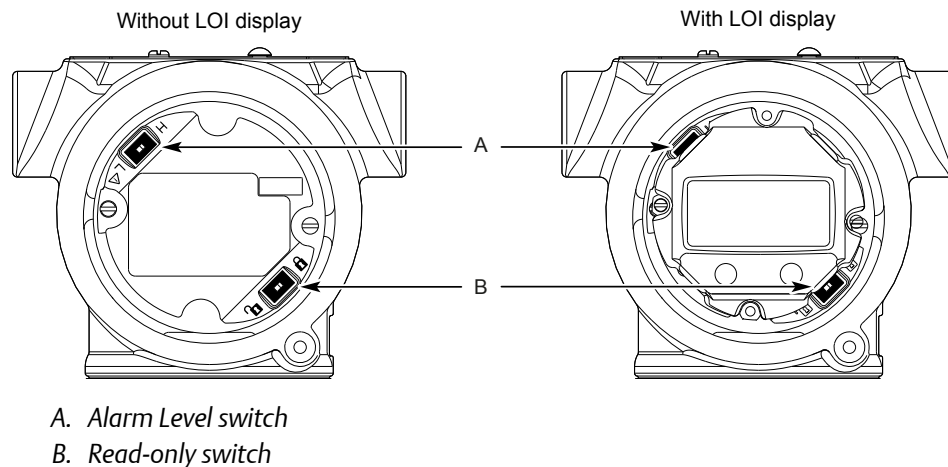
Figure 2-2: Alarm Level and Read-only Switches
