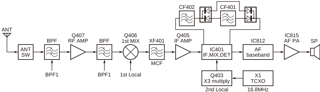
Fig. 2 Receiver system
