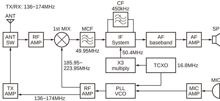
Fig. 1 Frequency configuration
