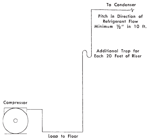
DISCHARGE LINE RISERS
