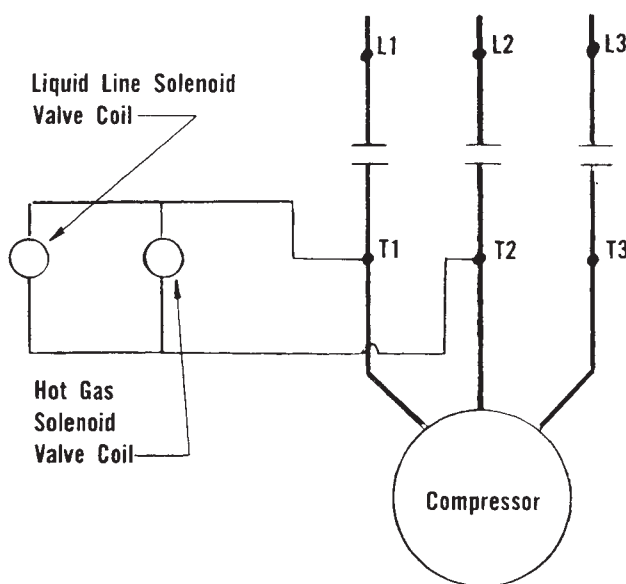
TYPICAL SCHEMATIC CONNECTION CONTINUOUS OPERATION - PILOT PROTECTION
