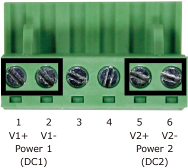
Figure 3-1: IGS-20160HPT Upper Panel
