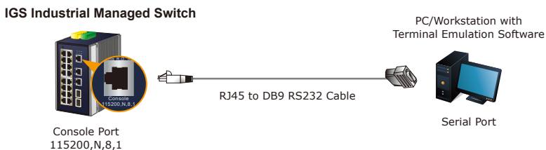
Figure 4-1: Industrial Managed PoE+ Switch Console Connectivity
